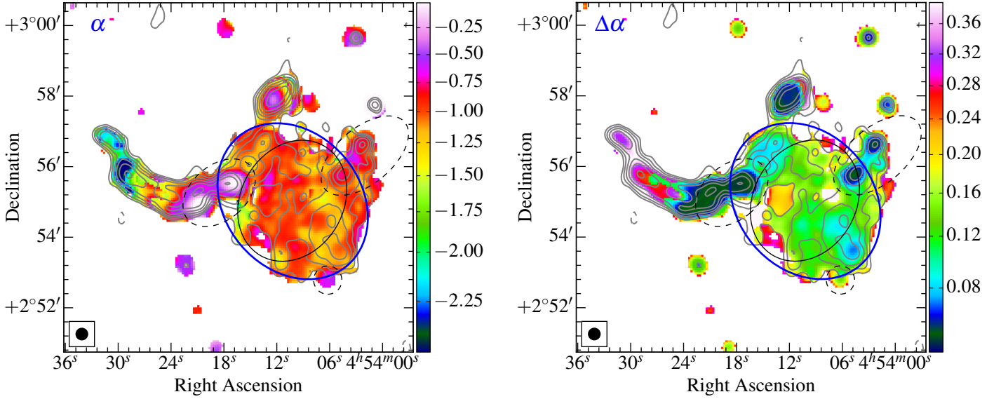
Fig. 3. Spectral index from 145 MHz to 1.5 GHz (left) and error (right) maps of A520. In the both panels, the blue thick ellipse roughly follows the 3\sigma contour of the halo emission. The black thin ellipse shows the inner region of the halo. The black dashed regions are masked. The LOFAR contours begin with 3\sigma , where \sigma = 450 \mu\text{Jy beam}^{-1} , and are spaced with \sqrt{2} .
