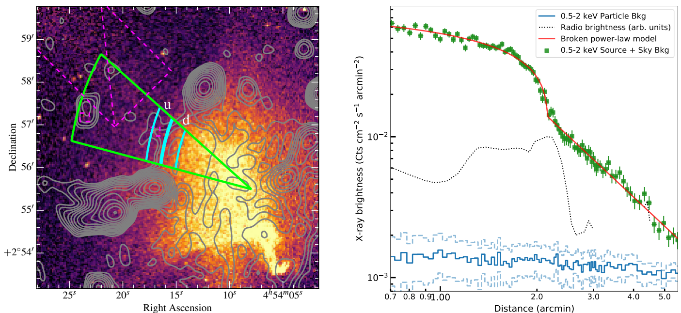
Fig. 7. Left: the sector where SB are extracted from the Chandra X-ray data. The magenta dashed regions are masked to remove the point sources and the emission from the NE plasma that is falling into the cluster. The blue regions represent where temperature is calculated for upstream and downstream ICM regions. Right: SB profile towards the NE region and the best-fit radial SB profile (red).
