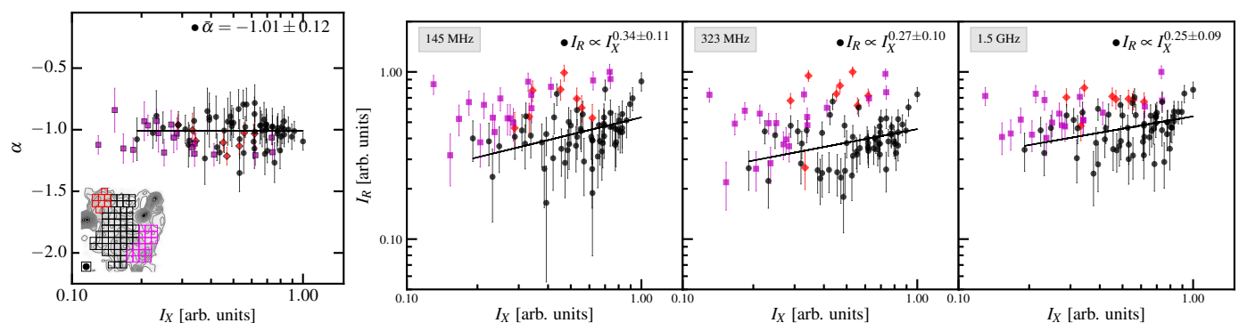
Fig. 8. Scatter plots of spectral index and radio SB ( I_R ) as a function of X-ray SB ( I_X ). The regions for extracting data are shown in the overlaid image (left). The data points are plotted in the same colour as the regions in the overlaid image (i.e. black circles for the central regions, magenta squares for the regions in the SW direction, and red diamonds for the regions in the NE direction). The best-fit parameters are obtained for the central regions.
