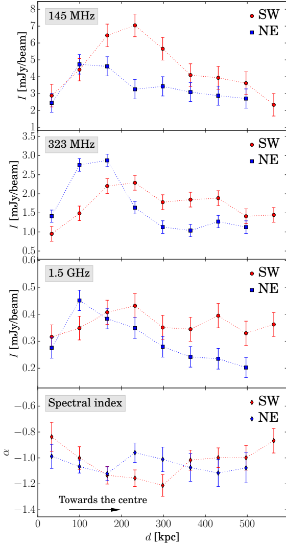
Fig. 6. Surface brightness (top panels) and spectral index (bottom panel) profiles from outer edges towards cluster centre for the regions in the SW and NE directions in Fig. 5. Towards the cluster centre, the spectral index is steepened for the SW radio emission and remains approximately constant for the NE radio emission.
