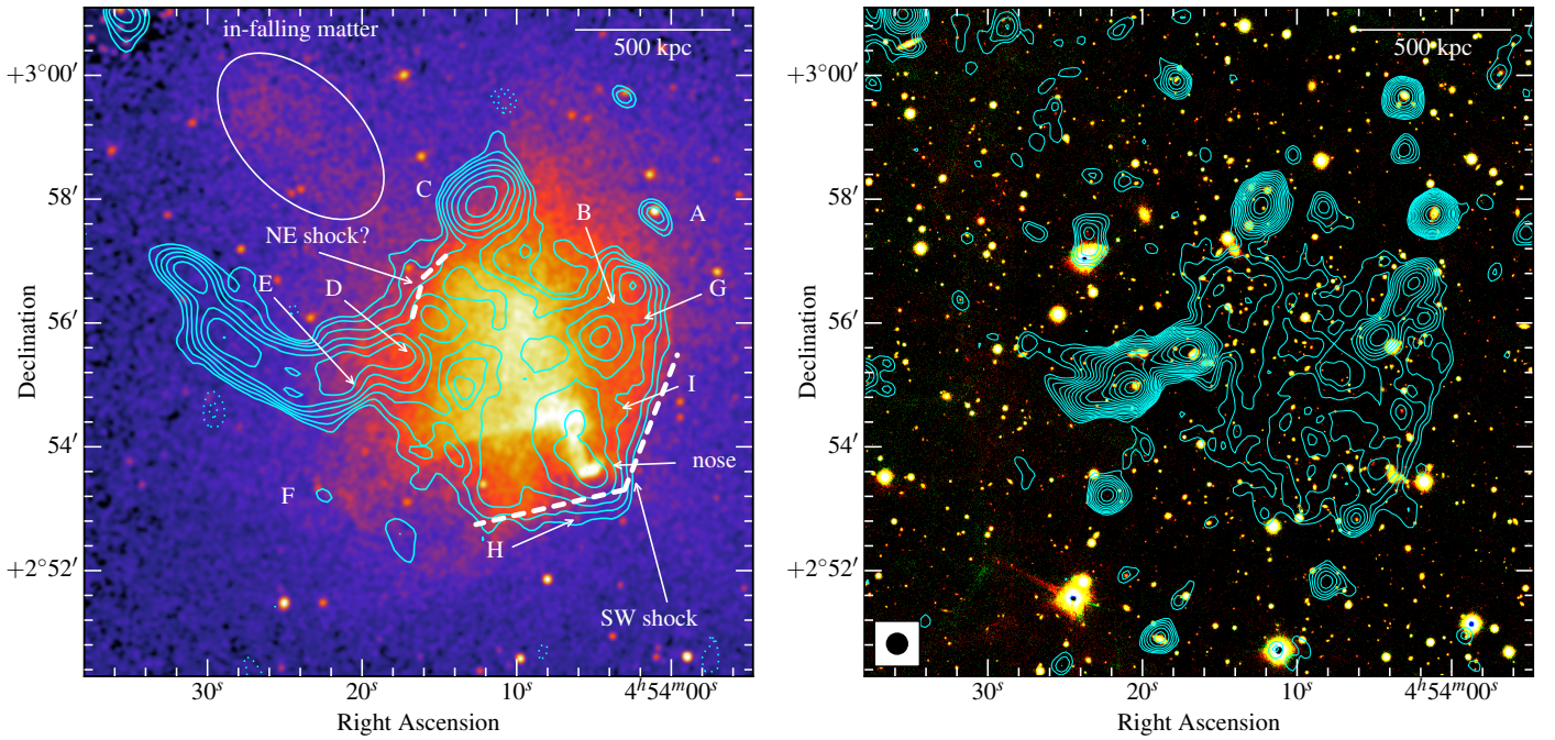
Fig. 2. Chandra 0.5 – 2.0 keV (left) and PanSTARRS colour (right) images of A520. The LOFAR (left) and GMRT (right) contours are identical to those in Fig. 1.
