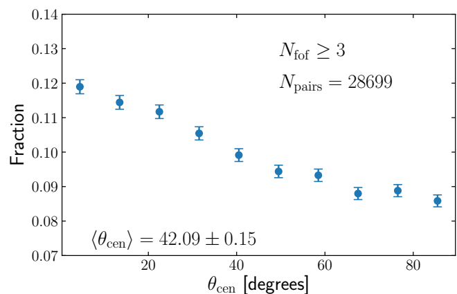
Fig. 10. Distribution of the angle \theta_{\text{cen}} between the BGG's semi-major axis and the line connecting the BGG-satellite pair. The mean value of the angle is shown in the bottom left of the plot.
