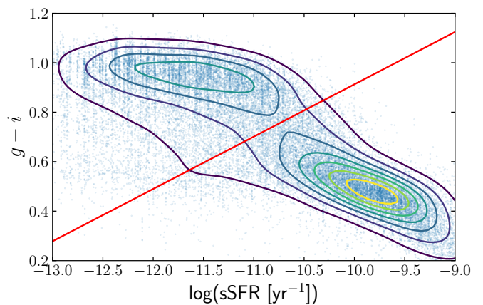
Fig. 7. Rest-frame, dust-corrected g - i colour of our satellite galaxy sample against their specific star formation rate. Smoothed density contours are shown, with dense regions appearing more yellow. The red line indicates the cut performed to divide our galaxy sample into blue star forming, and red galaxies with lower star formation rate.
