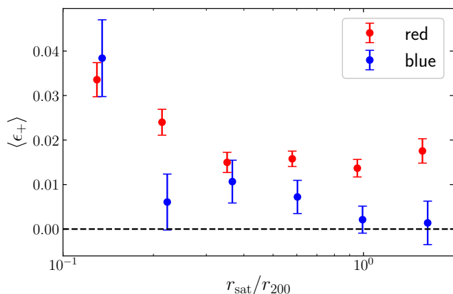
Fig. 12. Average tangential ellipticity of the BGG shape with respect to the satellites position, for red and blue BGGs. Results are obtained using r_{\text{wf}} = r_{\text{iso}} .
