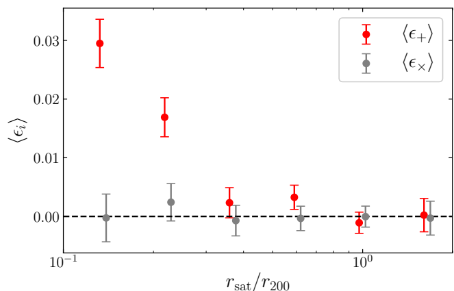
Fig. 3. Mean tangential/cross ellipticity (red/gray points) versus projected satellite distance from the group’s BGG, obtained using satellite shape - BGG position pairs. Positive values of \langle\epsilon_{+}\rangle indicate radial alignment while randomly oriented galaxies exhibit \langle\epsilon_{+}\rangle = 0 . Results shown for shape measurements obtained from r -band images, with r_{\text{wf}} = r_{\text{iso}} .
