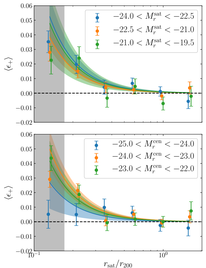
Fig. 5. Mean tangential/cross ellipticity components versus satellite distance from the BGG, obtained using satellite shape - BGG position pairs. Top: binned in satellite’s r -band absolute magnitude. Bottom: binned in BGG’s r -band absolute magnitude. Power-law fits with fixed index are over-plotted, with the 1\text{-}\sigma uncertainty on the fit, for the three bins. The grey area covers the radial bins over which we regard the BGG light correction to be too significant, and these scales are not used for our model fitting. Shapes were measured in r -band for r_{\text{wf}} = r_{\text{iso}} .
