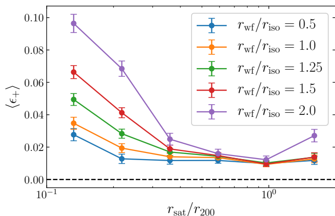
Fig. 11. Average tangential ellipticity of the BGG shape with respect to the satellites position, as a function of the projected distance of the satellite to the BGG. Results are obtained using 5 different weight function sizes, and are shown with a different colour.
