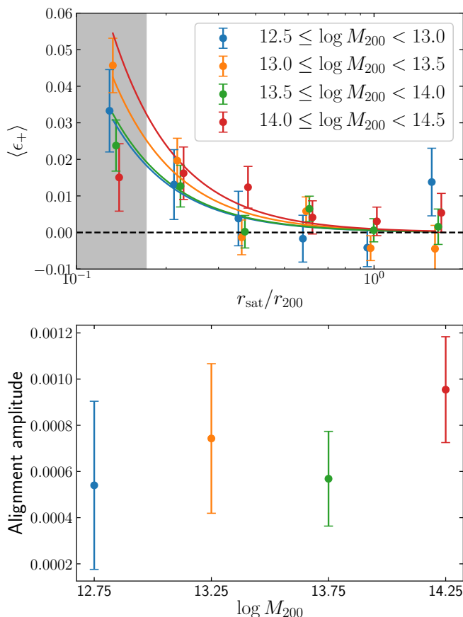
Fig. 6. Top: mean tangential/cross ellipticity as a function of satellite distance from the group’s BGG, obtained using satellite shape - BGG position pairs, binned in the group’s M_{200} . The best fit power-law with a fixed slope is overplotted for each mass bin. The grey area covers the radial bins over which we regard the BGG light correction to be too significant, and these scales are not used for our model fitting. Shapes were measured in r -band for r_{\text{wf}} = r_{\text{iso}} . Bottom: Amplitude of the power-law fit to the alignment signal for each individual group mass bin.
