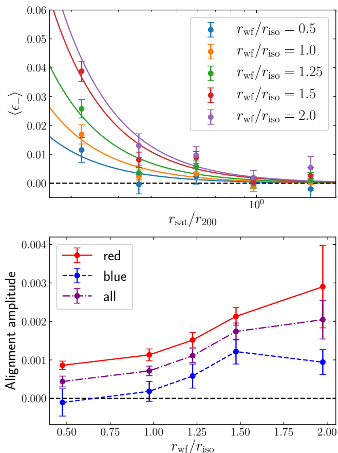
Fig. 9. Top: Average tangential ellipticity of the full satellite galaxy sample versus projected satellite distance from the group BGG, obtained using satellite shape - BGG position pairs. Results shown for different weight function sizes used in the shape measurement process. The r_{\text{wf}} indicates the size of the initial weight function and r_{\text{iso}} is the isophote of the galaxy. Bottom: Amplitude of power-law fits with fixed exponent, to the average ellipticities for all, red and blue galaxies, for the different weight function sizes involved. Lines connecting the data points added for clarity.
