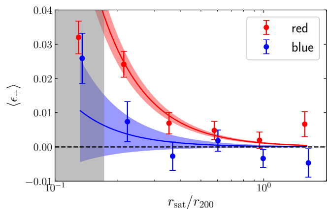
Fig. 8. Average tangential ellipticity against projected satellite distance from the group BGG, obtained using satellite shape - BGG position pairs. Results shown for red, low sSFR and blue, high sSFR galaxies. Power-law fits of fixed index are overplotted, with the shaded region indicating the 1-\sigma confidence limit. The grey area covers the radial bins over which we regard the BGG light correction to be too significant, and these scales are not used for our model fitting.
