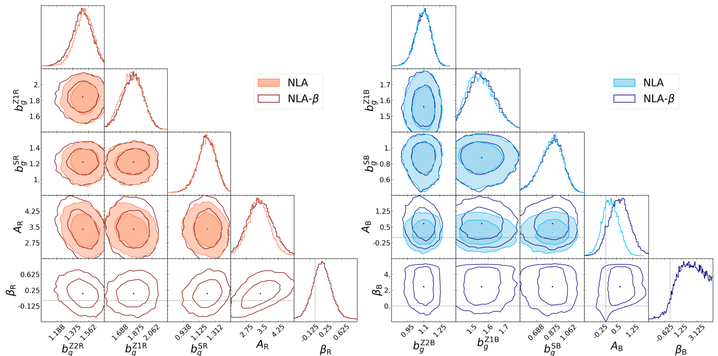
Fig. 5. Posterior probability contours of our fitted galaxy bias b_g , NLA amplitude A and luminosity power-law \beta parameters, for red (left) and blue (right) galaxies. The filled (unfilled) contours are for the NLA (NLA- \beta ) models. Dashed grey lines mark values of zero for IA parameters.
