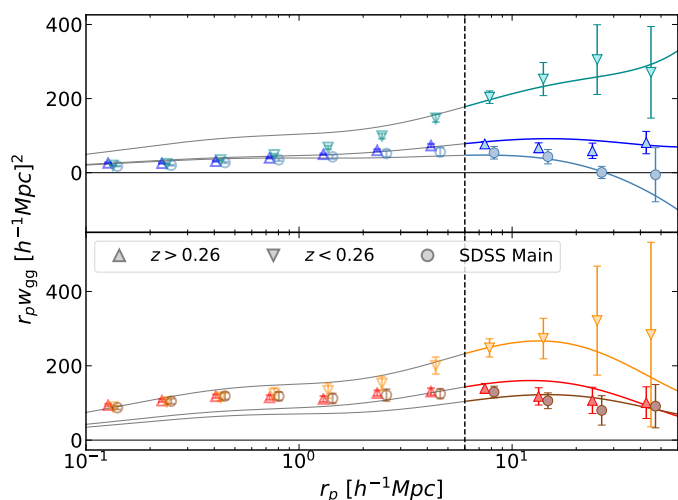
Fig. 2. Measured galaxy clustering for our blue ( top ) and red ( bottom ) galaxy samples. Solid curves illustrate the best-fit linear clustering per sample (Eq. 3.9). The vertical dashed line indicates r_p = 6 h^{-1} \text{Mpc} , below which scales are excluded from fitting (Section 3.3).
