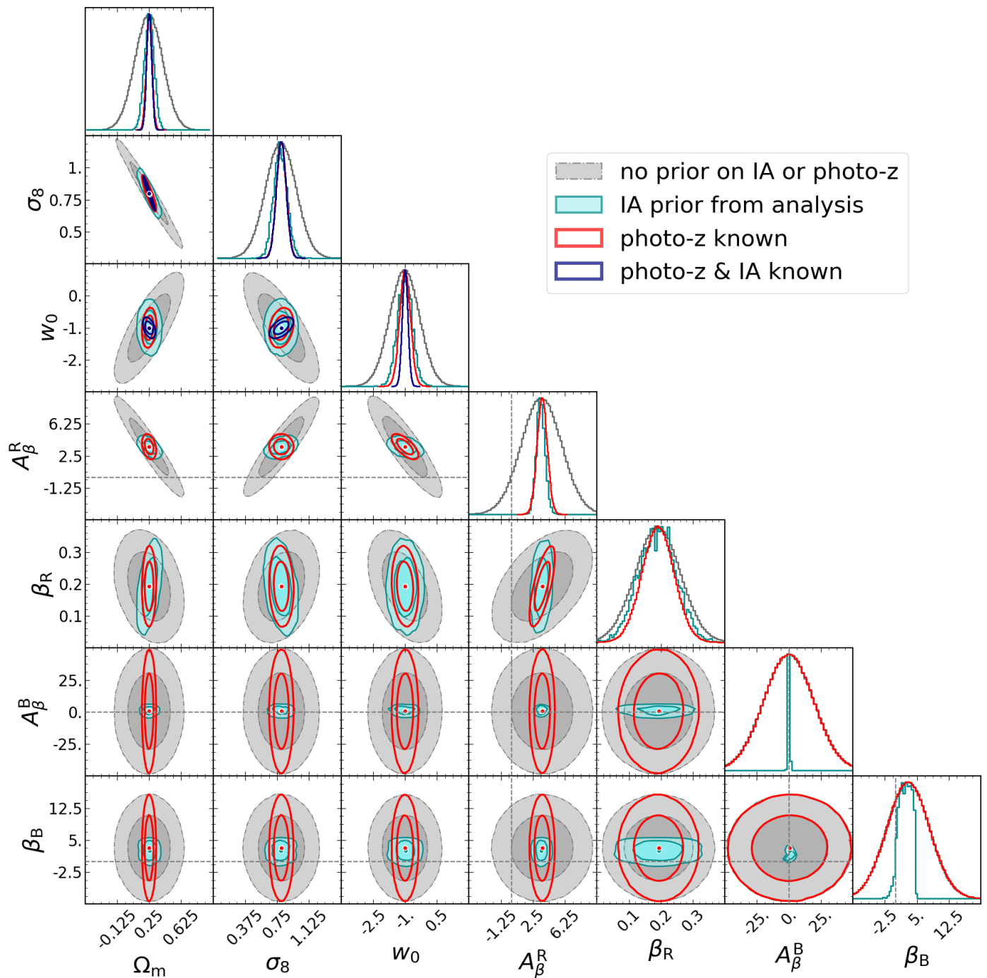
Fig. 9. The same as Figure 8, but assuming luminosity-dependent non-linear alignments (NLA- \beta ) in the data.
