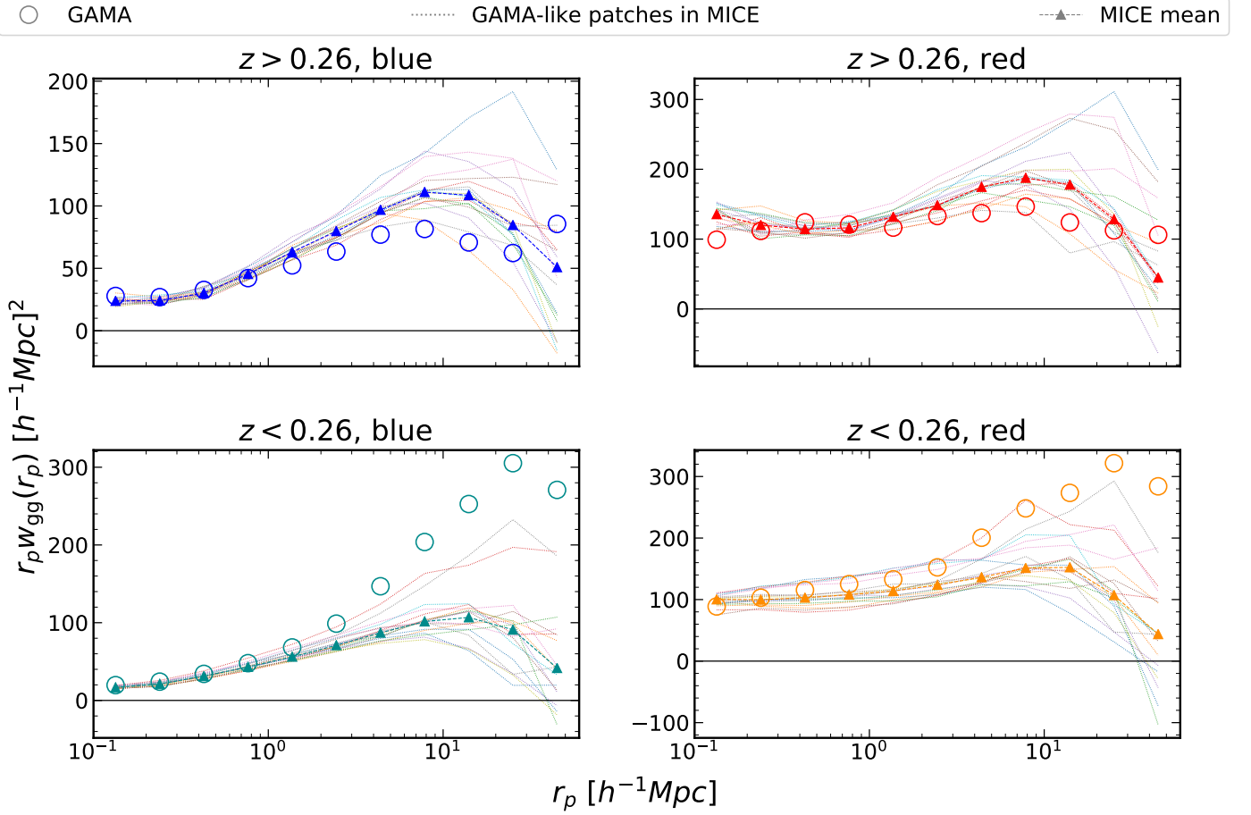
Fig. A.3. Clustering measurements from our defined GAMA galaxy samples (open circles) overlaid with corresponding measurements from individual, \sim 180 \text{ deg}^2 MICE subvolumes (dotted lines). Filled triangles show the means of the MICE clustering signals. We see significant differences between MICE and GAMA, particularly at low redshift and large scales, and so choose not to estimate covariances directly from MICE – see Appendix A.2 for details.
