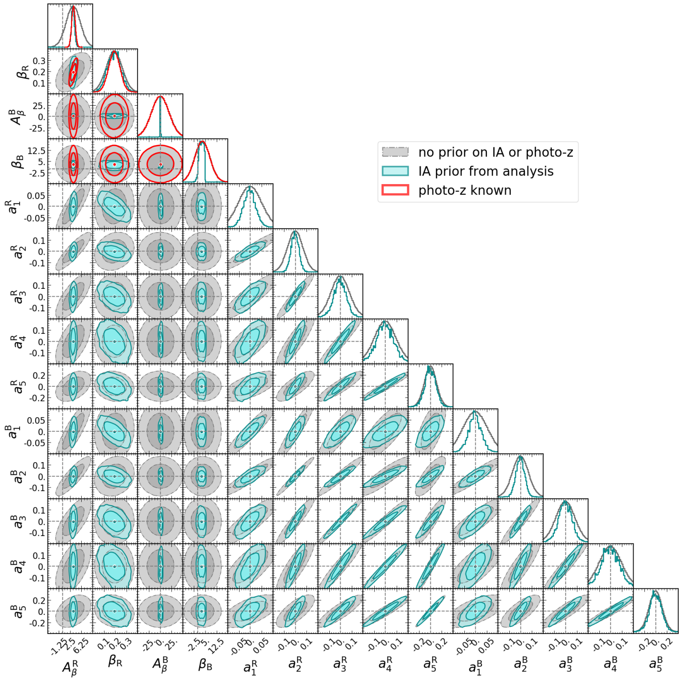
Fig. C.2. The same as Figure 9, for nuisance parameters only.
