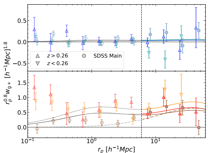
Fig. 3. Measured galaxy position-intrinsic shear correlations for our blue ( top ) and red ( bottom ) galaxy samples. Best-fit NLA models are shown as solid curves, and the vertical dashed line indicates r_p = 6 h^{-1} \text{Mpc} , below which scales are excluded from fitting (Section 3.3). The best-fit LA model to SR is shown as a dot-dashed line.
