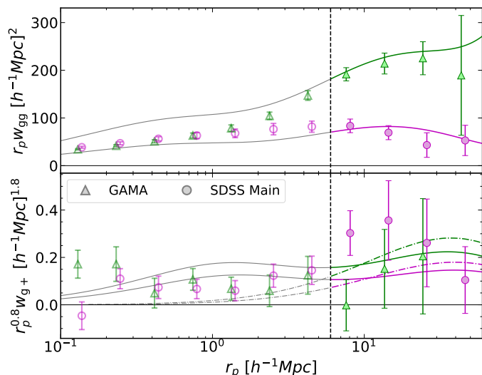
Fig. 4. Galaxy clustering ( top ) and position-intrinsic shear correlations ( bottom ) measured in the full KiDS+GAMA and SDSS Main datasets. Solid lines illustrate the best-fit NLA model, and dot-dashed lines the LA. The vertical dashed line indicates r_p = 6 h^{-1}\text{Mpc} , below which scales are excluded from fitting (Section 3.3).
