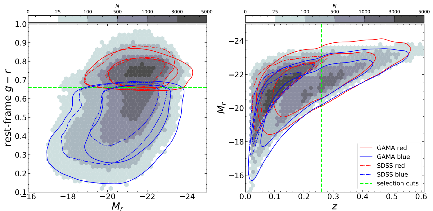
Fig. 1. Left: Galaxy rest-frame colour-magnitude diagram, where we choose a cut in g - r to isolate the red sequence in GAMA and SDSS. Right: Sample absolute r -band magnitude-redshift diagram. The total distribution of GAMA and SDSS galaxies is shown, binned in hexagonal cells with a colour scale corresponding to the counts in cells. Coloured contours indicate 75% and 95% of galaxies in a sample. Colour/redshift cuts are shown as dashed green lines, and the apparent leakage of contours is due to the grid-size used in kernel density estimation.
