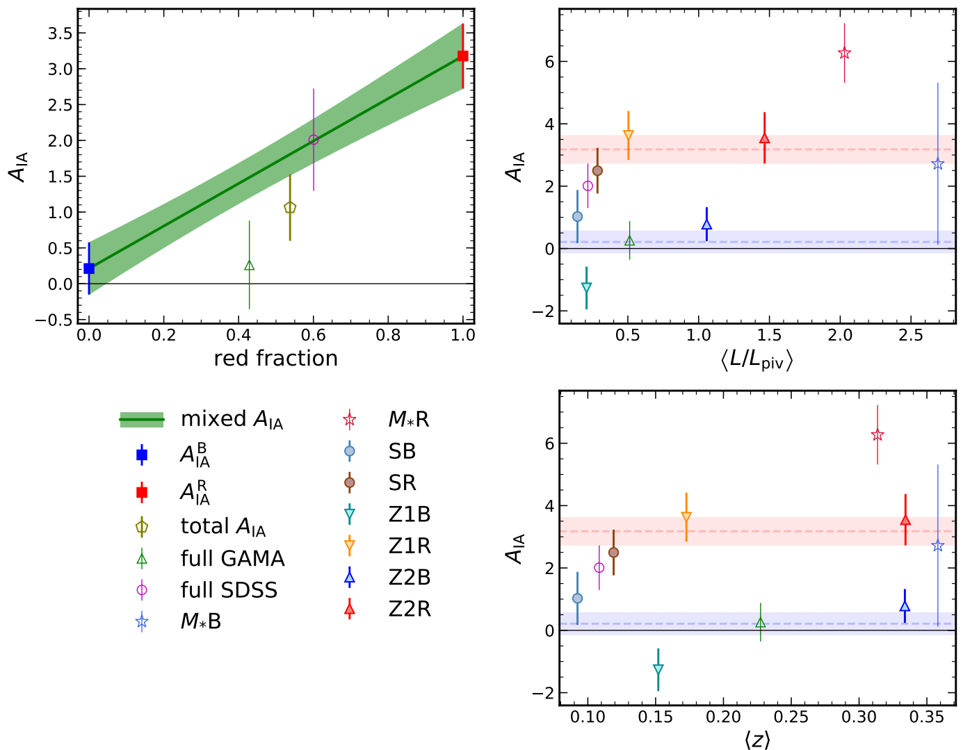
Fig. 6. Constraints on the NLA model alignment amplitude A_{\text{IA}} , from various subsamples of GAMA and SDSS (Table 1), plotted against sample properties. Top left: A_{\text{IA}} vs. shape sample red galaxy fraction. We interpolate (green line/shading) between our fits to blue (blue square) and red (red square) galaxy samples, according to A_{\text{IA}} = A_{\text{IA}}^{\text{R}} f_{\text{red}} + A_{\text{IA}}^{\text{B}} (1 - f_{\text{red}}) , where f_{\text{red}} is the red fraction and we assume linearity in the contributions of galaxy populations to the total alignment signal/amplitude. The inconsistency of mixed-sample signals (open points) with this interpolation is due to variable contributions of satellite galaxies – this is discussed in Section 4.2.2. Top right: A_{\text{IA}} vs. shape sample luminosity (as a ratio to the pivot L_{\text{piv}} \sim 4.6 \times 10^{10} L_{\odot} , corresponding to absolute r -band magnitude M_r = -22 ). Bottom right: A_{\text{IA}} vs. shape sample mean redshift. All plotted data points illustrate the mean and 68% confidence interval of 1D marginalised posterior distributions on A_{\text{IA}} , after fitting to relevant alignment/clustering signals. Only the filled points are independent of each other; each of the open points is in some way correlated with the others. Dashed lines and shading indicate the mean and 68% CI of the total-colour fits, highlighting the type-dependence of alignments.
