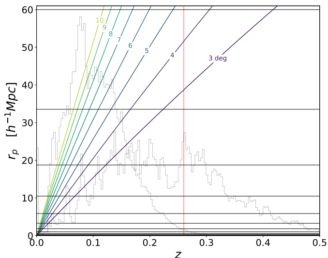
Fig. A.1. The comoving transverse distances corresponding to jackknife patches of given scales (in degrees), as functions of redshift. The r_p bin edges we employ are plotted as horizontal black lines, highlighting the limitations of too-small patches to sample larger r_p pairs, esp. at lower redshifts. The red vertical line indicates the z = 0.26 redshift division for the GAMA samples, and normalised redshift distributions for SDSS ( z \sim [0.02, 0.3] ) and GAMA ( z \sim [0.02, 0.5] ) are overlaid as dotted histograms.
