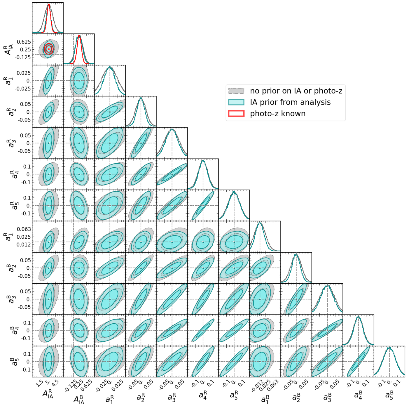
Fig. C.1. The same as Figure 8, for nuisance parameters only.
