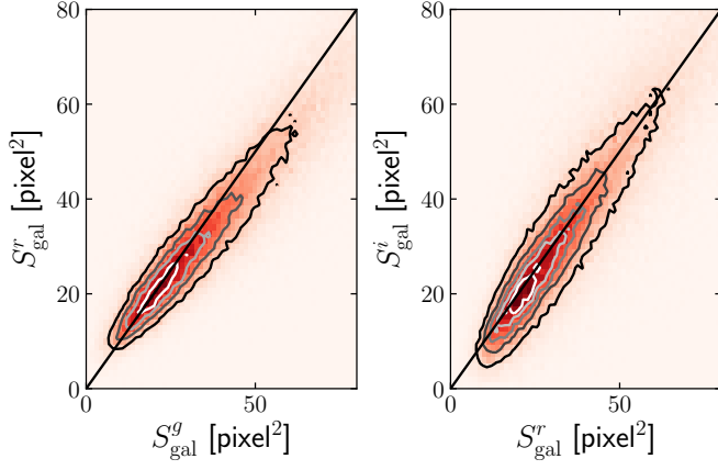
Fig. 6. Comparison of galaxy sizes, given from Eq. (12), between g and r -band sizes (left) and r and i band (right). The density map is shown, with denser regions appearing redder. Equally spaced contours are overlaid for clarity.
