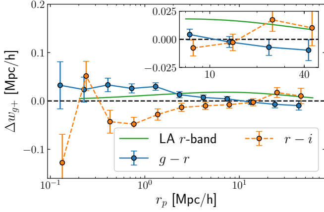
Fig. 7. Difference in projected density-shape correlation function between the g-r and r-i filters (blue and orange points respectively). The x-axis shows the transverse separation of galaxy pairs. For reference, the green line shows the LA model fit to the r -band data, described in Johnston et al. in prep. The in-line figure is a zoom-in on the last four data points, in the highest separations. Points are horizontally displaced for clarity.
