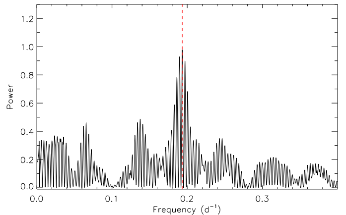
Fig. A.2: Generalised Lomb-Scargle periodogram of the combined FIES RVs. The red dashed line marks the orbital frequency of the brown dwarf. Note the presence of the 1-year aliases symmetrically distributed around the orbital frequency.
