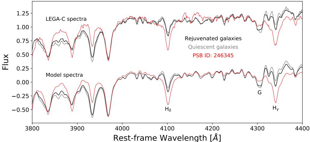
Figure 2. Average spectrum (LEGA-C as well as best-fit model) of rejuvenated galaxies (black) compared to the average spectrum of stellar mass and H\delta matched quiescent galaxies that do not show evidence of rejuvenation (gray). The PSB spectrum is shown for comparison. The spectra have been normalised and shifted for comparison purposes.
