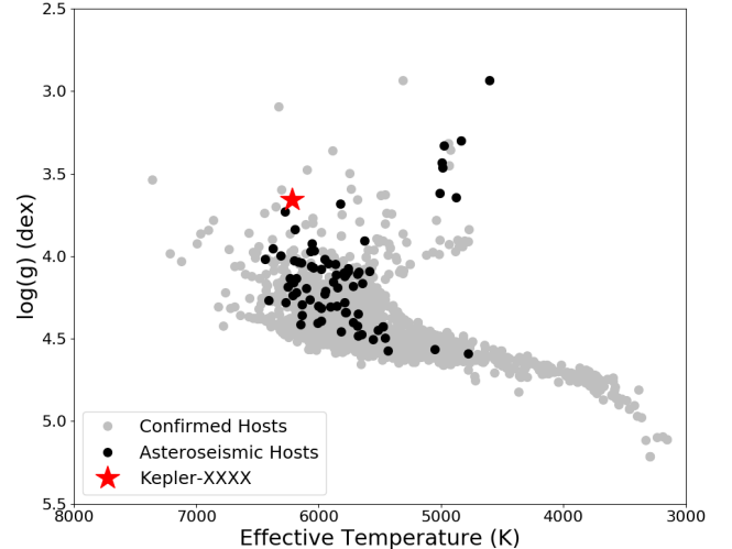
Figure 3. Surface gravity versus effective temperature for confirmed Kepler exoplanet hosts. Gray points represent confirmed hosts, with known asteroseismic hosts in black. Kepler-1658, represented by the red star, sits in an underpopulated area of stellar parameter space as a massive, evolved subgiant.
