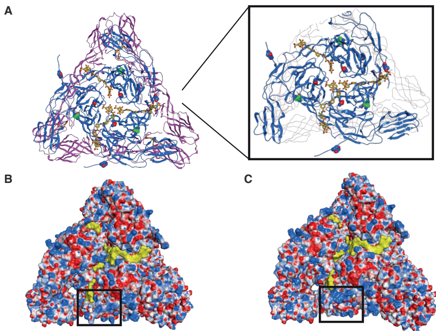
Figure 4. Molecular docking of suramin to a mature CHIKV spike. (A) The top view of a full wt E1-E2 heterotrimer (PDB ID 3J2W). The E2 proteins are represented as blue ribbon, the E1 as purple ribbon and the fusion loop as orange ribbon; the N5 and H18 residues are represented with carbon atoms in blue and green, respectively, and residue G82 with carbon atoms in red, belong to E2. Suramin is represented in yellow (3 molecules, carbon atoms and molecular surface). In the right black rectangle there is a clearer view of the spike core. (B) Electrostatic potential (Coulombic surface coloring) of the heterotrimer of wt CHIKV. The black rectangle marks the N-terminal domain of one E2 protein, where the positive charges are found. (C) Electrostatic potential (Coulombic surface coloring) of the heterotrimer of the N5R/H18Q mutant, CHIKV S9. The black rectangle highlights the N-terminal domain of E2 showing an increase in positive charges (blue molecular surface). For presentation purposes, the transmembrane and C-terminal segments of the E1 and E2, which interact with capsid proteins seen in (A), were removed.
