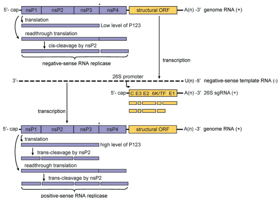
Figure 4. Schematic representation of the alphavirus genome, its translation products, polypeptide processing, and the types of RNA produced during replication/transcription. Upon genome translation the polypeptides nsP123 and nsP1234 are produced, the latter after read-through of the opal stop codon between nsP3 and nsP4. The cis-cleavage of nsP1234 produces the replicase complex (nsP123+nsP4) that synthesizes only the negative sense RNA (upper part of the figure). As the level of nsP123 increases, trans-cleavage occurs generating a short-lived nsP1+nsP23+nsP4 complex and the final nsP1+nsP2+nsP3+nsP4 complex, which is involved in synthesizing only positive sense RNA (g and sgRNA) – lower part of the figure. The structural proteins are translated from the sgRNA, also as two polypeptides due to a frameshift within the 6K protein-coding region: capsid-E3-E2-6K-E1 and capsid-E3-E2-TF. Capsid catalyzes its release from the polypeptide and the remaining polypeptide is processed by host proteases into individual proteins while trafficking along the secretory pathway. (Adapted from https://talk.ictvonline.org/ictv-reports/ictv_online_report/positive-sense-rna-viruses/w/togaviridae )
