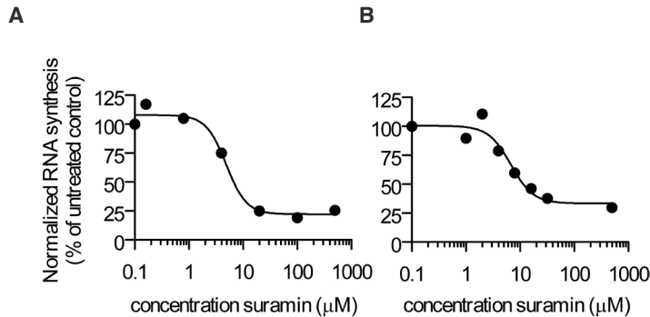
Figure S1. Quantification of the effect of suramin on alphavirus RNA synthesis in vitro . In vitro RNA synthesis assays were performed with RTCs, either isolated from CHIKV-infected Vero E6 cells (A) or from BHK-21 cells transfected with a CHIKV replicon (B), in the presence of increasing concentrations of suramin. RNA synthesis, i.e. the amount of incorporated 32 P-CTP, was quantified by determining the volume of the bands that are visible in Fig. 1A and Fig. 6A using the Quantity One® software. The values (sum of genome and subgenomic RNA) were normalized to the untreated control sample (100%) and were corrected for variations in RNA isolation efficiency and loading using 18S ribosomal RNA signal (detected by hybridization). The corrected normalized values (amount of RNA synthesized) obtained at each suramin concentration were plotted against the log of the suramin concentration and the IC 50 value was determined by non-linear regression using GraphPad Prism 5.
