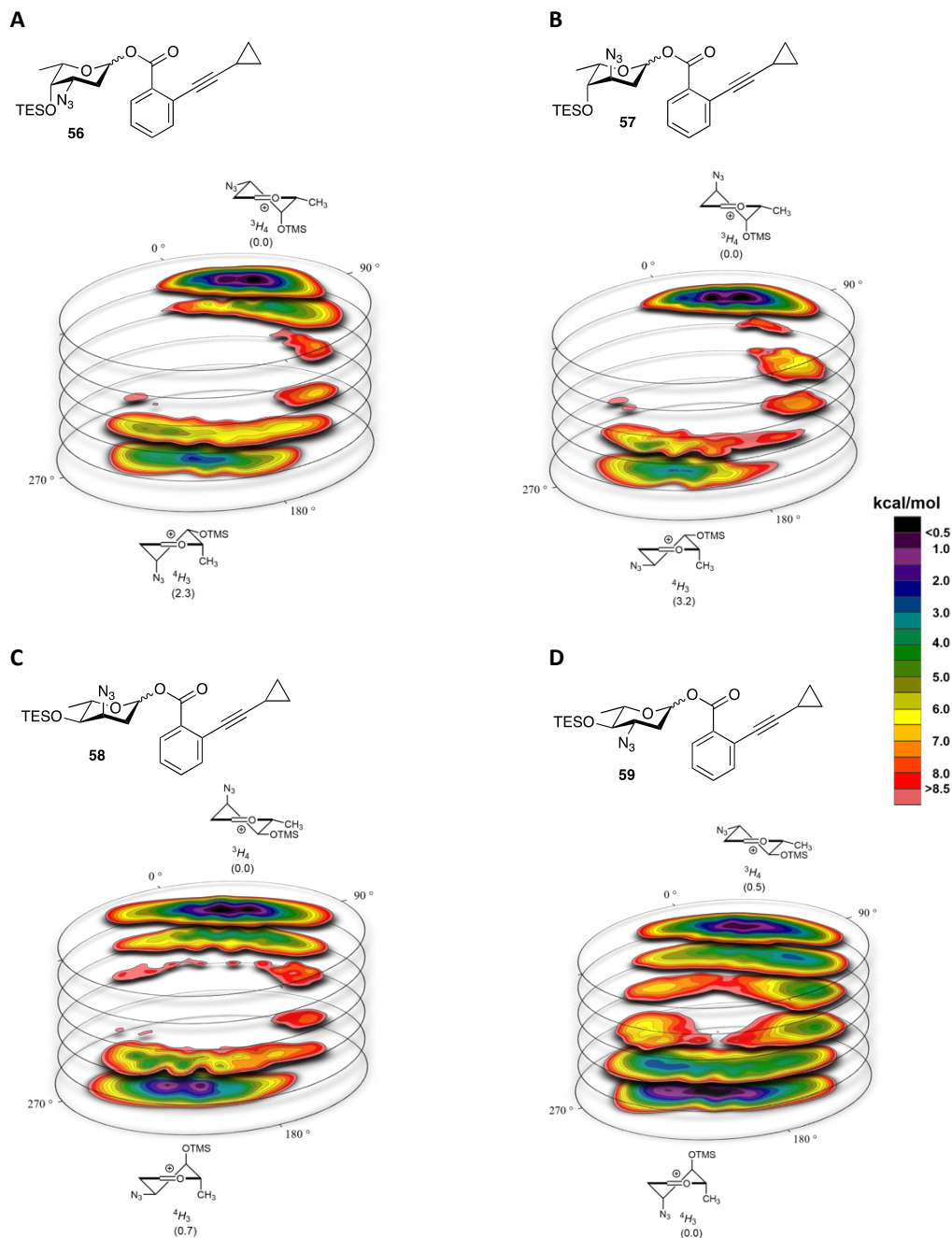
Figure 3. CEL maps of oxocarbenium ions in which the found local minima are indicated with their respective energies. (A) CEL map of daunosaminyl donor 56 derived oxocarbenium ions; (B) CEL map of 3- epi -daunosaminyl donor 57 derived oxocarbenium ions; (C) CEL map of ristosaminyl donor 58 derived oxocarbenium ions; (D) CEL map of acosaminyl donor 59 derived oxocarbenium ions.
