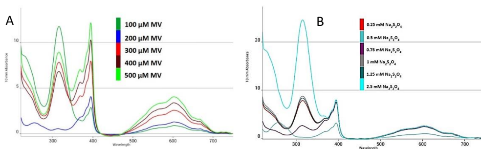
Figure 2.5 A: the UV spectra of MV with different concentration with 1.25 mM sodium dithionite in the solution. The ratio of A396 nm/A606 nm is about 3 which is same as the ratio in spectra of MV + . The peak at 606 nm is attributed to MV + , whereas the peak 396 nm can be from MV + and MV 0 . That means the sodium dithionite only converts MV to MV + . If there is MV 0 , the MV 0 will contribute to the UV absorption at 396 nm. In this case, the ratio A396 nm/A606 nm should be larger than 3. This reaction was also reported in the literature. 45 B: the UV spectra of 300 \mu M MV with different amounts of sodium dithionite. Adding more excess sodium dithionite does not improve the conversion rate. The MV can be saturated at about 60% conversion rate.
