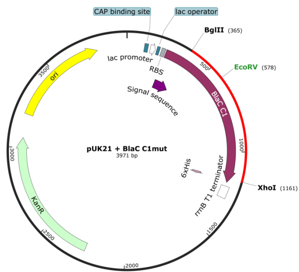
Figure S4.8. Map of the cloning/expresson plasmid used for generation of the mutant library. The section of DNA that was mutated through error-prone PCR is displayed in red.
