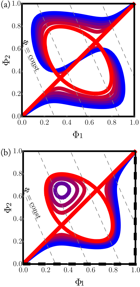
Figure 4.9: Lines of equilibrium. Solutions of Equation 4.49 for two spheres with radii ratio R_2/R_1 = 2/3 at sub-critical temperature T = 0.45 qJ . (a) Lines have all T_L^{(a)} = 0 but regularly increasing T_c^{(a)} from 1/2 qJ (red) to (1/2 + 1/10 R_a^{-2}) qJ (blue). (b) Lines have all \Delta T_c = 0 while T_L^{(a)} increases from 0 (red) to 1/20 R_a^{-2} qJ (blue). The black, thick, dashed line corresponds to the infinite T_L^{(a)} limit. Diagonal dashed lines are of constant \Phi .
