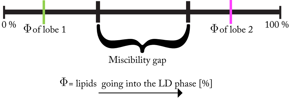
Figure 3.6: Schematic definition of antimixing. In the antimixed configurations, the percentages of lipids going into the LD phase of the single lobes \{\Phi_1, \Phi_2\} are located on antipodes, i.e. opposite sides, of the local miscibility gap. The notation \{\Phi_1, \Phi_2\} will also be used in Section 3.5. We stress that it is different from \{\varphi_1, \varphi_2\} which indicate the percentages of area occupied by the LD phase in the two lobes.
