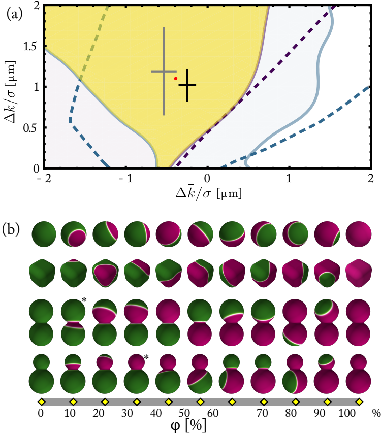
Figure 3.8: Elastic moduli differences and interface models. (a) In the two-dimensional parameter space spanned by (\Delta k/\sigma, \Delta \bar{k}/\sigma) , the yellow region shows the parameter values for which the minimal-energy configurations match with the experimental observations for the two CSLBs highlighted by the white asterisks in Figure 3.5. The solid lines correspond to the boundaries of allowed parameters for the symmetric (blue) and asymmetric dumbbell-shaped (violet) configurations obtained via minimisation of the diffuse interface model, Equation 3.4. The dashed lines show the analogous result obtained from minimising the sharp interface model Equation 3.3 under the further assumption of an axis-symmetric interface. For further comparison, we show measurements of these parameters obtained previously using GUVs. The points with error bars are from Baumgart et al. 65 (grey) and Semrau et al. 66 (black), and their average is shown by a red dot. (b) Theoretical diagrams of the percentage of area for the four geometries used in the experiments obtained by minimising the diffuse interface energy Equation 3.4 (green and magenta colours correspond to LO and LD phases, and white to the interfacial region). The asterisks depict the two configurations that match the ones highlighted in Figure 3.5. These models cannot reproduce the observed gaps. In the Appendix “Details on the numerical simulations of Chapter 3”, we report details on the numerical simulations to obtain this figure.
