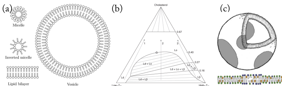
Figure 1.2: Model lipid bilayers. (a) Overview of self-assembled structures of lipids, including a vesicle and a planar lipid bilayer. (b) Schematic ternary phase diagram of a mixture of high melting temperature lipids, low melting temperature lipids, and cholesterol. L \beta , Ld, and Lo are the solid, liquid disordered, and ordered phases, respectively 13 . (c) Top: illustration of a phase-separated lipid vesicle. Bottom: phase-separated lipid bilayer composed of cholesterol (yellow), low (green) and high (blue) melting temperature lipids. 14 Images reprinted with permission of Cold Spring Harbor laboratory press (b) and Elsevier (c).
