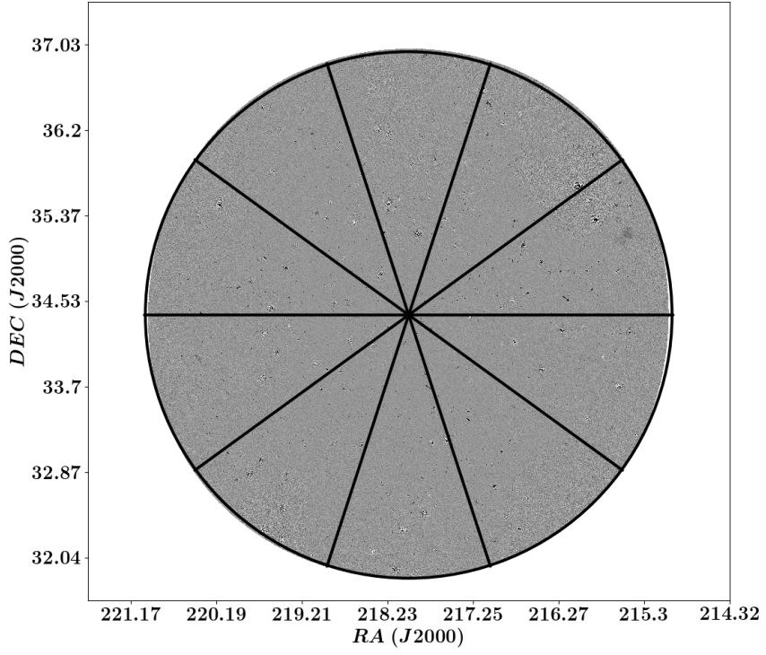
Figure 3.15: The spatial distribution of the circular sectors in the Boötes mosaic used to test the effect of cosmic variance in our source counts. Each circular sector has an approximate area of 2 \text{ deg}^2 .
