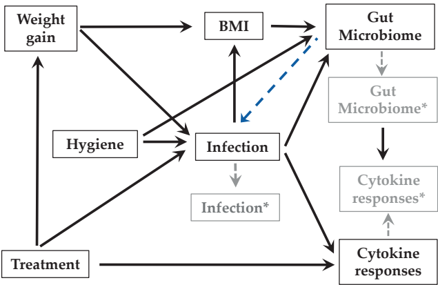
Figure 6.2: The DAG representing the relationship of all variables when measurement errors were included. The grey variables represent the observed variables with errors and blue line represents the possible causal direction.
