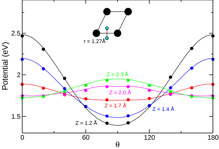
Figure 4.5: The \theta -dependence of the H_2 + \text{Ag}(111) SRP48 PES is shown for molecular configurations centered on a bridge site ( X = 1/2a ; Y = 0 ), \phi = 90^\circ and r_b = 1.27 \text{ \AA} , where a is the surface lattice constant. Full lines: interpolated PES; symbols: DFT results. The values of Z corresponding to different curves and sets of symbols are provided with matching color.
