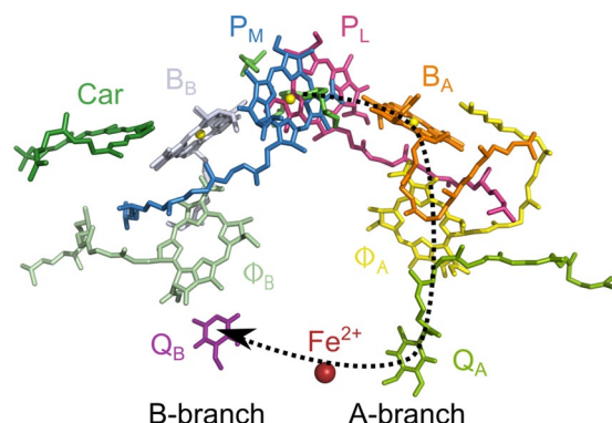
Figure 1. Cofactor arrangement in the RC of R. sphaeroides WT: P_M and P_L — bacteriochlorophyll a dimer, forming the primary electron donor, the Special Pair P, B_{A/B} — accessory bacteriochlorophyll a , \Phi_{A/B} — bacteriopheophytin a , Q_{A/B} — quinone A and terminal electron accepting quinone B, Fe^{2+} — non-heme iron, Car — carotenoid. The electron is transferred only via the A-branch (black arrow). For details, see text.
