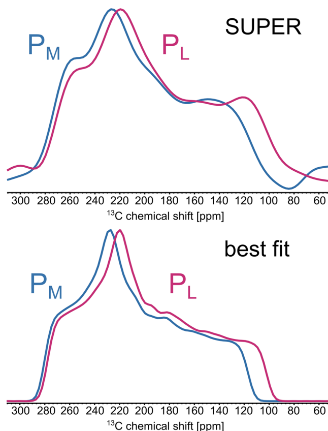
Figure 6. Cross section from the experimental 2D SUPER spectra (top) and the best fit (bottom) patterns of the C-3 1 -carbon in the acetyl groups of P M and P L . The principal values of the best fit are summarized in Tab. 2 in the “Experiment P L ” and “Experiment P M ” column.
