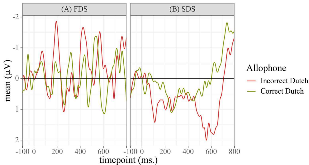
FIGURE 8 | Grand-average waveforms calculated over the [ε~ε:] condition only, averaged over all participants, electrodes, and the three sessions. A difference in amplitude can be observed between the two allophone conditions, in the SDS group only, which reaches permutation-based significance in the 560–660 ms window.
