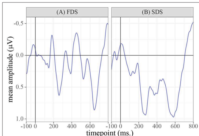
FIGURE 6 | Grand-average waveforms calculated over the full dataset, averaged over the three sessions and the two allophone conditions. A difference in amplitude can be observed between the FDS and the controls, which reaches permutation-based significance in the 390–470 ms window.
