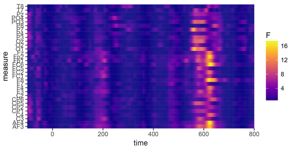
FIGURE 7 | Permutation tests performed on the data for the [ɛ~ɛ:] contrast, showing the effect of the factor “Allophone×Group.” A significant difference can be observed, which reaches permutation-based significance between 560 and 660 ms.
