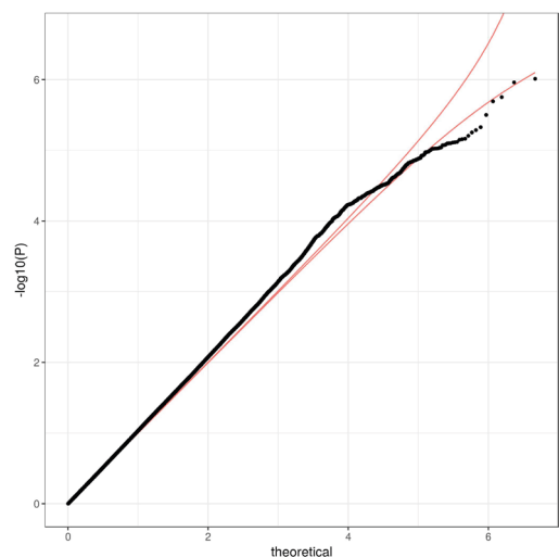
Figure 3. QQ-plot of p-values The Quantile-Quantile (QQ)-plot shows the extent to which the observed distribution of the test statistic follows the theoretical null distribution. The inflation factor was \lambda=1.04 .
