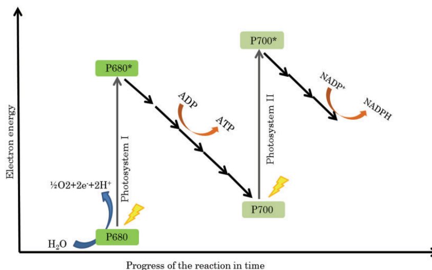
Figure 1.2 Representation of the linear electron flow in the light reactions process according to Hohmann-Marriot et al. [1].
