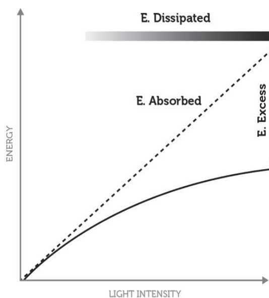
Figure 1.3 The graphic illustration, according to Ruban et al. , shows how in high light condition is necessary the photoprotection of the photosystem II. The 'excess energy' is defined as the difference between the light absorbed and the utilized, which can cause photo-oxidative damage to the photosynthetic system. This excess will be dissipated via NPQ processes as heat [10].
