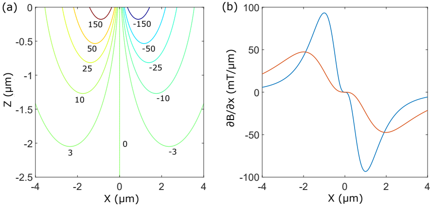
Figure 8.4: (a) Contourplot of \partial B/\partial x in the Y = 0 plane for a magnet with radius 0.95 \mu\text{m} . The labels indicate the magnitude of \partial B/\partial x in units \text{mT}/\mu\text{m} . The surface of the magnet is located at Z = 0 . (b) Cross-section of Fig. (a) for two different magnets, one with radius 0.95 \mu\text{m} (blue) and the other with radius 1.9 \mu\text{m} (red), along Z = R_0/3 (following Garner). As predicted, the magnitude of \partial B/\partial x scales with the inverse of the radius of the magnet, while the distance between the center of the magnet and the optimum of \partial B/\partial x scales linearly with the radius.
