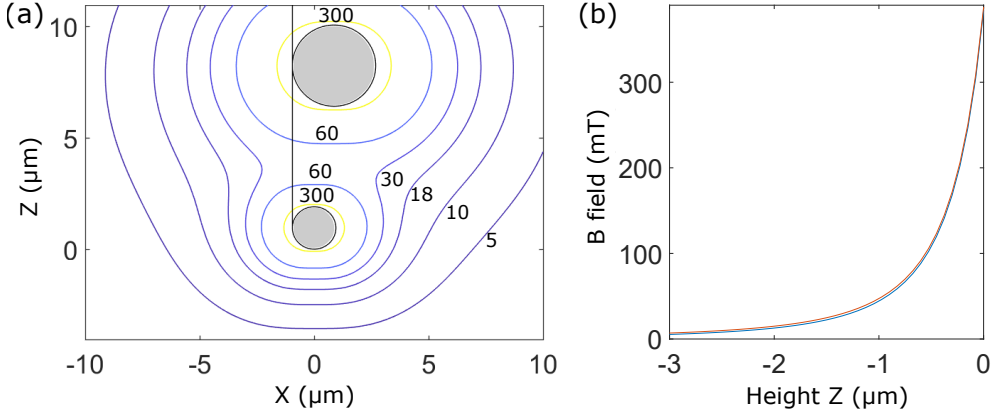
Figure 8.3: (a) Contour plot of the magnetic field distribution around the new cantilever (radii 0.95 \mu\text{m} and 1.82 \mu\text{m} ). The gray circles indicate the positions of the magnets. The labels indicate the magnitude of the field (mT) for the different contour lines. (b) B-field versus the distance between the sample and the surface of the magnet for a single magnet (blue) and the double magnet (red) configurations, calculated directly below the magnet.
