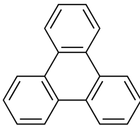
FIGURE 4.1: Molecular structure of triphenylene ( C_{18}H_{12} ). The peripheral hydrogen atoms are omitted for clarity.
