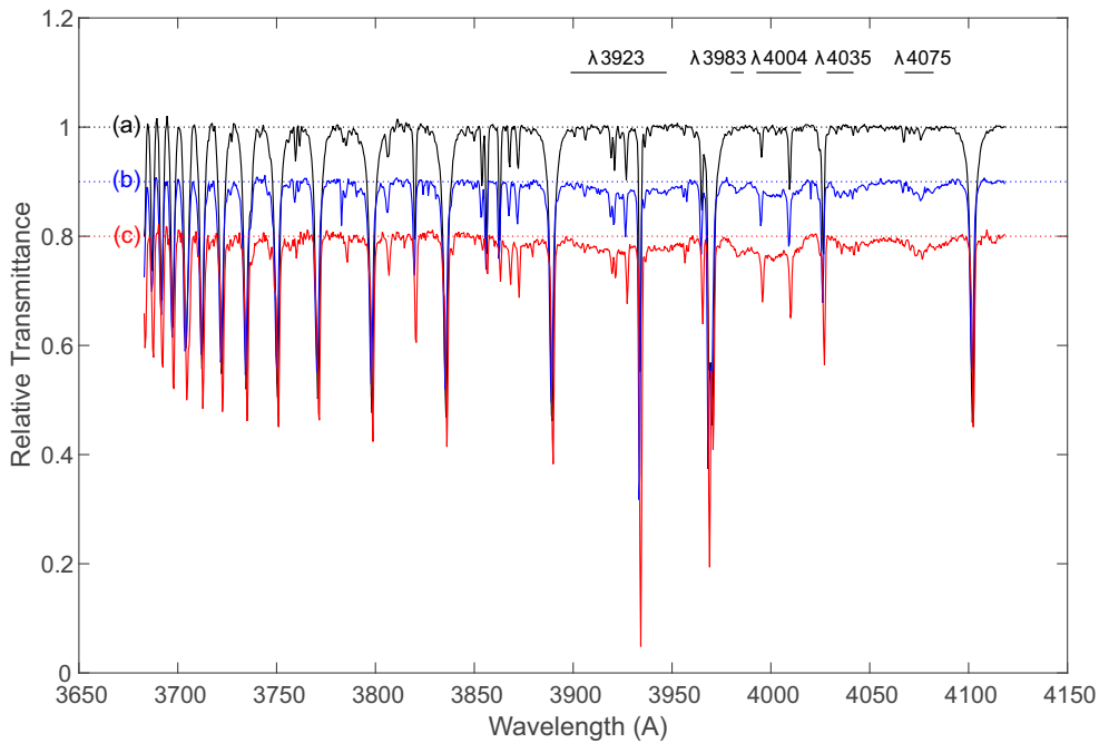
FIGURE 4.4: Spectra recorded towards the unreddened standard star \beta Ori (HD 34085) (a), and two reddened stars HD 183143 (b) and HD 50064 (c), with the latter two spectra each offset vertically by 0.1. Stellar hydrogen and interstellar Ca II H and K (3968.5 and 3933.7 Å) lines are prominent, with broad diffuse bands seen towards the two reddened stars between 3850 and 4100 Å (see also table 4.2 and the text). The location of the diffuse bands is marked with horizontal bars.
