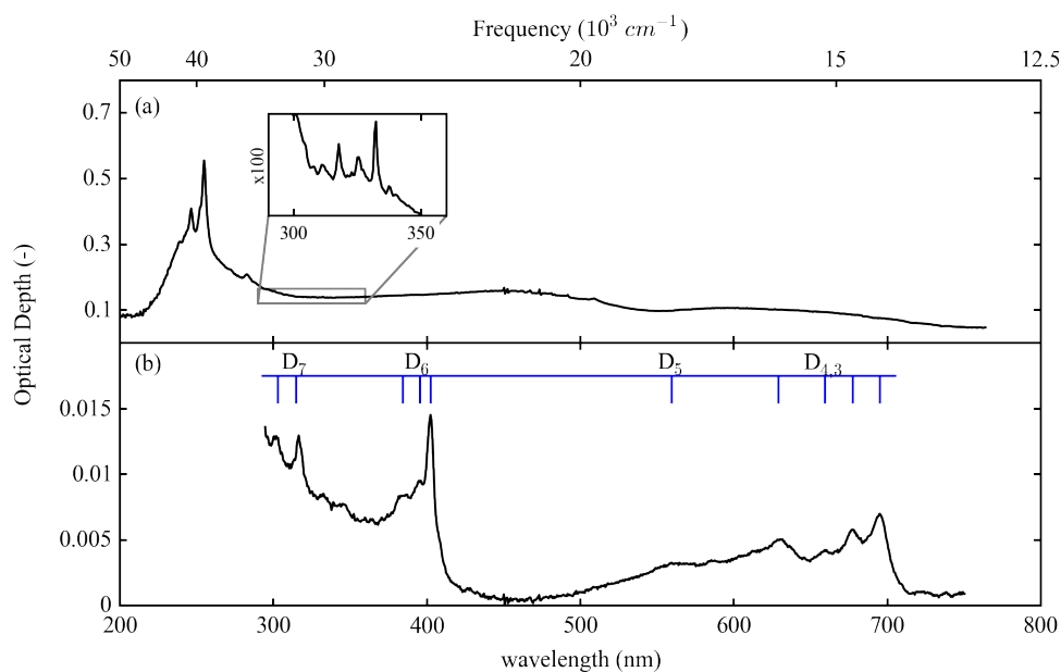
FIGURE 4.2: Electronic spectra of triphenylene neutral (a) and cation (b) in an argon matrix at 12 K. The inset in (a) shows the forbidden transitions to the S_1 state, which are approximately two orders of magnitude weaker and significantly narrower than the allowed transitions. In (b) the labeling D_3 , D_4 , D_5 etc. indicates the electronically excited doublet (D) state of the cation involved in the transition and follows the notation given in Keszthelyi et al., 2000.
