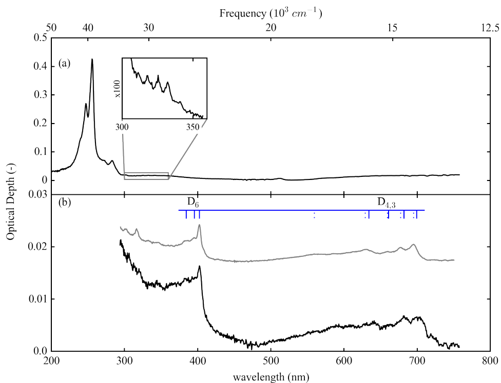
FIGURE 4.3: Triphenylene neutral and cation deposited in a water matrix at 12 K where (a) shows the neutral spectrum and (b) the cation (see 4.5.2). Dotted lines in the cation assignments indicate the location of the transitions in the argon matrix, full lines indicate the position in the water. For clarity, the spectrum of the cation in argon as presented in figure 4.2 is shown below the cation spectrum in water ice.
