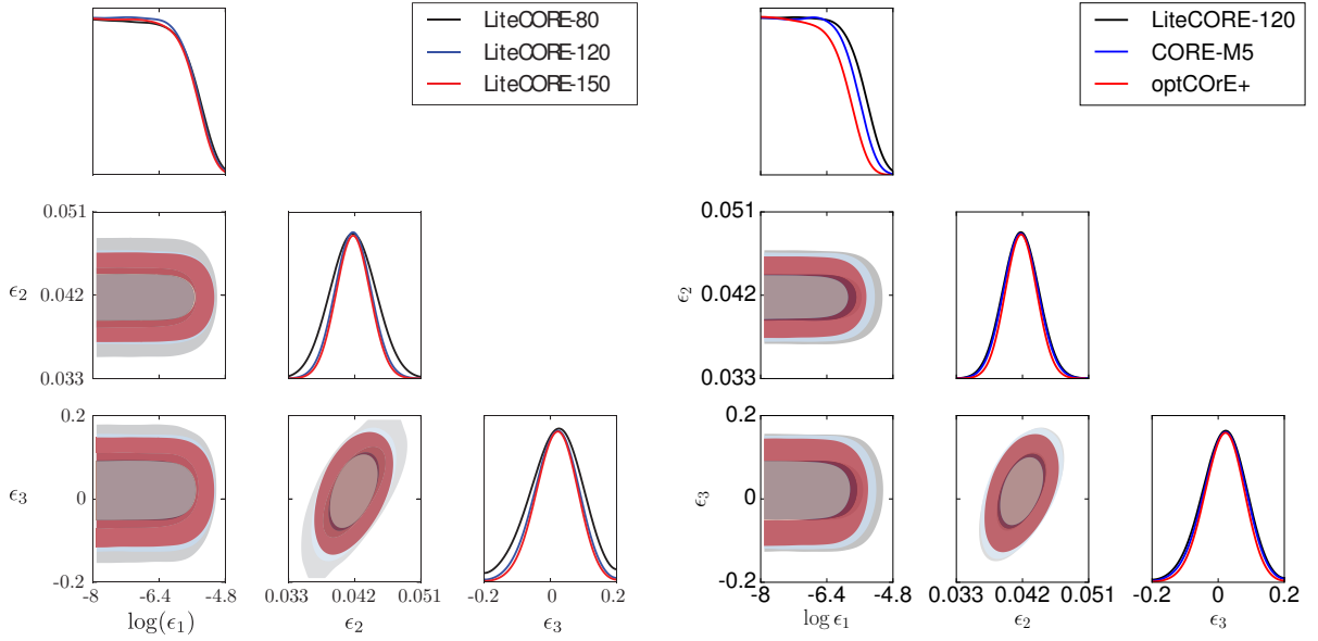
Figure 14: Compared forecasts on the Hubble flow parameters (1D and 2D marginalized posterior distributions after CMBxMCMC delensing) when the fiducial model is MHI.
