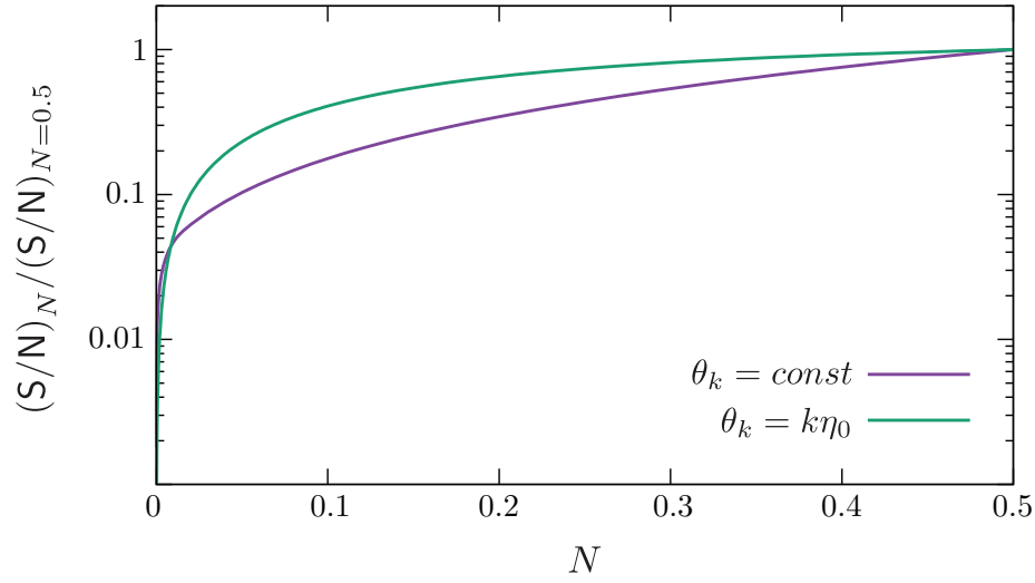
Figure 36: Dependence of the signal-to-noise ratio on the value of the occupation number N . Signal-to-noise ratio for different N is here normalized to the values obtained for N = 0.5 as displayed in Fig. 35.
