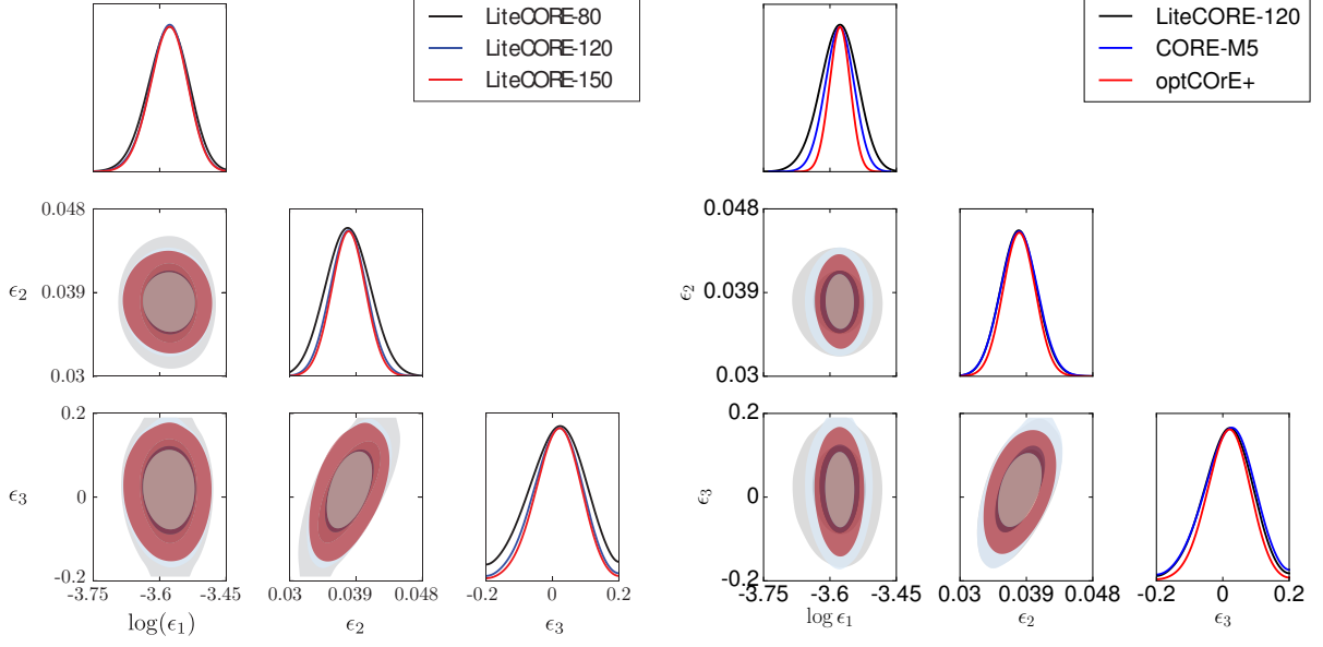
Figure 13: Compared forecasts on the Hubble flow parameters (1D and 2D marginalized posterior distributions after CMBxMCMC delensing) when the fiducial model is SI.
