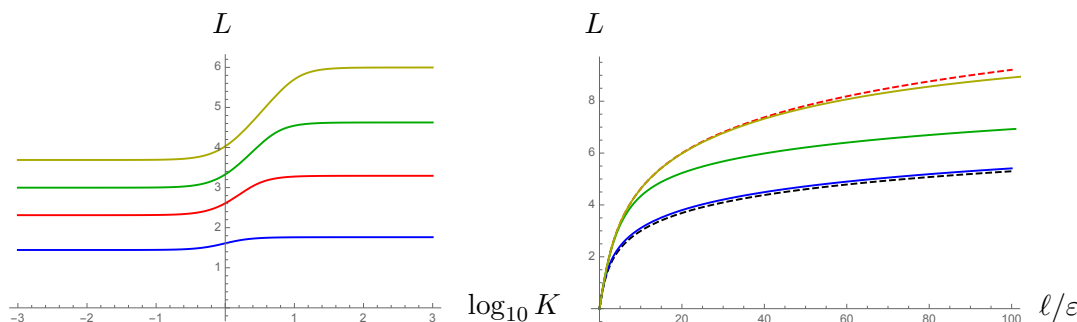
Figure 4. Entanglement entropy for a flow between a CFT in the IR and z = 2 Lifshitz theory in the UV. Left: length as a function of \log_{10} K for \ell/\varepsilon = 2, 5, 10, 20 (bottom to top). These curves interpolate monotonically between the correct IR (left) and UV (right) limits. Right: length as a function of \ell/\varepsilon for K = 0.5, 5, 50 (bottom to top, solid). The dashed lines correspond to the IR (black) and UV (red) limits.
