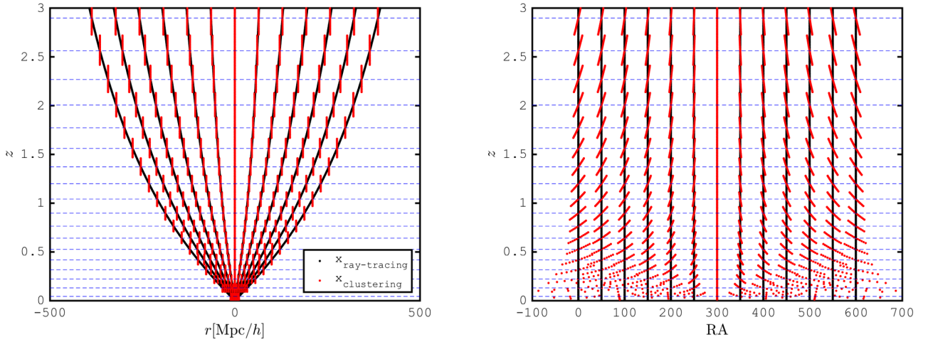
Figure C1. Illustration of the two coordinate systems needed by the mock data. Left: the data points in each red ‘stick’ represent example of objects that share the same \theta_{\text{ray-tracing}} coordinates, even though their \theta_{\text{clustering}} coordinates differ. In the multiple lens technique, the photon trajectories descend along red sticks that are connected by a common black line. They are then assigned to pixels with coordinate \theta_{\text{ray-tracing}} , traced by the black lines. In the far-field limit, the red and black align. Right: the \theta_{\text{clustering}} coordinate of the same red points, as seen from lines of constant \theta_{\text{ray-tracing}} . In this frame, the \theta_{\text{clustering}} coordinates extend outside the 10 \times 10 \text{ deg}^2 patch.
