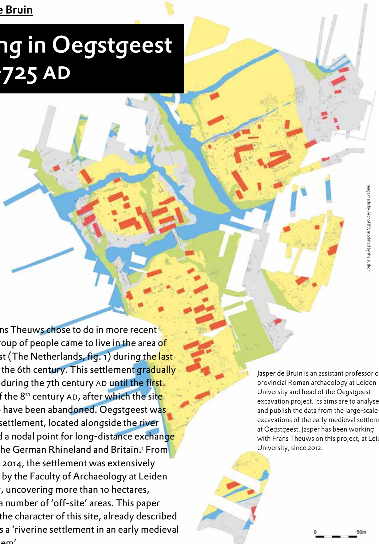
Fig. 2 General overview of the Oegstgeest settlement, including the most recent excavations from 2017-2018. Blue is water, green are low lying clay areas, grey are low levees, composed of silty clay, yellow are higher, sandy levees and lastly red are buildings.
