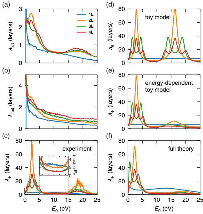
FIG. 3. (a) Energy-dependent total MFP \lambda_{tot} for electrons impinging on 1–4 layer graphene obtained from the spectra in Fig. 2 using Eq. (1). It decreases with energy, but is generally much lower than the universal curve predicts. (b) The inelastic MFP \lambda_{inel} [Eq. (2)] shows a similar trend but the layer-dependent maxima are absent. (c) The elastic MFP \lambda_{el} [Eq. (3)] exhibits strong, layer-dependent peaks at the energies of high-transmission states where \lambda_{el} is very long. The enlarged inset shows that the \lambda_{el} is largest for monolayer graphene in the energy range from 6 to 12 eV. (d) An optical toy model based on transfer matrices describes position and shape of the layer dependent oscillations in the \lambda_{el} well. (e) When an energy-dependent absorption is taken into account, the experimental data in (c) is well described by this simple model over the full energy range. (f) The \lambda_{el} calculated from the ab initio spectra in Figs. 2(c), 2(d) also reproduces the experiment well over the full energy range.
