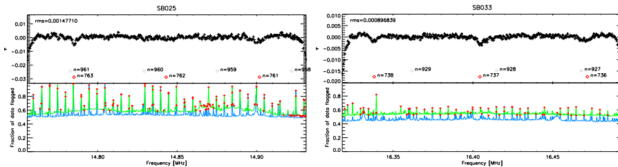
Figure 2.2.: Spectra of two individual subbands, 25 and 33. The top panels show the optical depth \tau as function of frequency. The red diamonds show the location of \text{Ca} lines, while the empty labels those of \text{C}\beta . The bottom panels show the percentage of data flagged for the L69891 and L69893 datasets in blue and green respectively. Red diamonds mark channels which were removed because their flagging percentage is larger than 5% that of the subband mean.
