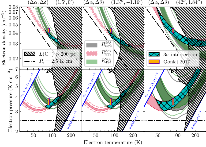
Figure 3.8.: Constraints imposed by the R_{539}^{268} = \text{C}268\alpha/\text{C}539\alpha , R_{539}^{357} = \text{C}357\alpha/\text{C}539\alpha and R_{494}^{268} = \text{C}268\alpha/\text{C}494\alpha line ratios in the n_e - T_e plane (top panels) and in the P_e - T_e plane (bottom panels). The constraints are shown for the -47 \text{ km s}^{-1} velocity component at three different positions in the map. The positions, relative to the map centre, are shown on the top of the corresponding column. These positions are shown in Figures 3.7 and 3.9 as green crosses. The orange rectangle with purple borders shows the gas physical conditions derived by Oonk et al. (2017). The dot-dashed line shows a curve of constant electronic pressure. The cyan region hatched with black lines shows the intersection of the constraints imposed by the R_{539}^{268} , R_{539}^{357} and R_{494}^{268} line ratios if we consider their 3\sigma ranges. The densely hatched region shows where the required ionized carbon path length is larger than 200 pc. Blue lines in the bottom row show the limits of the grid of CRRL models.
