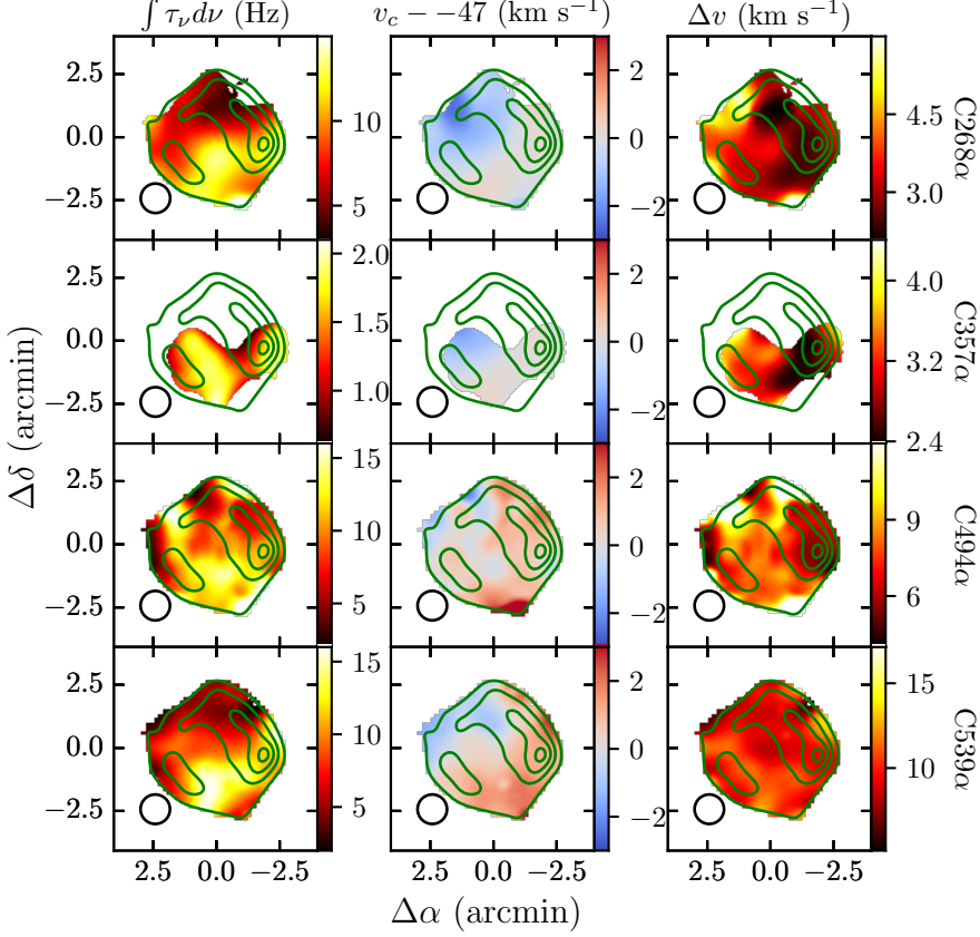
Figure 3.5.: Moment maps for the CRRs at -47 \text{ km s}^{-1} . The top row shows the moment maps for the C268 \alpha line, the upper middle row for the C357 \alpha line, the lower middle row for the C494 \alpha line and the bottom row for the C539 \alpha line. The left column shows the integrated optical depth, the middle column the velocity centroid of the line with respect to -47 \text{ km s}^{-1} and the right column the full width at half maximum of the line. The green contours show the 345 MHz continuum from Cas A at 51'' \times 45'' resolution. The 70'' resolution of the moment maps is shown in the bottom left corner of each map. At the edges of Cas A the signal-to-noise ratios are lower due to the fainter continuum.
