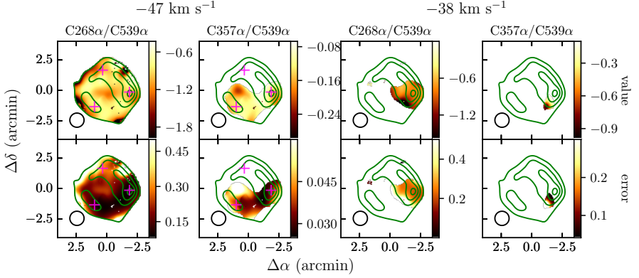
Figure 3.7.: Ratios between different CRRLs at different velocities. The ratios shown are the R_{539}^{268} = \text{C268}\alpha/\text{C539}\alpha and R_{539}^{357} = \text{C357}\alpha/\text{C539}\alpha line ratios. The top panels show the ratio value and the bottom panels the error on the ratio. The text on top of each column indicates which ratio is shown in the corresponding column, and a text label on the top of the Figure shows the velocity component. The ratios show only regions where both lines involved have been detected with a signal-to-noise ratio larger than three. The pink crosses in the top panel show the regions used in Figure 3.8. The 70'' resolution of these maps is shown in the bottom left corner of each map.
