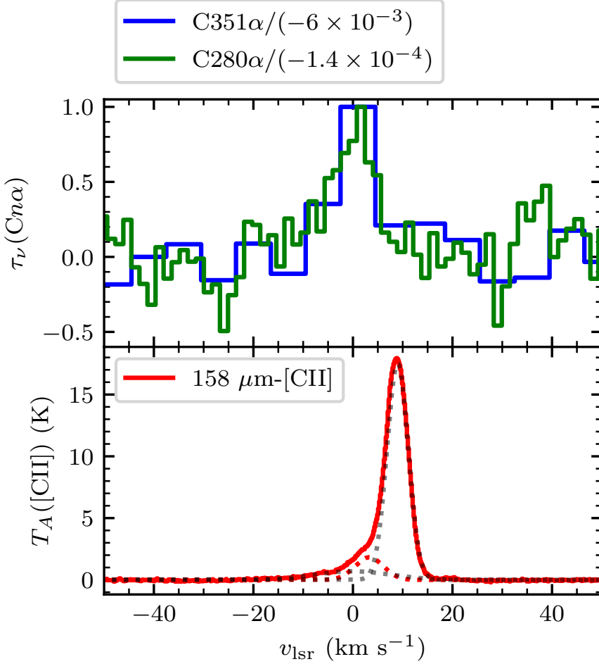
Figure 4.6.: Comparison between the CRRLs observed in absorption and the 158\ \mu\text{m} -[CII] line. The blue steps show the C351 \alpha line profile inverted (from the LOFAR observations in 2014), the green steps the C280 \alpha line inverted (from the GBT observations AGBT02A_028) and the red steps show the 158\ \mu\text{m} -[CII] line (from the SOFIA observations of Pabst et al. 2019). The CRRLs trace a fainter velocity component in the 158\ \mu\text{m} -[CII] line due to the effect of stimulated emission. The dotted lines in the lower panel show the best fit Gaussian line profiles used to decompose the 158\ \mu\text{m} -[CII] line (the properties of these component are given in Table 4.3). The spectra are the spatial average over a circle 36'' in diameter centered on M42.
