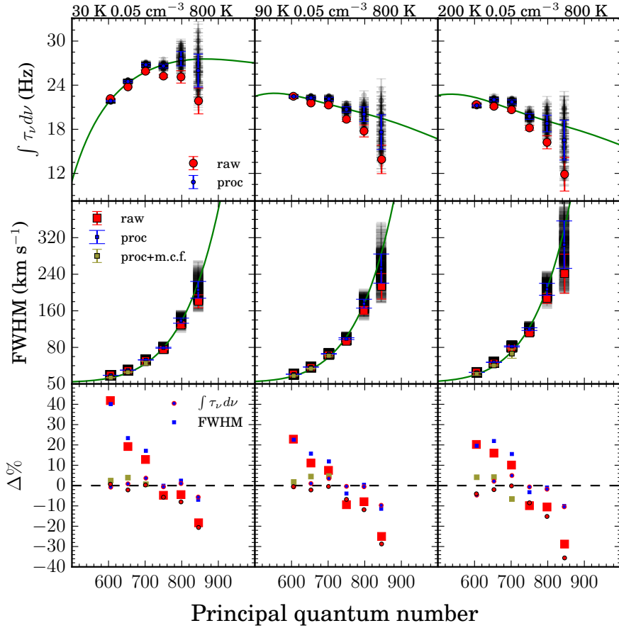
Figure 2.10.: Comparison between the input line properties and the measured line properties of synthetic spectra. The top row shows the integrated optical depth as a function of principal quantum number. The grey points show the results of individual simulations after continuum subtraction, stacking and baseline removal, the blue points show the mean of the grey points and the red points show the mean of the stacks with no baseline removal. The input line property is shown with a green line . The middle row shows the line FWHM. The symbols have the same meaning as in the top row, but the points are now squares . The yellow squares show the line width of the dominant component when multiple velocity components are fitted (m.c.f.) to the line profiles. The bottom panel shows the difference between the input value and the measured one. The comparison with processed data is shown by the blue symbols , while for the unprocessed data we use red symbols . The yellow squares show the difference between the input model for the dominant component and the measured line width for the dominant component after processing.
