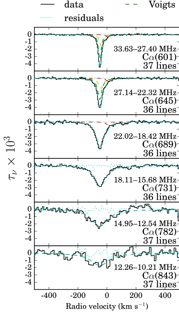
Figure 2.3.: Stacked \text{Ca} spectra. The black steps show the stacked spectra after processing, the green, yellow and red dashed lines show the best fitting Voigt profiles for the different components, the cyan dashed line shows the combined best fit Voigt profile and the cyan dotted line shows the residuals. The spectra are shown in optical depth units.
