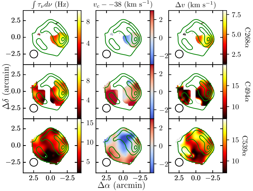
Figure 3.6.: Moment maps for the CRRLs at -38 \text{ km s}^{-1} . The top row shows the moment maps for the C268 \alpha line, the middle row for the C494 \alpha line and the bottom row for the C539 \alpha line. The left column shows the integrated optical depth, the middle column the velocity centroid of the line with respect to -38 \text{ km s}^{-1} and the right column the full width at half maximum of the line. Here we do not show the C357 \alpha line moments as they are similar to those of the C268 \alpha line. The green contours show the 345 MHz continuum from Cas A at 51'' \times 45'' resolution. The 70'' resolution of the moment maps is shown in the bottom left corner of each map. At the edges of Cas A the signal-to-noise ratios are lower due to the fainter continuum.
