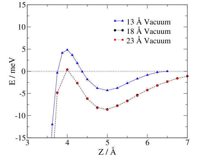
FIG. 4. The PBE interaction energy is plotted as a function of Z , using the same equilibrium 5-layer slab to model the W(110) surface, but using different vacuum spaces along the surface normal. The N_2 bond length has been kept equal to the equilibrium value of 1.117 Å. The zero of energy is defined as the energy of the molecule in its equilibrium geometry placed midway between two slabs.
