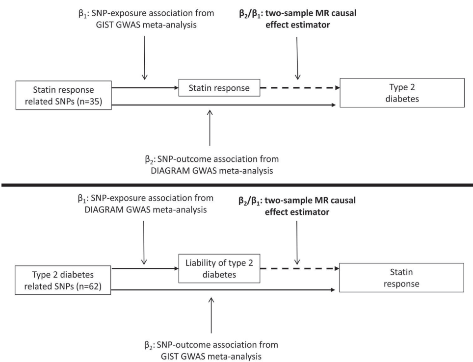
Figure 1. Overview of two-sample Mendelian randomization (MR) study on the bidirectional association between statin-induced LDL cholesterol response and type 2 diabetes (T2D). Top panel shows direction of statin response to T2D, bottom panel liability to T2D to statin response. Layout of figure based upon the work by Taylor et al. 2016 (PMID 27215954).
