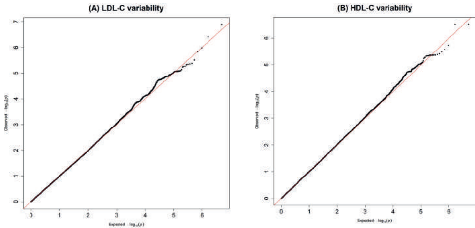
Supplemental Figure. Q-Q plots for the two genome-wide association analyses. Corresponding \lambda 's: (A) 0.995; (B) 1.002
