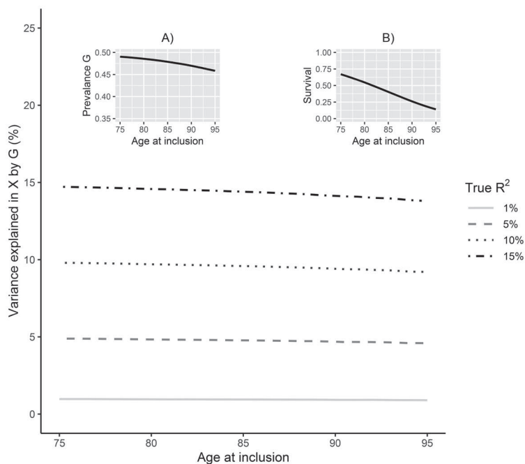
eFigure 2. Variance explained in the exposure of interest X by its genetic proxy G for an increasingly selected population, for a continuously distributed R . Shown in the insets are A) the prevalence of G and B) the accompanying survival curve, both with the true (i.e. unselected) R^2 set at 5%.
