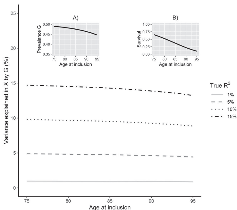
Figure 3. Variance explained in the exposure of interest X by its genetic proxy G for an increasingly selected population, when incorporating a binary R . Shown in the insets are A) the prevalence of G and B) the accompanying survival curve, both with the true (i.e. unselected) R^2 set at 5%.
