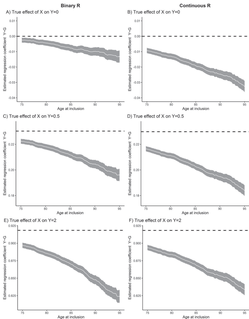
eFigure 9. Effect of survival bias on the association between the genetic instrument G and the outcome of interest Y , for different true effects of exposure X on Y . Data are presented as regression coefficients (95% CI) estimated with linear regression. The true (i.e. unselected) regression coefficient for G on Y is shown as a dashed line in each plot. Shown for binary (left column) and continuously (right column) distributed R .
