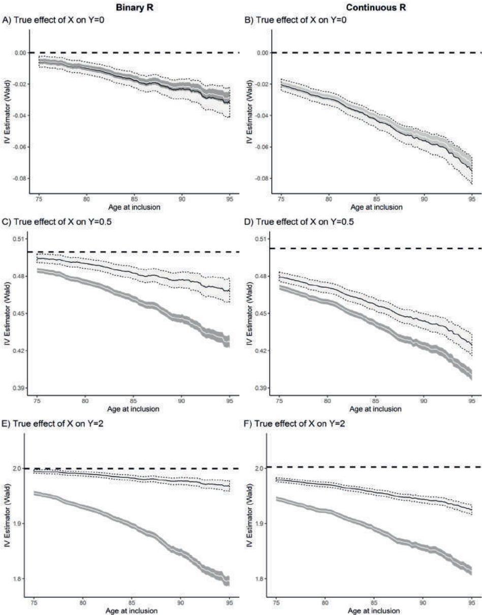
eFigure 10. Wald ratios (95% CI) based on internally (white ribbon) versus externally (grey ribbon) estimated association between exposure X and the outcome Y , for different true effects of exposure X on Y . Shown for binary (left column) and continuously (right column) distributed R . Dashed lines denote the true (i.e. unselected) Wald ratio, which equals the true causal effect of X on Y .
