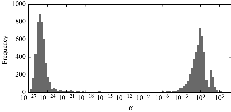
Figure 3.11: Distribution of the final value of E for 10^4 randomly generated/relaxed spring-connected eight-polygon systems [Fig. 3.8]. The left and the right clusters represent systems that relax to a zero energy state and a finite energy state respectively. The two well separated clusters allow to set a cutoff value of E , below which the system can be assumed to be at practically the zero-energy state and in which case CG can be terminated. This saves a considerable amount of computational power. We set the cutoff value of E to be at 10^{-10} .
