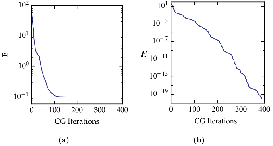
Figure 3.10: Conjugate Gradient (CG) convergence curve of a eight-polygon spring connected system [Fig. 3.8] that: (a) relaxes to a finite energy state and (b) relaxes to a zero energy state and forms a mechanism, at least in the vicinity of the relaxed state.
