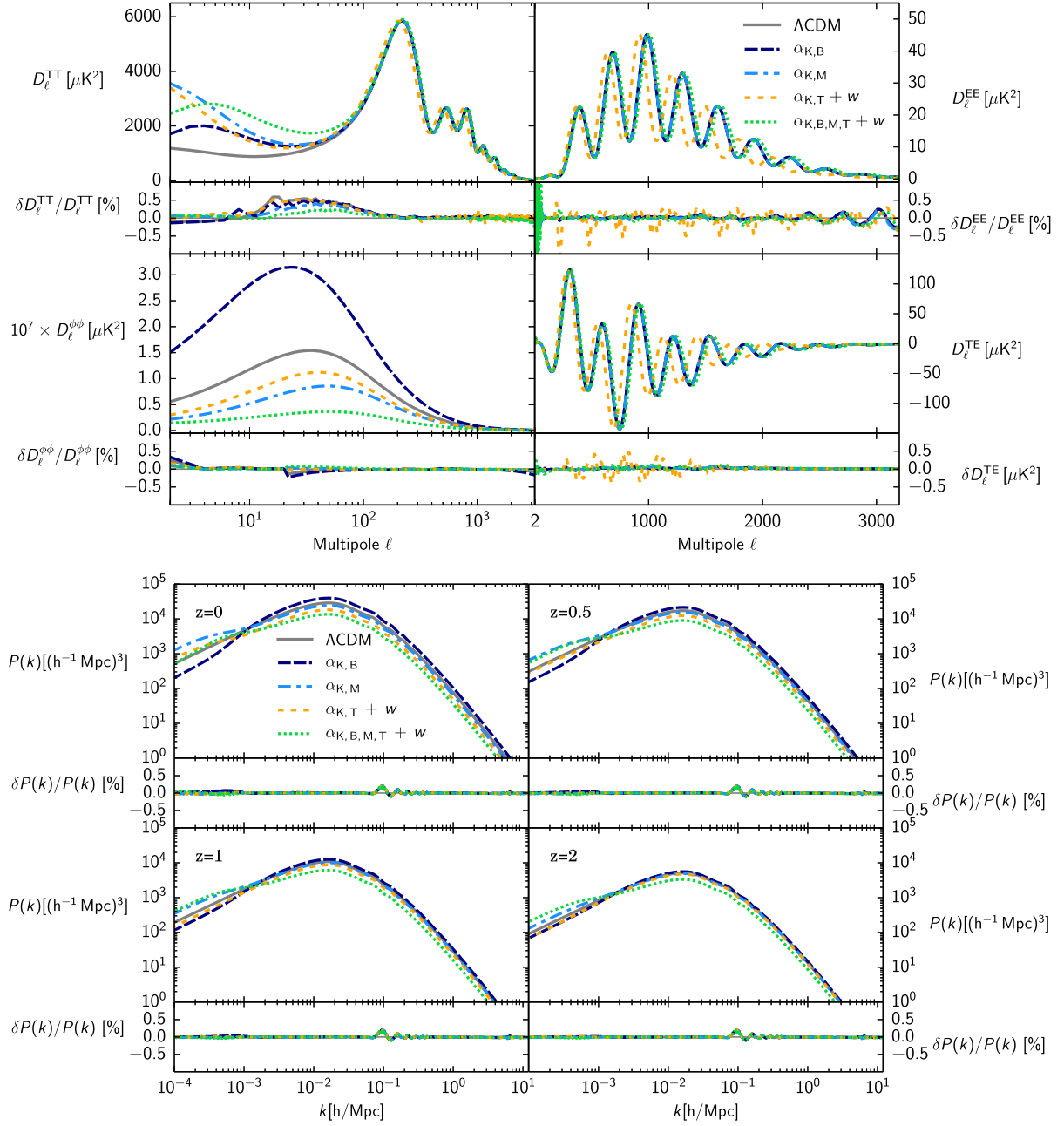
FIG. 9. Alphas. Top figure: The TT , EE , lensing, and TE angular power spectra of the CMB for a reference \Lambda\text{CDM} and four different choices of the \{w_{DE}, \alpha_i\} functions along with the relative difference between EFTCAMB and hi_class. Bottom figure: The same as in the top figure but for the matter power spectrum at different redshifts. The exact values for the cosmological parameters used here can be found in Appendix B 6.
