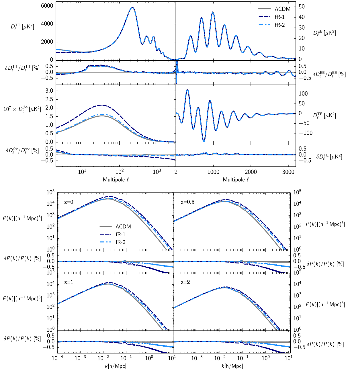
FIG. 6. f(R) . Top figure: The TT , EE , lensing, and TE angular power spectra of the CMB for two different f(R) models and a reference \Lambda CDM along with the relative difference between EFTCAMB and CLASS_EOS_fR. Bottom figure: The same as in the top figure but for the matter power spectrum at different redshifts. The exact values for the cosmological parameters used here can be found in Appendix B 3.
