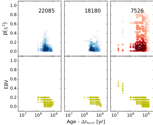
Figure 2. Probability ( p(\chi^2) , upper panels) and E(B-V) (lower panels) as a function of [age - \Delta t_{burst} ] of all the possible solutions in the SED-fitting process, for three red and dead candidates in the TH selection (IDs 22085, 18180 and 7526, chosen as examples of three levels of robustness in the selection, see also Fig. 4; the plot for the full TH sample is in Appendix D). The colours of the dots in the probability panels refer to the belonging of the source to the selection with (blue) or without (red) the inclusion of nebular lines. The dots (i.e. the models) are shaded as a function of their density. All the solutions have age > \Delta t_{burst} , as required to be classified as passive in this approach. Galaxies excluded from the selection, on the other hand, have been fitted by at least one model with age \leq \Delta t_{burst} , i.e. still star-forming, with a probability p_{sf} > 5\% (not shown).
