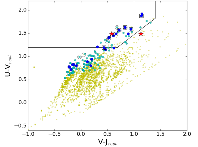
Figure 6. UVJ diagram for z_{CANDELS} > 3 sources, computed adopting the standard \tau -models to derive the rest-frame magnitudes. The passive selection region is defined by (U - V) > 0.88 \times (V - J) + 0.59 , (U - V) > 1.2 and (V - J) < 1.4 (Whitaker et al. 2011). Yellow points are the whole sample of z > 3 , Ks+3.6+4.5 \mu\text{m} H -detected galaxies from G13. Cyan small dots refer to the objects having a passive best-fit both with and without the inclusion of the emission lines in the TH library. Blue large dots are the 30 galaxies in the reference sample, with empty squares indicating the 10 sources selected also including nebular emission lines. The red stars refer to the candidates surviving the z -free selection. Finally, empty circles refer to the \tau -model red and dead selection ( sSFR < 10^{-11} \text{ yr}^{-1} , Sect. 5). Not all the galaxies in the selections are visible because some models have very similar rest-frame properties and colours, so that the symbols overlap.
