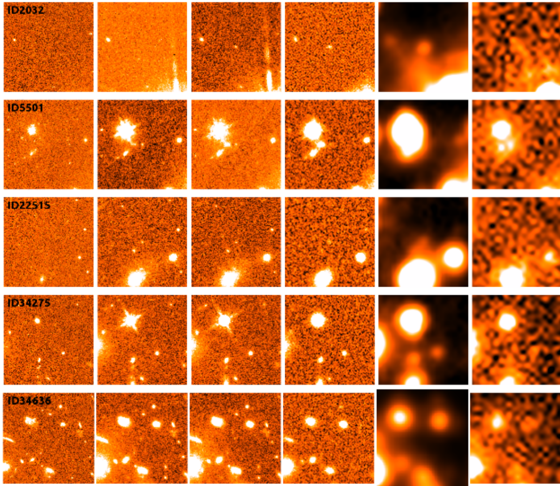
Figure E1: Snapshots of the 5 passive candidates selected with the \tau -models library which are not present in the reference sample. Left to right: ACS B435 + V606 + I814 stack, WFC3 J125 , WFC3 H160 , Hawk-I Ks , IRAC 3.6 + 4.5 \mu\text{m} stack, IRAC 5.8 + 8.0 \mu\text{m} stack.
