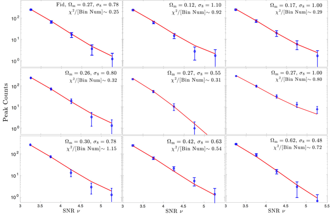
Figure A2. The peak count distribution of the selected simulations. The corresponding solid lines are the theoretical prediction with the input cosmological parameters.
