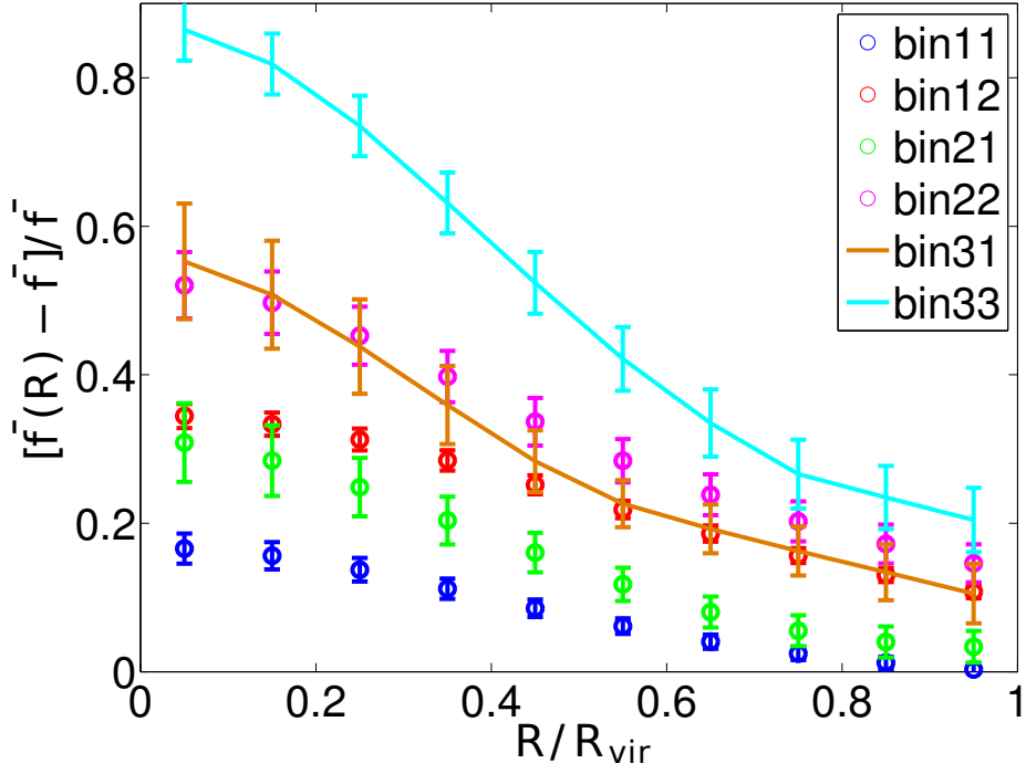
Figure D3. Excess galaxy number density (filling factor) distribution around cluster candidates for each bin. The error bars on the mean are estimated from a bootstrap analysis.
