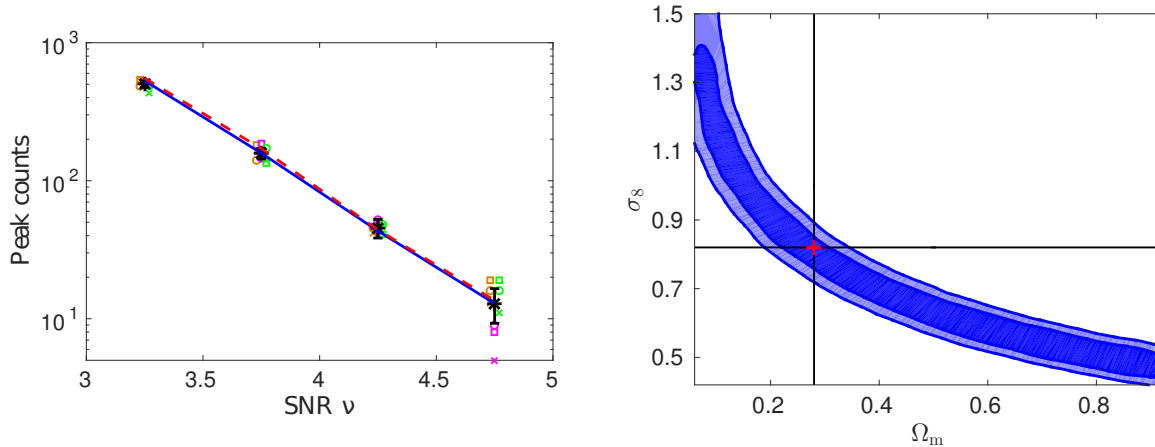
Figure C1. The results of the mock analysis. Left panel: The peak count distribution of the KiDS-450 mock data. The black ‘*’ denotes the average value of the 3 independent mocks. The error bars are the square root of the diagonal terms of the covariance matrix. The nine sets of symbols with different colours correspond to the 3 independent mocks with 3 different noise realizations. The solid blue line is the theoretical prediction with the input cosmological parameters. The dashed red line is the peak count of the smoothed convergence field including a uniform random noise field with the mean noise level of 9 mocks. Right panel: Cosmological constraints on (\Omega_m, \sigma_8) derived from the KiDS-450 mock peak count. The red ‘+’ denotes the input (\Omega_m, \sigma_8) .
