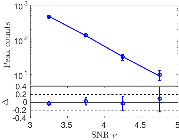
Figure 1. Upper panel: The fiducial peak count distribution of the KiDS-450 data. The corresponding solid line is the theoretical prediction with the best-fit cosmological parameters obtained from MCMC fitting. The error bars are the square root of the diagonal terms of the covariance matrix. Lower panel: The difference between the peak counts of the data and the best-fit theoretical predictions.
