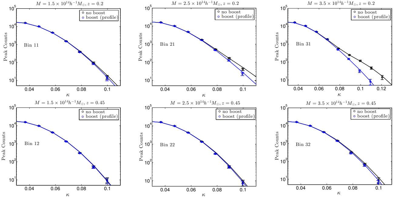
Figure D4. The peak distribution with and without the boost factor effects for different bins. The circles with error bars are the measurement from the mock analysis. The lines with different colour are the corresponding analytical predictions.
