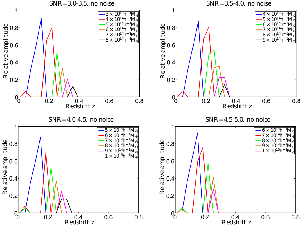
Figure D1. The fractional contributions of clusters with different mass and redshift to WL peaks of different heights using the KiDS-450 source redshift distribution without the shape noise.
