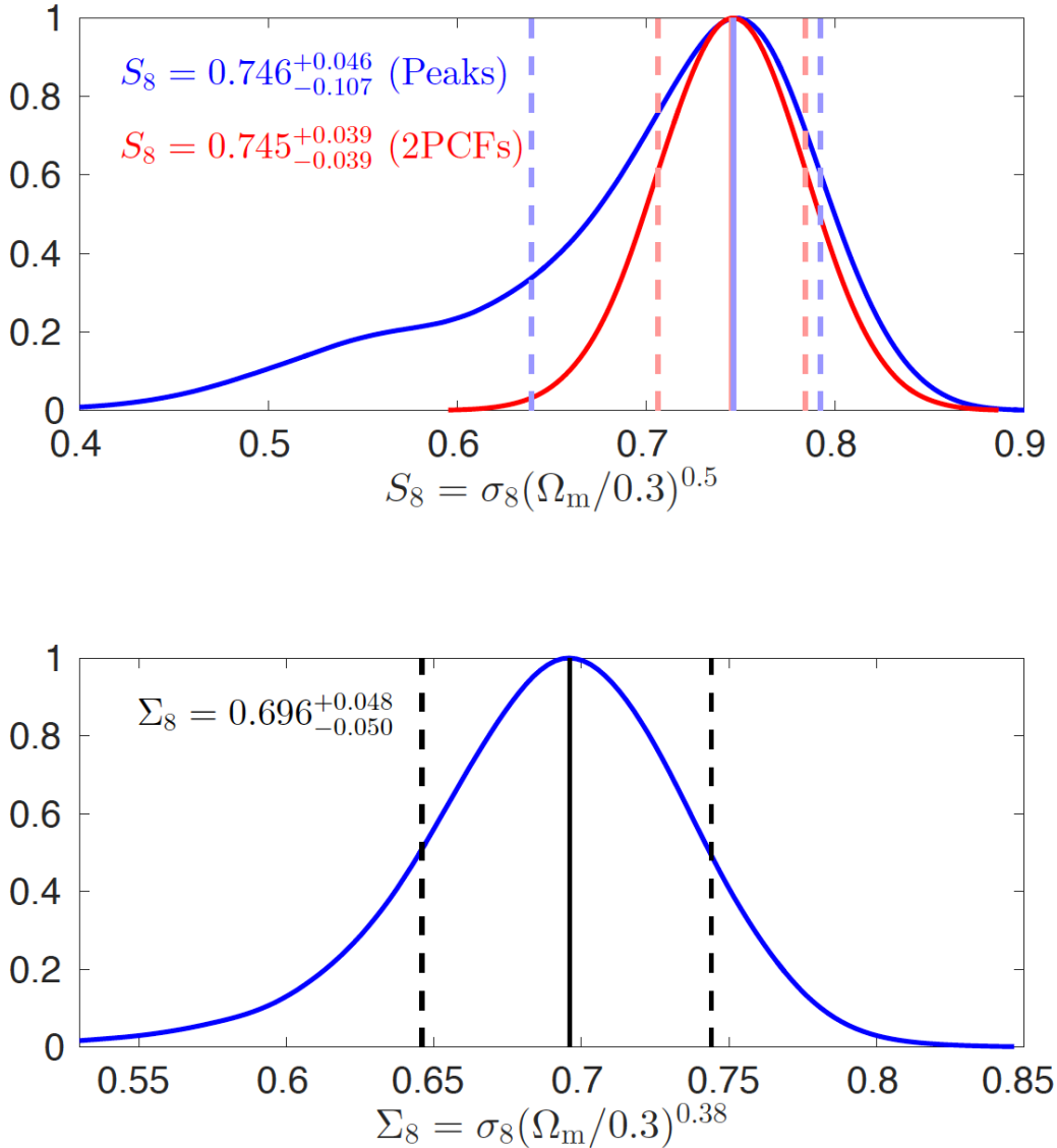
Figure 4. Upper panel: The marginalised probability distribution of S_8 for KiDS-450 WL peak statistics (blue) and the cosmic shear tomographic 2PCFs analysis (red). Lower panel: The marginalised distribution of \Sigma_8 for KiDS-450 WL peak statistics.
