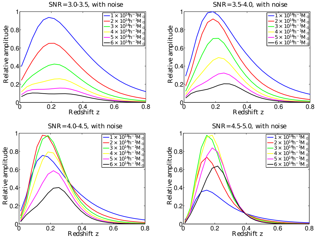
Figure D2. The fractional contributions of clusters with different mass and redshift to WL peaks of different heights using the KiDS-450 source redshift distribution with KiDS-450-like shape noise.
