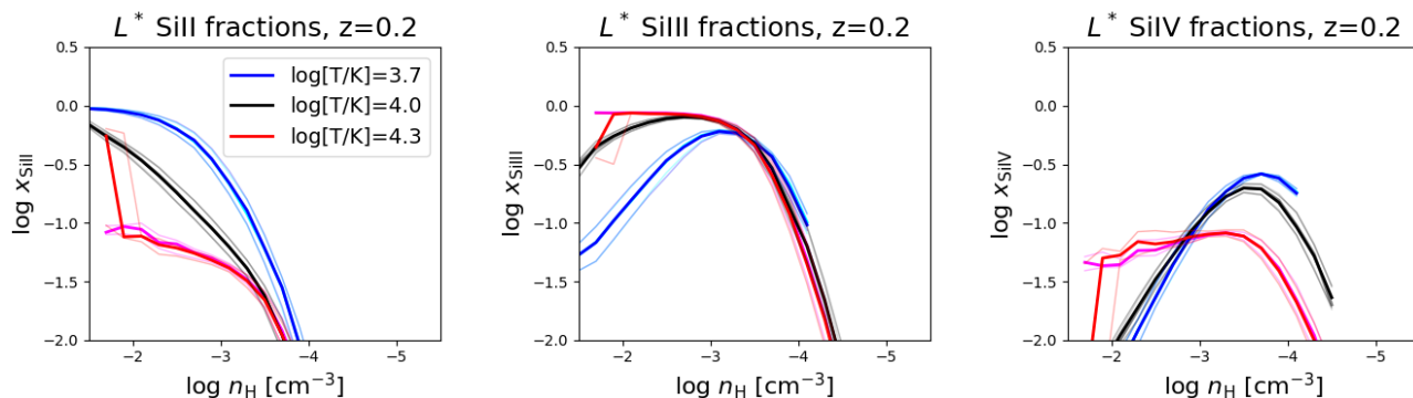
Figure A2. Median silicon ionization fractions, x_{\text{ion}} , of gas particles as a function of density at z = 0.2 for three temperatures ( T = 10^{3.7} K in blue, 10^{4.0} K in black, and 10^{4.3} K in red) for the NEQ runs. Particles are selected from L^* zooms to lie within 300 kpc of the central galaxy. We also show the ionization fractions for ioneq(NEQ) runs in cyan, grey, and magenta, and for the most part they lie directly beneath the NEQ curves except for instances where there is little data. The 1-\sigma spreads are also shown with thin lines and do not indicate a greater spread for NEQ versus ioneq(NEQ) runs.
