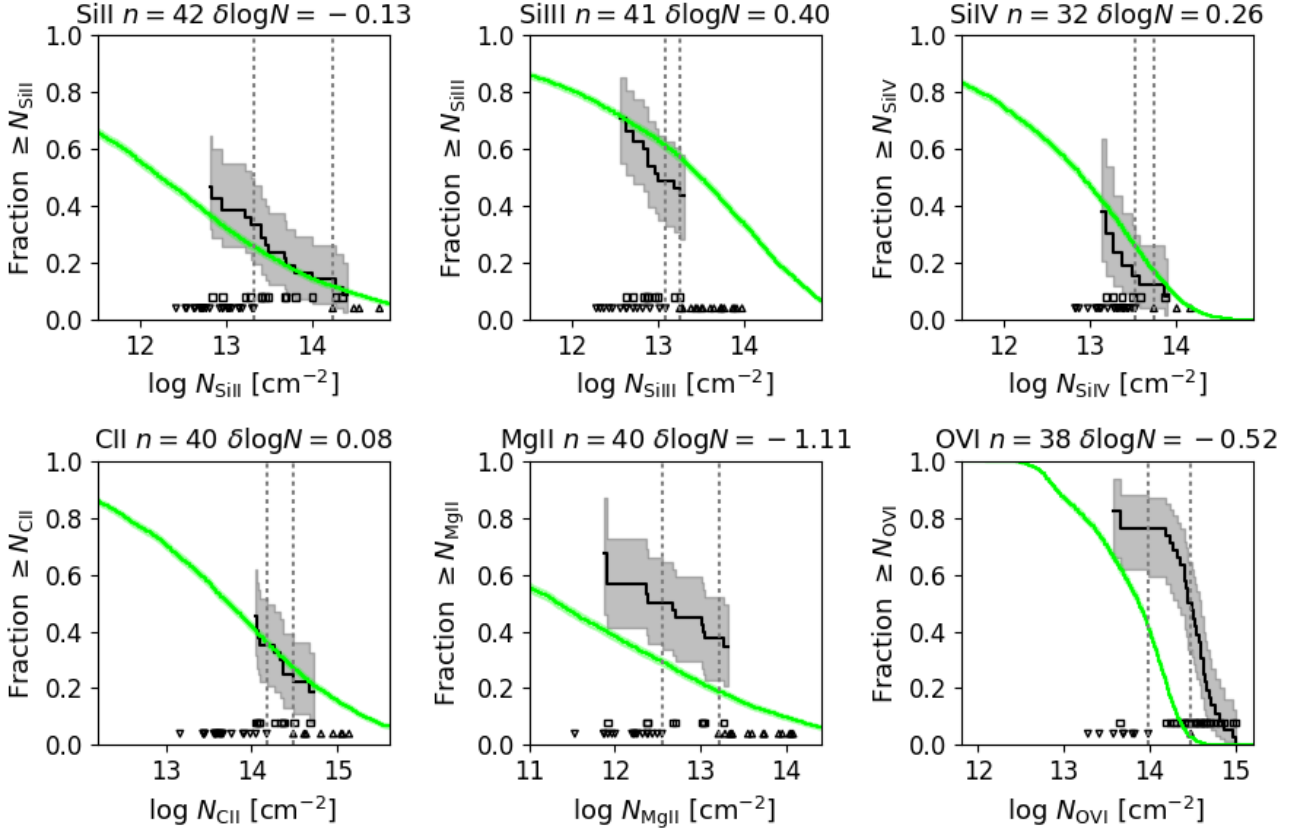
Figure 5. Cumulative distribution functions (CDFs) of COS-Halos column densities for various ions (black step function with shading indicating 95% confidence limits) compared to the simulated CDFs (thin green band) generated from 100 SMOHALOS realizations. The Kaplan-Meier method is applied to handle upper and lower limits. The total number of observations ( n ) is listed on the top along with the average difference in column density between observations and simulations ( \delta\log N ). The three silicon ions (Si II, Si III, & Si IV) are shown on top and C II, Mg II, and O VI are shown on the bottom. The input datapoints are shown along the bottom: squares for detections, upside-down triangles are upper limits, and upwards pointing triangles are lower limits. Two-sided censoring results in the observed CDFs never reaching 0 or 1. Vertical dotted lines encompass the range over which K-M estimation is not required.
