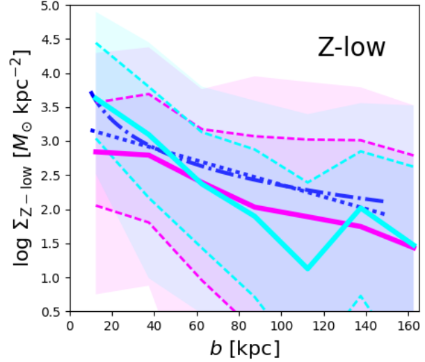
Figure 9. The median low ions metal surface densities for the 28 star-forming galaxies (thick solid cyan line from 100 SMOHALOS realizations) derived from summing Si II, Si III, and Si IV compared to the COS-Halos low-ion metal surface densities derived from W14 CLOUDY modelling as reported in Peeples et al. (2014) (blue dotted lines, 2 different functional fits shown). One \sigma dispersions are indicated by dashed lines. The passive SMOHALOS realizations are displayed in magenta for comparison.
