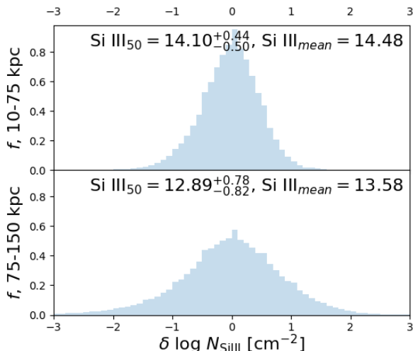
Figure 10. The residual distributions of Si III column densities after subtracting the median column density profiles plotted in Fig. 2. The distributions of \delta \log N_{\text{Si III}} are calculated across 9 L^* galaxies and binned into two impact parameter bins (10 – 75 kpc in the upper panel, and 75 – 150 kpc in the lower panel). For each bin, we list the median value of \log N_{\text{Si III}} and the 1 - \sigma range, as well as the mean \log N_{\text{Si III}} .
