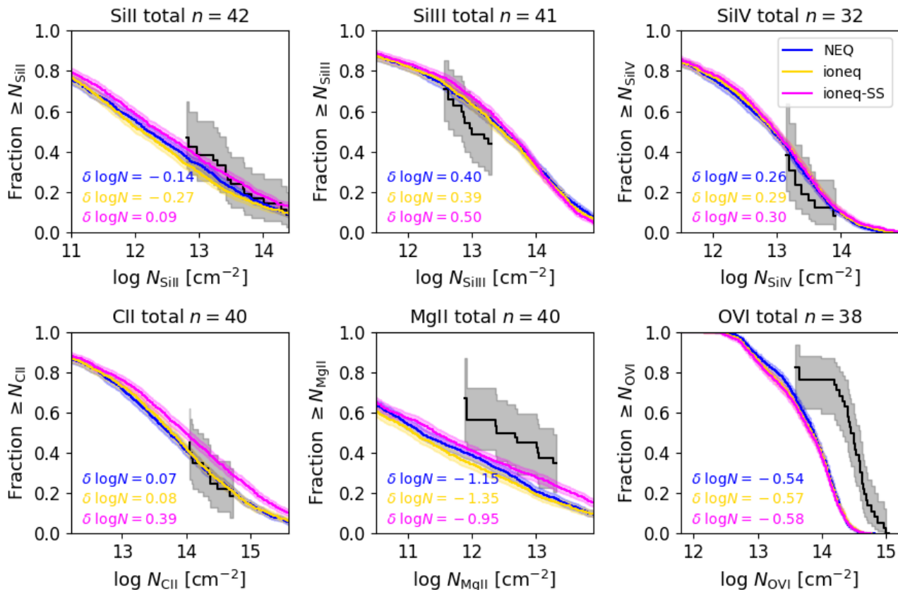
Figure 7. Kaplan-Meier CDFs for the entire COS-Halos sample, as in Fig. 5, compared to different model variations. The z = 0.20 NEQ sample in blue is compared to standard equilibrium EAGLE simulations of the same haloes assuming ionization equilibrium for the uniform Haardt & Madau (2001) background (gold), and then applying a self-shielding criterion following the Rahmati et al. (2013) prescription (magenta).
