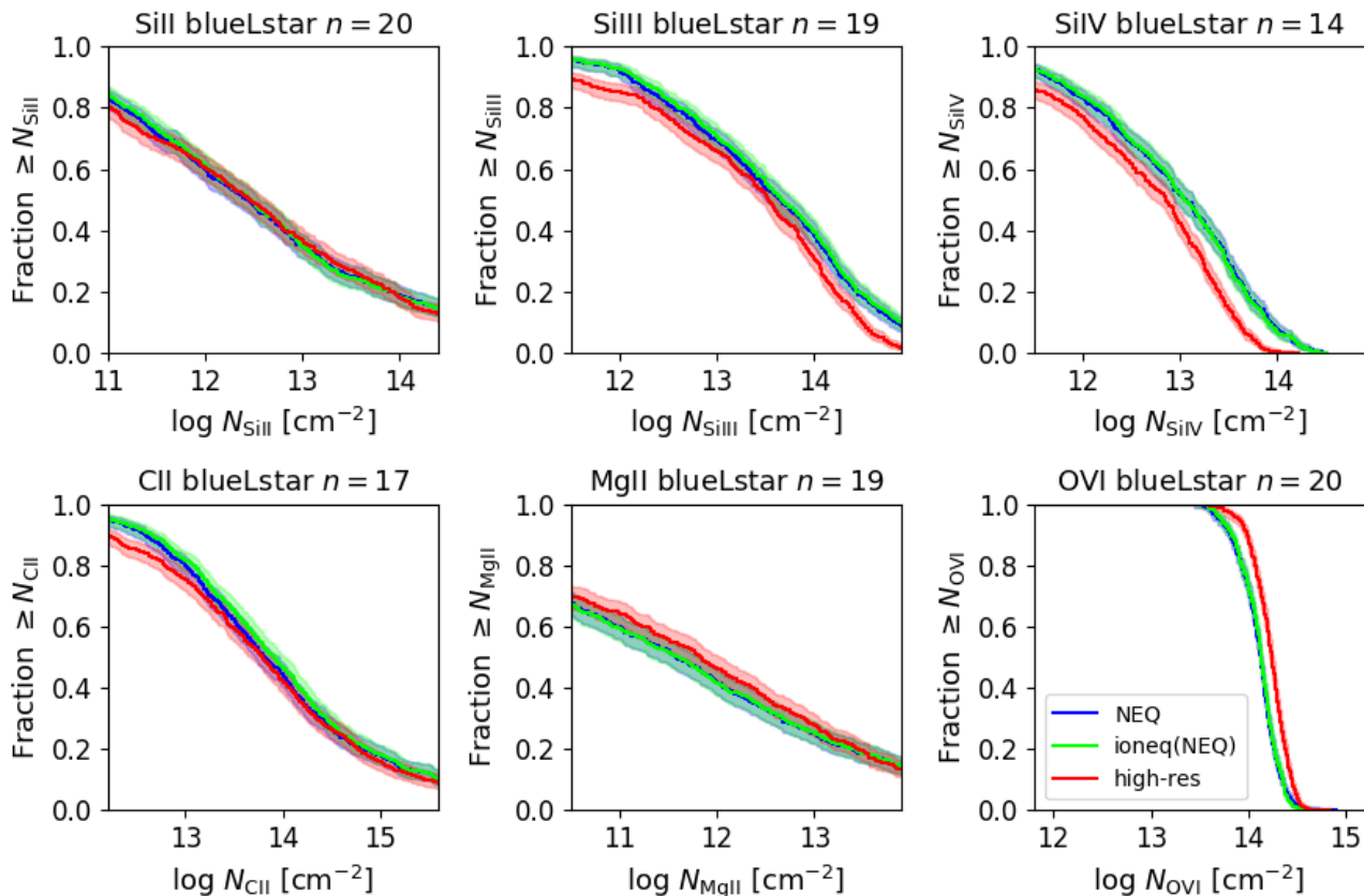
Figure A1. SMOHALOS cumulative distribution functions simulating the COS-Halos blue L^* galaxies using three zoom simulations hosting star-forming galaxies in haloes of 10^{12.1} - 10^{12.3} M_\odot , all at z = 0.2 . Blue indicates the standard NEQ simulations, green (often overlapping blue curves) indicates the NEQ simulations where ionization equilibrium is assumed, and red shows higher resolution NEQ M4.4 resolution simulations.
