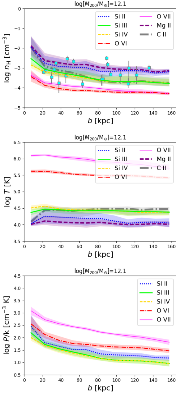
Figure 11. Physical properties weighted by ion column density as a function of impact parameter around the 10^{12.1} M_{\odot} halo. Hydrogen number density and temperature are shown in the upper and middle panels for low species (Si II, Si III, Si IV, C II, Mg II) as well as O VI. Additionally, O VII is shown to indicate the hot halo component, where most CGM metals reside in an L^* halo. Pressure, calculated by taking n_H \times T / (X_H \mu) is also plotted. COS-Halos densities derived from low ion modelling (Prochaska et al. 2017) around L^* appear as cyan squares.
