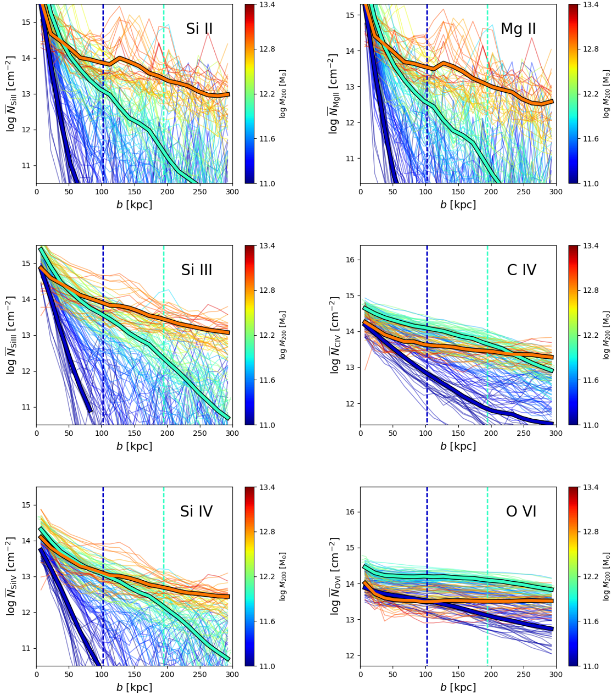
Figure 2. Linearly averaged column densities as a function of impact parameter at z = 0.2 , coloured by halo mass for silicon species on the left (Si II, Si III, & Si IV from top to bottom) and for Mg II, C IV, and O VI on the right. Individual galaxies in isolated projections are shown as thin lines, and averages for sub- L^* , L^* , and group-sized haloes (blue M_{200} = 10^{11.0} - 10^{11.3} M_{\odot} , aquamarine 10^{11.7} - 10^{12.3} M_{\odot} , & orange 10^{12.7} - 10^{13.3} M_{\odot} ) are shown as bordered, thick lines. Dashed vertical lines indicate average R_{200} for the 3 samples (the group haloes have R_{200} = 384 kpc). The column density range for each panel is scaled according to the relative abundance of each element in the simulation. Hence, the relative locations of the curves within their panels reflect the differences in ion fractions.
