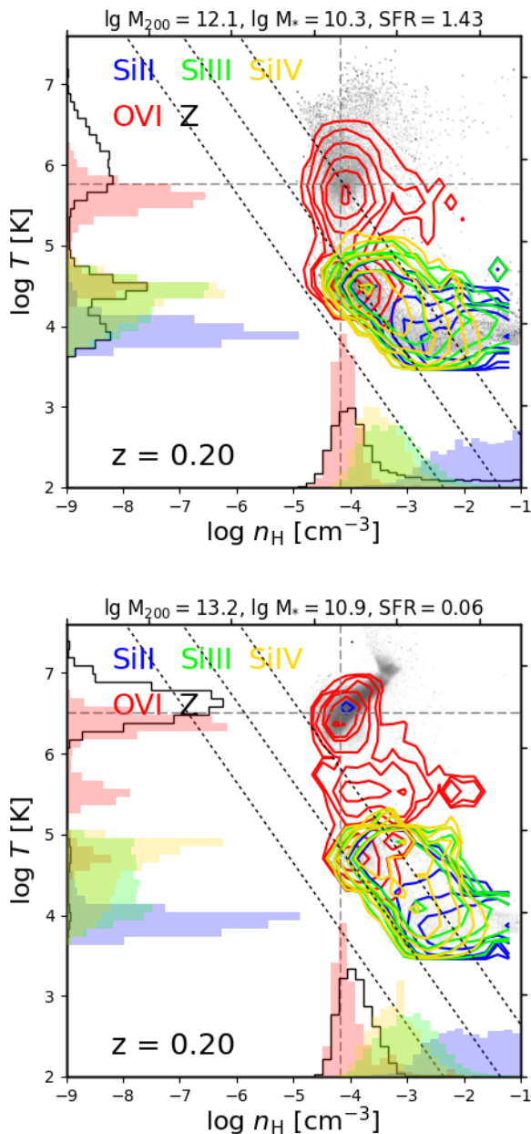
Figure 12. Density-temperature phase space diagrams of Si II (blue), Si III (green), Si IV (gold), O VI (red), and metals (grey shading) gas inside R_{200} for a typical L^* halo (upper panel) and group halo (lower panel) at z = 0.2 . Corresponding histograms along the bottom and left indicate the density and temperature distribution for each ion, respectively. The dashed grey horizontal line indicates T_{\text{vir}} and the dashed grey vertical line indicates 200 \times the critical overdensity. Dotted diagonal lines indicate isobars at 1, 10, and 100 \text{ cm}^{-3} \text{ K} from left to right.
