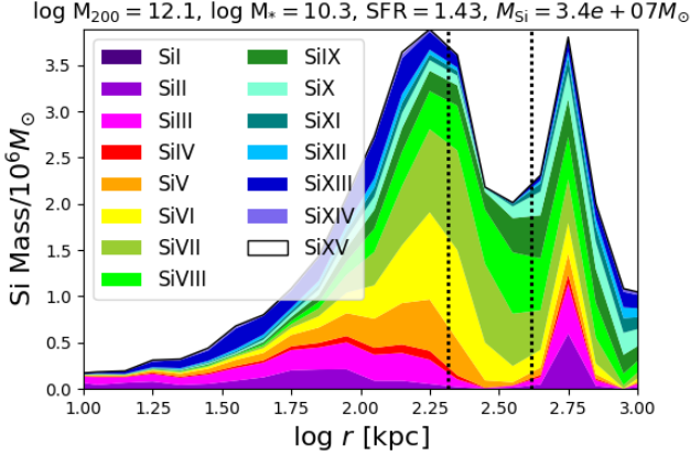
Figure 8. CGM silicon as a function of radius for a M_{200} = 10^{12.1} M_{\odot} z = 0.2 L^* galaxy, subdivided by ion and summed in 0.1 dex radial bins. The total silicon mass budget is 3.4 \times 10^7 M_{\odot} between 10 and 1000 kpc. The dotted vertical lines indicate R_{200} and 2R_{200} , and the secondary bump beyond 2R_{200} belongs to a neighbouring sub- L^* galaxy.
