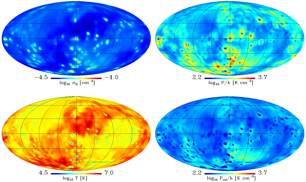
Figure C1. Mollweide projections of SPH particles at 0.3R_{200} of our reference 10^{12.1}M_{\odot} halo. Density and temperature (upper and lower left panels) show a multiphase structure of dense, cool CGM embedded in a hot ambient medium. The pressures (upper right panel) show much less variation between the phases, although some of the cool clumps appear to be at lower particle pressures. The weighted pressure used in the hydro equations of motion is shown in the lower right panel and yields much smaller pressure differences.
