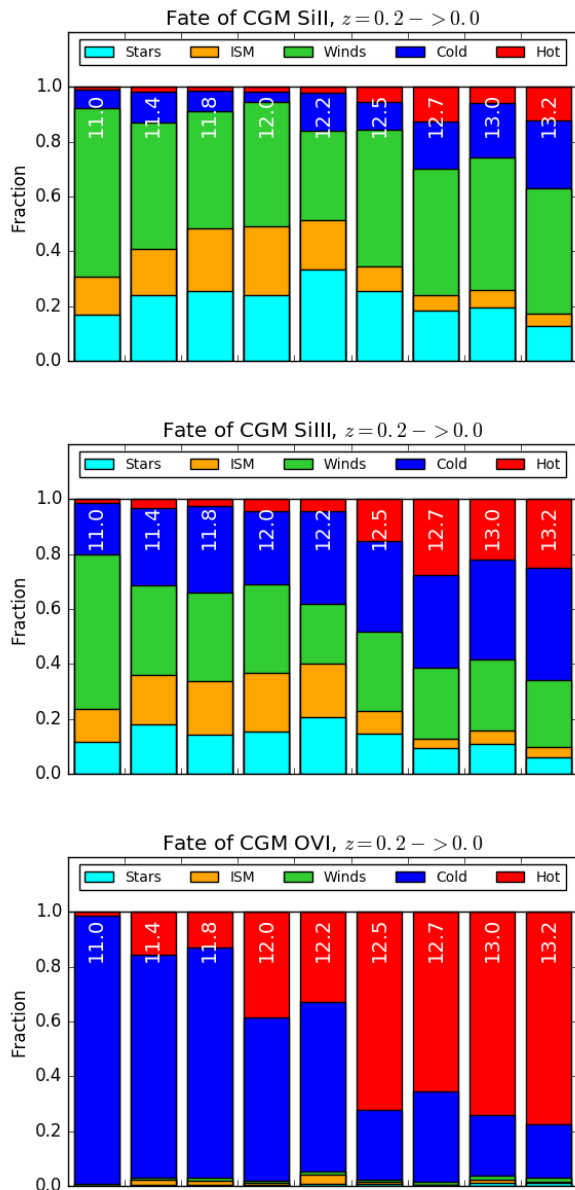
Figure 15. Tracking of gaseous ion species (Si II, Si III, and O VI from top to bottom) inside 500 kpc at z = 0.2 for haloes increasing in mass from left to right ( \log[M_{200}/M_{\odot}] indicated in white). The bars indicate the fate of the gas traced by each ion at z = 0 , with the possibilities that it joined a galaxy (converted into stars, resides in ISM, or returned to the CGM) or remains in the CGM (cold and hot phases divided by T = 10^{5.0} K).
