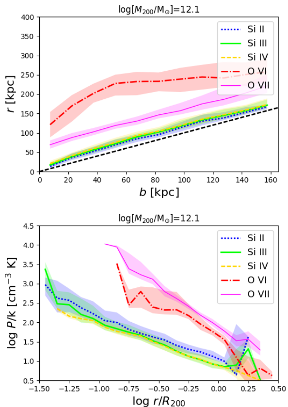
Figure 13. The upper panel shows column density-weighted mean physical radius, r , for a given ion plotted as a function of impact parameter for silicon species, O VI, and O VII for the reference M_{200} = 10^{12.1} M_{\odot} halo. The 1-to-1 correspondence is plotted as a dashed black line. Cool silicon species show r \sim b , while O VI in contrast arises from much larger physical radii at a given impact parameter (O16) and traces a physically and spatially distinct phase at a given impact parameter. The lower panel plots ion-weighted pressure as a function of radius, indicating cool silicon ions and warm-hot oxygen species trace different pressures at the same physical radius.
