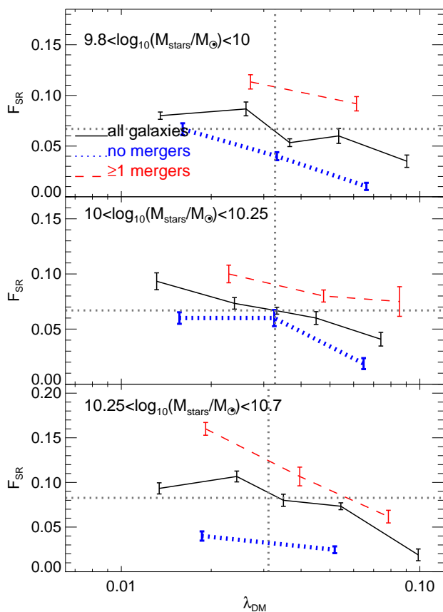
Figure 16. The fraction of central galaxies that are slow rotators at z = 0 (defined as those with \lambda_{r50} \leq 0.1 ) as a function of the halo spin parameter, \lambda_{\text{DM}} , in three bins of stellar mass of the central galaxy, as labelled in each panel. We show this for 3 samples: all central galaxies (solid line), and the subsamples that had at least 1 merger (dashed line) or no mergers (dotted line). Bins are chosen to have \approx 150 galaxies. Error bars correspond to 1 standard deviation calculated with 10 jackknife resamplings in individual mass bins. The horizontal and vertical line shows the fraction of slow rotators for all galaxies at z = 0 in the stellar mass bins and their median \lambda_{\text{DM}} . There is a clear tendency for low \lambda halos to have a higher fraction of slow rotators.
