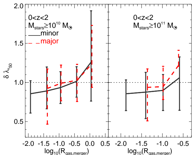
Figure 13. Variation of \lambda_r measured at r_{50} as a function of the gas to stellar mass ratio of the merger (see Eq. 8) separating minor and major mergers, as labelled. The left panel shows all the mergers that took place in galaxies with M_{\text{stars}} \geq 10^{10} M_{\odot} at 0 \leq z \leq 2 , while the right panel shows the subsample of galaxies with M_{\text{stars}} \geq 10^{11} M_{\odot} . Lines with error bars show the median and 25 th – 75 th percentile ranges. Only bins with \geq 5 objects are shown. For reference, the dotted horizontal line shows no change in \lambda_r . Positive values indicate the merger remnant has a higher value of \lambda_r than the progenitor.
