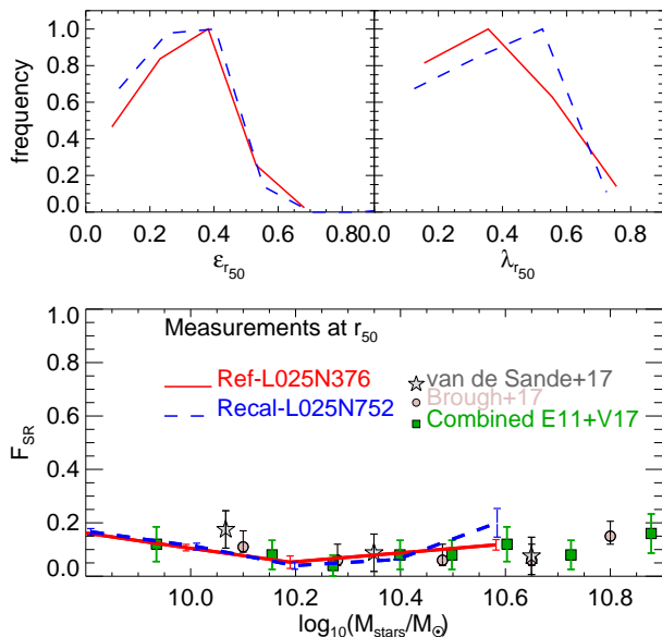
Figure A2. Top panel: Normalised histograms of \lambda_{r50} and ellipticity, measured adopting edge-on orientation, for the galaxies in Fig. A1. The solid and dashed lines correspond to the Ref-L025N0376 and Recal-L025N0752 simulations, respectively. The high-resolution simulation produces slightly more galaxies of high \lambda_{r50} . Bottom panel: Fraction of slow rotators using the classification of Cappellari (2016) as a function of stellar mass in the Ref-L025N0376 (solid line) and Recal-L025N0752 (dashed line) simulations. Because of the small volume of these simulations, we lack the massive galaxies, and thus we only show the range in which the statistics is good. Error bars correspond to 1 standard deviation calculated with 10 jackknife resamplings in individual mass bins. Both simulations agree well within the error bars suggesting that the fraction of slow rotators is well converged despite Recal-L025N0752 producing a slightly higher abundance of galaxies with high \lambda_{r50} .
