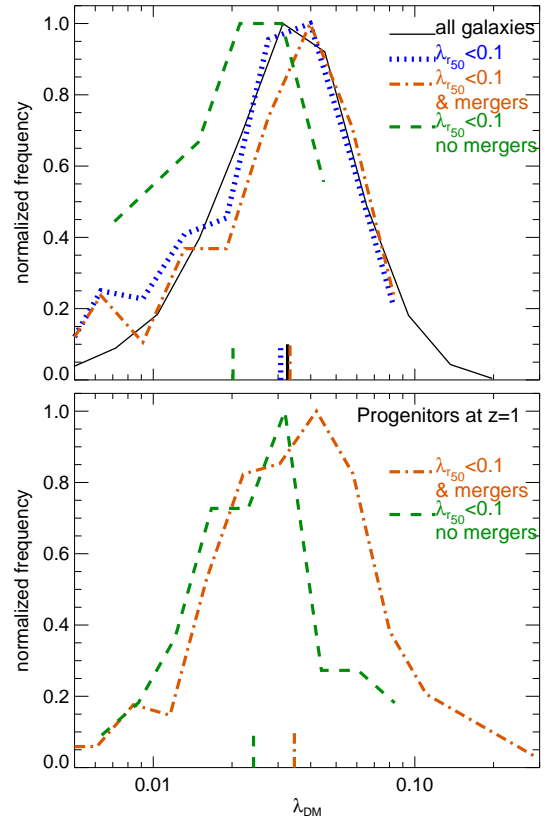
Figure 15. Top panel: The dark matter halo \lambda for central galaxies in EAGLE at z = 0 that have M_{\text{stars}} \geq 10^{10} M_{\odot} . Four subsamples are presented: all galaxies (solid line), those with \lambda_{r_{50}} < 0.1 (dotted line), those with \lambda_{r_{50}} < 0.1 and that had at least 1 merger in the last 10 Gyr (dot-dashed line), and those with those with \lambda_{r_{50}} < 0.1 that have not had any mergers in the same period of time (dashed line). Bottom panel: As in the top panel but for the progenitor halos at z = 1 of the two populations of slow rotators at z = 0 : (i) those that experienced mergers, and (ii) those that did not. We find that the host halos of slow rotators that at z = 0 have not yet experienced mergers, are biased towards low spins even at z = 1 .
