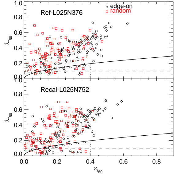
Figure A1. \lambda_{r50} as a function of ellipticity for galaxies in the Ref-L025N0376 (top panel) and Recal-L025N0752 (bottom panel) simulations that have M_{\text{stars}} \geq 5 \times 10^9 M_{\odot} at z = 0 . Circles and squares show galaxies seen edge-on and randomly, respectively. The three lines correspond to different classifications of slow rotators, and are as in Fig. 3.
