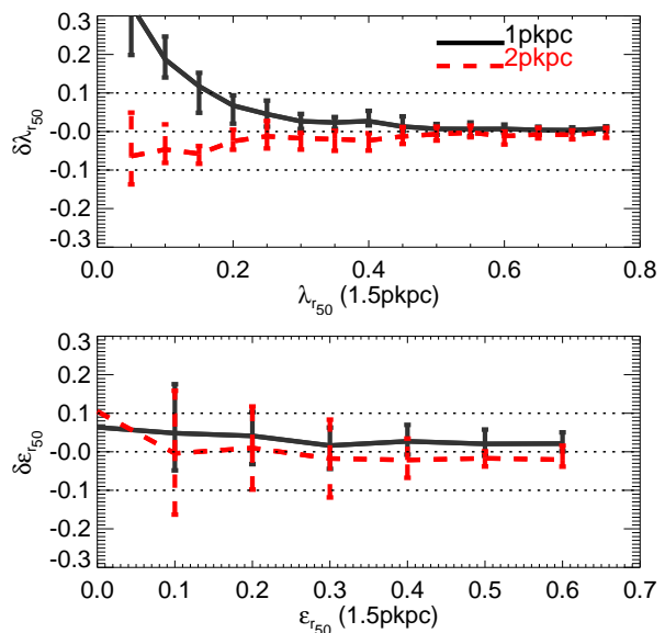
Figure A4. The fractional variation of \lambda_{r50} (top panel) and \epsilon_{r50} (bottom panel) as a function of these two quantities using bins of 1 and 2 pkpc, as labelled (see Eq. A1 for a definition of the fractional variation). Lines and error bars show the median and 25 th – 75 th percentile ranges. In this test we use the Ref-L050N0752 simulation and show all galaxies at z = 0 that have M_{stars} \geq 10^{10} M_{\odot} .
