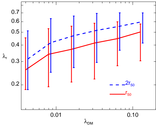
Figure 14. \lambda_R measured within r_{50} and 2r_{50} , as labelled, as a function of the dark matter halo \lambda (Eq. 11) for central galaxies in EAGLE at z = 0 that have M_{\text{stars}} \geq 10^{10} M_{\odot} . Lines with error bars show the median and 16 th – 84 th percentile ranges, respectively.
