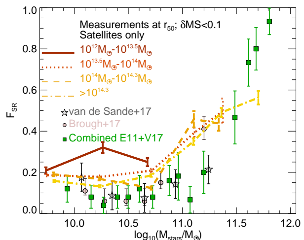
Figure 9. As in the bottom panel of Fig 8 but for passive satellites (i.e. those with \delta MS < 0.1 ).
