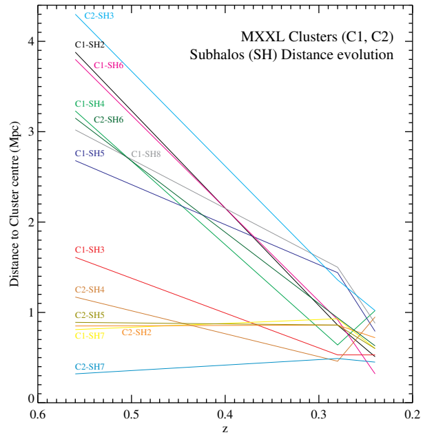
Figure 2. Projected distances to the main halo center as a function of redshift for the two MXXL clusters’ subhalos as listed in Table 4.
