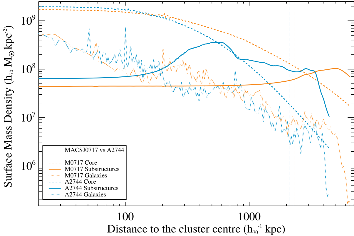
Figure 5. Density profile of the different components in MACSJ0717 (orange) and Abell 2744 (cyan) as a function of the distance to the cluster center: the core component (dashed line), the galaxy component (dotted lines) and the substructure component (plain lines). We differentiate between galaxies and (massive) substructures. The (long) dashed vertical lines highlight R_{200} for both clusters, MACSJ0717 and Abell 2744 in orange and cyan respectively.
