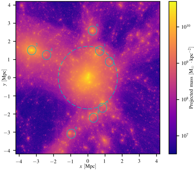
Figure 3. Projected mass map of halo CE-29 of the C-EAGLE simulation suite at z = 0.47 centered on the cluster’s minimum of potential. At this time the halo has a mass M_{200} = 9.15 \times 10^{14} M_{\odot} and a spherical over-density radius R_{200} = 1.72 Mpc (dashed circle). The small cyan circles indicate the eight subhalos that have a projected mass in a circular aperture of radius 250 kpc larger than our threshold for detection (see text for details). The overall distribution of sub-structures is in qualitative agreement with what is observed in the MACSJ0717 lensing mass map.
