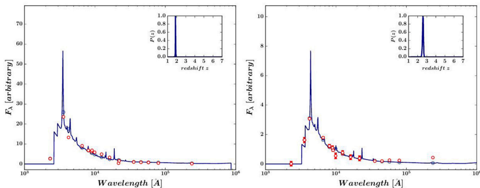
FIGURE 2 | Typical examples of the spectral energy distribution for two candidate quasars identified using our selection method. In each case the best-fit quasar template (as derived from the EAZY calculation) is also plotted. Red circles are the photometric points and the blue circles indicate the predicted photometry by the best-fit template. The photometric redshifts for objects are 1.87 and 2.57, respectively. The probability density distributions (PDFs) for each object are shown in the small inset. These PDFs strongly suggest that these objects are located at high- z . The Ly \alpha line in the two candidate quasars is clearly identified as an abrupt break in the quasar SED between the NUV-GALEX band and U_{\text{spec}} and B_W filters, respectively.
