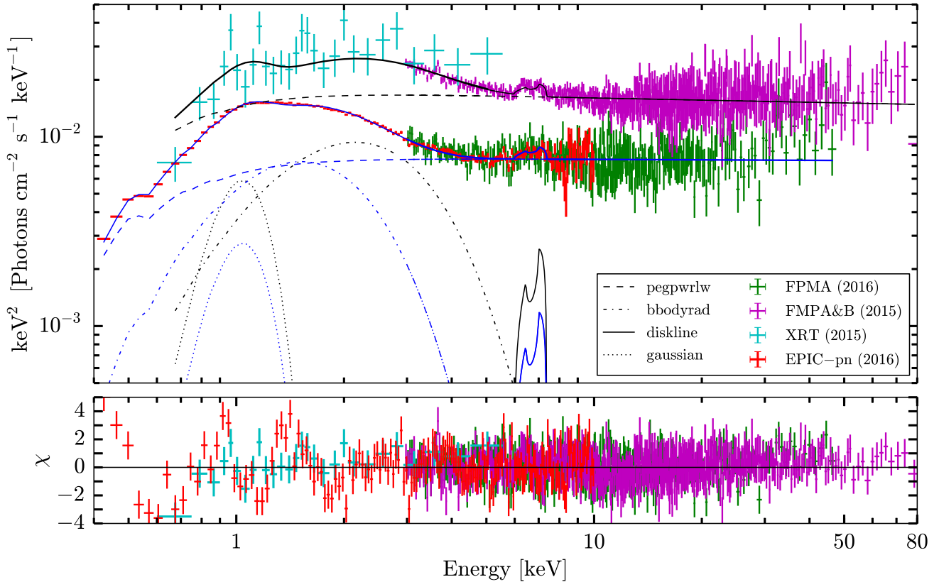
Figure 3. The best-fitting relativistic-reflection model with the XMM-Newton EPIC-pn, Swift -XRT, and two NuSTAR observations. Top: All spectra unfolded around the best-fitting \text{CONSTANT} \times \text{TBABS} \times (\text{BBODYRAD} + \text{PEGPWLW} + \text{GAUSS} + \text{DISKLINE}) model. For visual clarity, the two sets of simultaneously observed spectra have separately been rescaled by their fitted cross-calibration constant. For the same reason, we also do not plot the 2016 FPMB spectrum, which is consistent with the FPMA data. See Section 3.2 for details on which parameters were tied between the two observational epochs. Bottom: Residuals of the best-fitting relativistic reflection model. Note that despite the Gaussian component, residual structure remains around \sim 1 keV, which we investigate in detail in Section 4.
