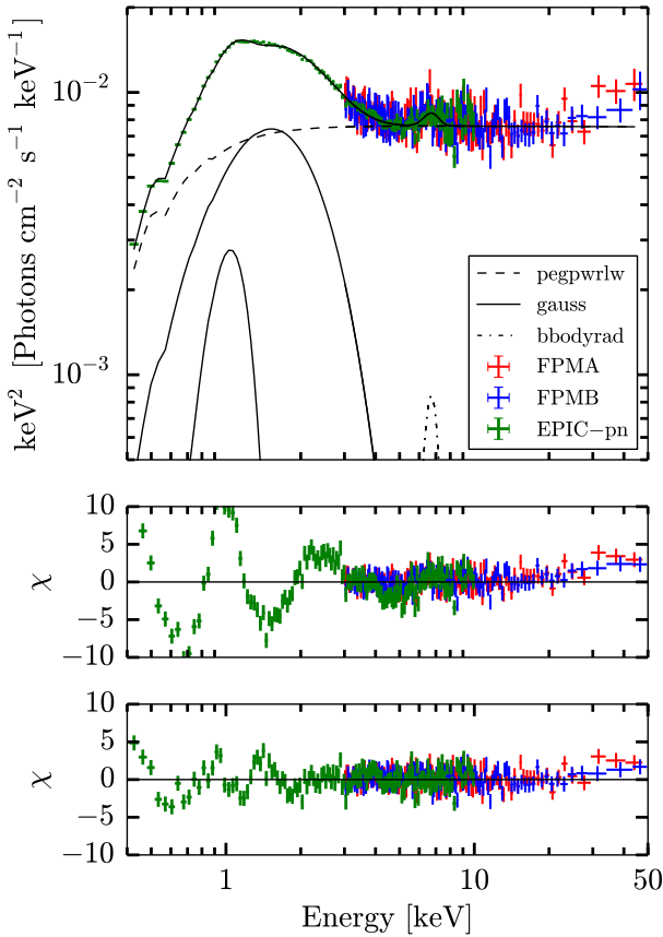
Figure 1. Top: The 2016 XMM-Newton EPIC-pn (green) and NuSTAR FPMA (red) and FPMB (blue) spectra unfolded around the best-fitting phenomenological model \text{CONSTANT*TBABS*}(\text{BBODYRAD}+\text{PEGPWRLW}+\text{GAUSS}+\text{GAUSS}) . The FPMB and EPIC-pn spectra have been rescaled by their fitted cross-calibration constant for visual clarity. Middle: \chi for the phenomenological model in D17, showing a broad Fe K \alpha feature and an emission feature around \sim 1 keV. Bottom: \chi for the best-fitting phenomenological model. We discuss the residuals remaining below 2 keV in detail in Section 4.
