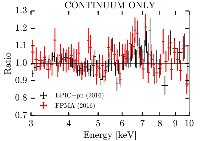
Figure 2. Data-to-model ratio of the 2016 XMM-Newton EPIC-pn (black) and NuSTAR FPMA (red) spectra fitted with a simple continuum model (see Section 3.1). An excess emission feature around the Fe K \alpha energy (6.4–6.97 keV) is clearly visible. The spectrum has been rebinned for visual purposes.
