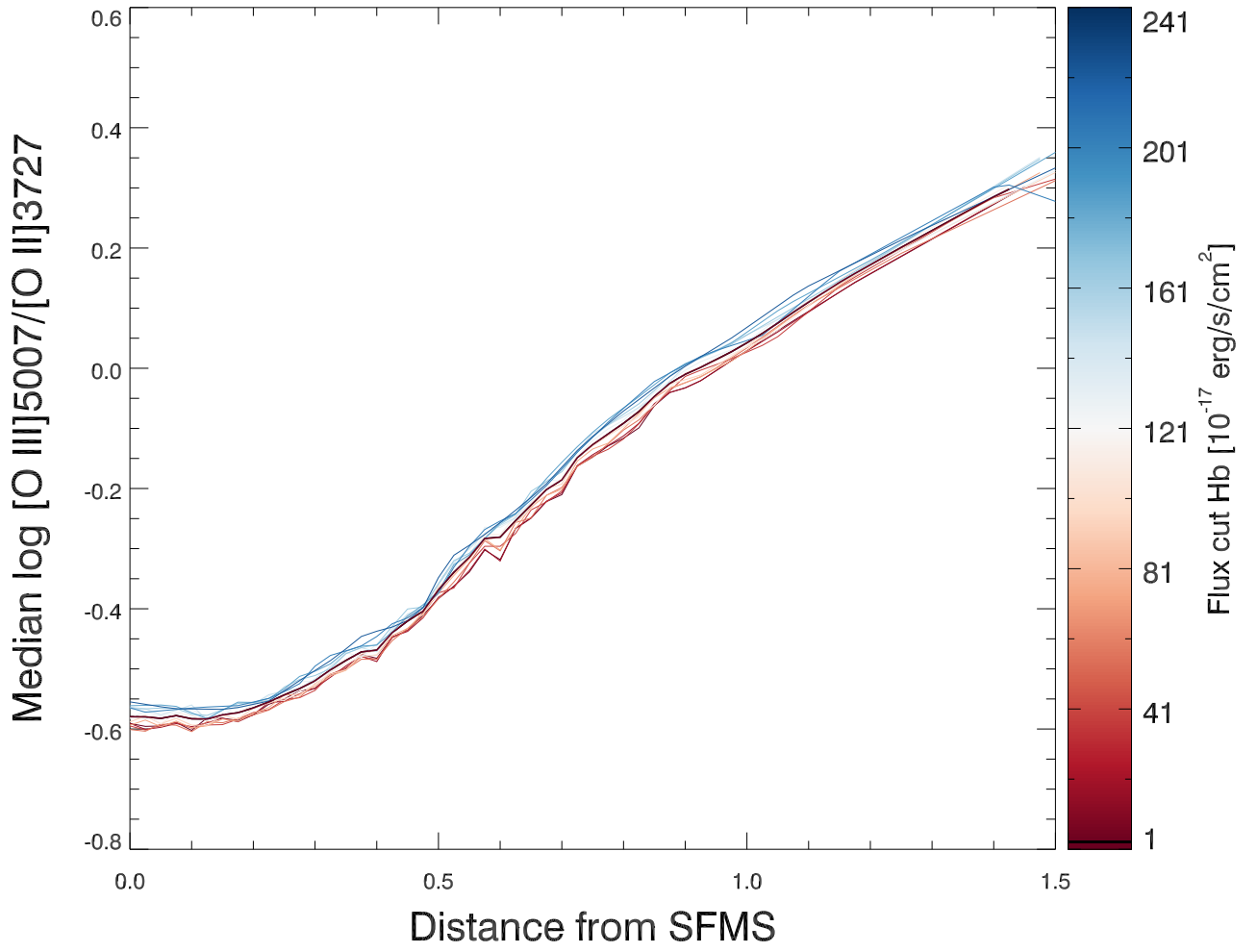
Fig. B.1. Median of the logarithm of O32 versus the distance to the SFMS of Eq. 1, shifted by 0.2 in the \log \text{SFR} - 2.93 \log(1+z) direction to correct for the different flux measurements method for the SDSS data. The colours indicate the \text{H}\beta flux cut.
