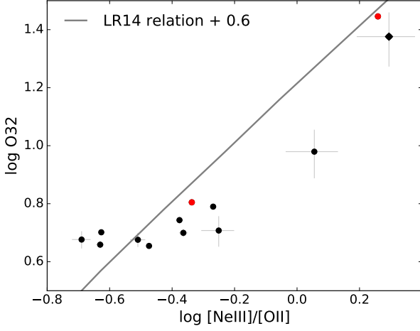
Fig. 17. Log O32 versus the log [Ne III]λ3869/[O II] ratio for our extreme emitters ( O32 > 4 ) with a [Ne III]λ3869 detection of at least 3\sigma . The galaxies of which we do not have a significant [O II] detection are presented by red circles, which are the 3\text{-}\sigma upper limits on both ratios. The rest of the extreme emitters sample is shown by black circles and the most extreme O32 emitter by the black diamond. The grey line corresponds to the Levesque & Richardson (2014) relation for Z = 0.2 Z_{\odot} between log O32 and log [Ne III]λ3869/[O II], which is offset by +0.6 in the y-direction.
