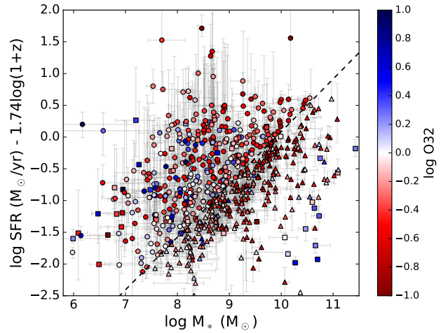
Fig. 5. SFR - M_* diagram where we have corrected the SFRs to z = 0 using the redshift evolution from Eq. 1. The dashed line shows this relation for z = 0 , above which we selected galaxies in our sample, as described in Sect. 2.6. The points are coloured by the logarithm of the dust-corrected O32 ratio. The symbols show galaxies in the final selection (circles), galaxies below the selection threshold (triangles), and galaxies with a lower limit on the O32 ratio (squares).
