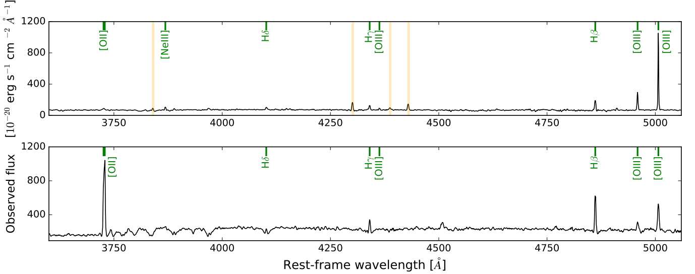
Fig. 1. Example spectra of O32 emitters in our sample. The upper panel shows the spectrum of the galaxy with the most extreme oxygen ratio (dust-corrected O32 = 23) from the UDF-mosaic catalogue with id = 6865 and z = 0.83 . The orange shaded lines show the H\gamma , H\beta , and [OIII]\lambda\lambda 4959, 5007 of neighbouring sources at z \approx 0.62 . An example spectrum of a galaxy with a lower O32 ratio, in this case with dust-corrected O32 = 0.25, is shown in the lower panel (UDF-mosaic, id = 892, z = 0.74 ).
