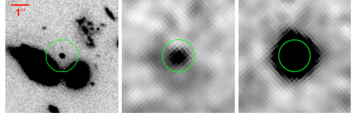
Fig. 19. HST F77W image (left), a MUSE narrow band image of the [O II]λ3727 line (middle), and a MUSE narrow band image of the [O III]λ5007 line (right) of the most extreme oxygen emitter with O32 = 23 .
