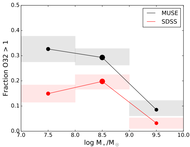
Fig. 11. Fraction of galaxies with O32 > 1 in bins of 1 dex with central \log M_*/M_\odot = 7.5, 8.5 , and 9.5 of our MUSE sample (black/grey) and the SDSS comparison sample (red) (see the text for details). The points denote the centres of the stellar mass bins and their size reflects the number of galaxies in the bin. The shaded areas cover the 1-\sigma errors as calculated by bootstrapping in the y-direction and the bin size in the x-direction.
