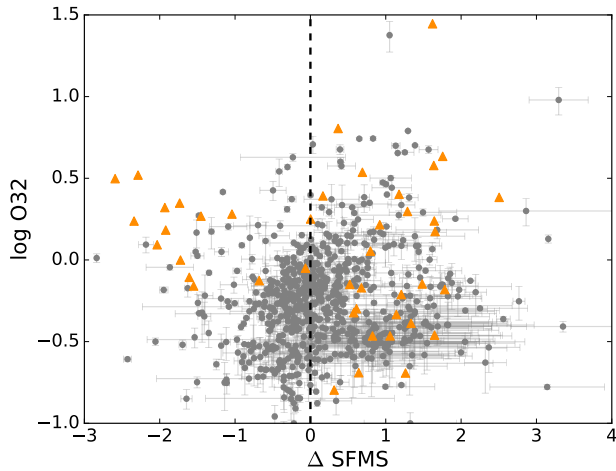
Fig. 6. O32 ratio versus the distance to the SFMS. Only galaxies above \Delta \text{SFMS} = 0 (dashed line) are included in the final sample. Lower limits on O32 are shown by orange triangles.
