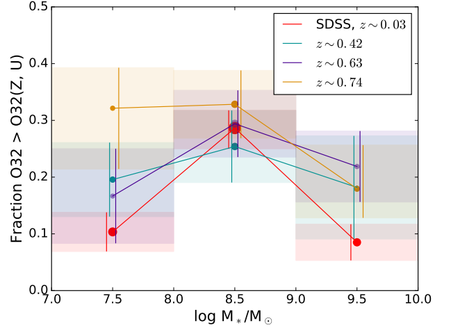
Fig. 14. Incidence rate of galaxies with O32 above the metallicity-dependent threshold for three equally sized redshift-selected subsets, with median redshifts of z = 0.42 (green), z = 0.63 (purple), and z = 0.74 (orange) and the entire SDSS comparison sample (red) with median redshift z = 0.03 . The vertical lines reflect the 1-\sigma errors in each bin.
