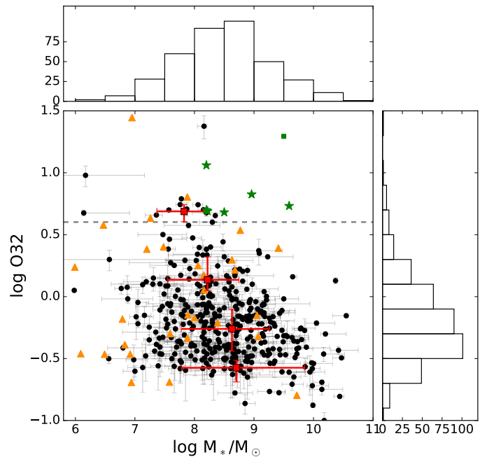
Fig. 7. Stellar mass as a function of \log \text{O32} (black dots) and lower limits on O32 (orange triangles). The median per bin with 1\text{-}\sigma errors is shown by the red squares and error bars. We defined the bins by intervals of \log \text{O32} between -1.0 and 1.0 with a step size of 0.5 . Three- \sigma lower limits on the O32 ratio for sources with a detection of [\text{O II}] below our S/N cut are shown by the orange triangles. The green stars indicate the positions of the confirmed Lyman continuum leakers from Izotov et al. (2016a,b, 2018a) and the green square is a LyC emitter at z=3.2 (de Barros et al. 2016; Vanzella et al. 2016). Galaxies above the grey dashed line have extreme O32 ratios ( \text{O32} > 4 ).
