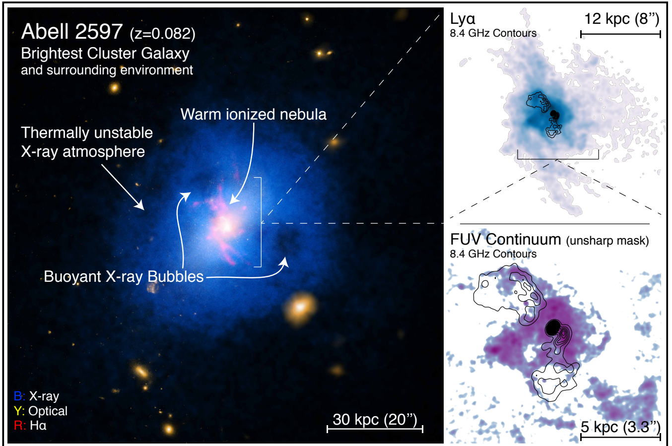
Figure 1. A multiwavelength view of the Abell 2597 Brightest Cluster Galaxy. ( Left ) Chandra X-ray, HST and DSS optical, and Magellan H\alpha+[N II] emission is shown in blue, yellow, and red, respectively (Credit: X-ray: NASA/CXC/Michigan State Univ/G.Voit et al; Optical: NASA/STScI & DSS; H\alpha : Carnegie Obs./Magellan/W.Baade Telescope/U.Maryland/M.McDonald). ( Top right ) HST /STIS MAMA image of Ly\alpha emission associated with the ionized gas nebula. Very Large Array (VLA) radio contours of the 8.4 GHz source are overlaid in black. ( Bottom right ) Unsharp mask of the HST /ACS SBC far-ultraviolet continuum image of the central regions of the nebula. 8.4 GHz contours are once again overlaid. In projection, sharp-edged rims of FUV continuum to the north and south wrap around the edges of the radio lobes. Dashed lines indicate relative fields of view between each panel. The centroids of all panels are aligned, with East left and North up. This figure has been partially adapted from Tremblay et al. 2016.
