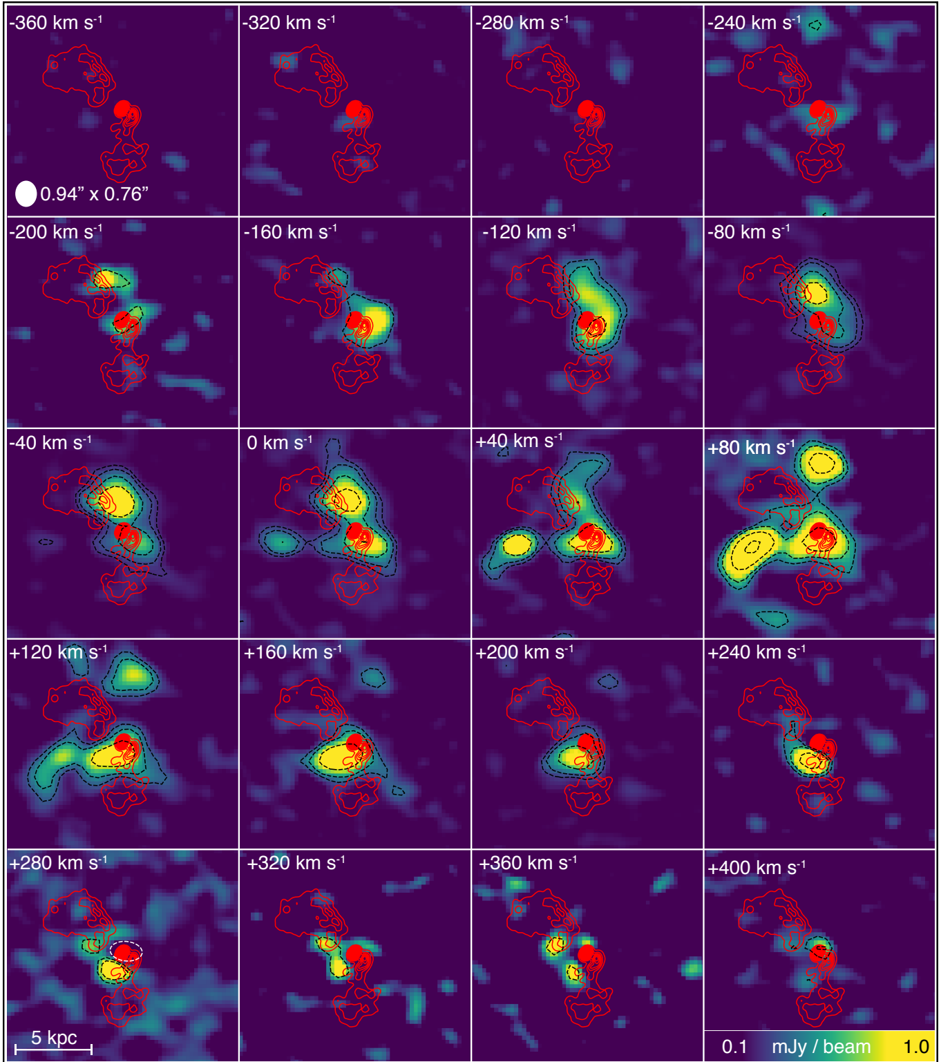
Figure 8. ALMA CO(2-1) channel maps, showing 40 km s -1 slices of the full data cube, ranging from -360 km s -1 through +400 km s -1 relative to the systemic velocity of the galaxy at z = 0.0821 . The outermost baselines have been tapered so as to increase signal to noise, resulting in beam size of 0.94'' \times 0.76'' , corresponding to a physical resolution of 1.4 kpc \times 1.2 kpc (marked by the white ellipse in the top left panel). Red contours show the 8.4 GHz radio source, and dashed black contours are used to mark significance of the emission. The outermost black dashed contours show where the CO(2-1) emission exceeds 3\sigma , and, when present, increase inward to show 5\sigma , 10\sigma , and 20\sigma over the background RMS noise of 0.18 mJy beam -1 per 40 km s -1 channel. The white dashed contour marks the continuum absorption discussed in subsection 3.1.
