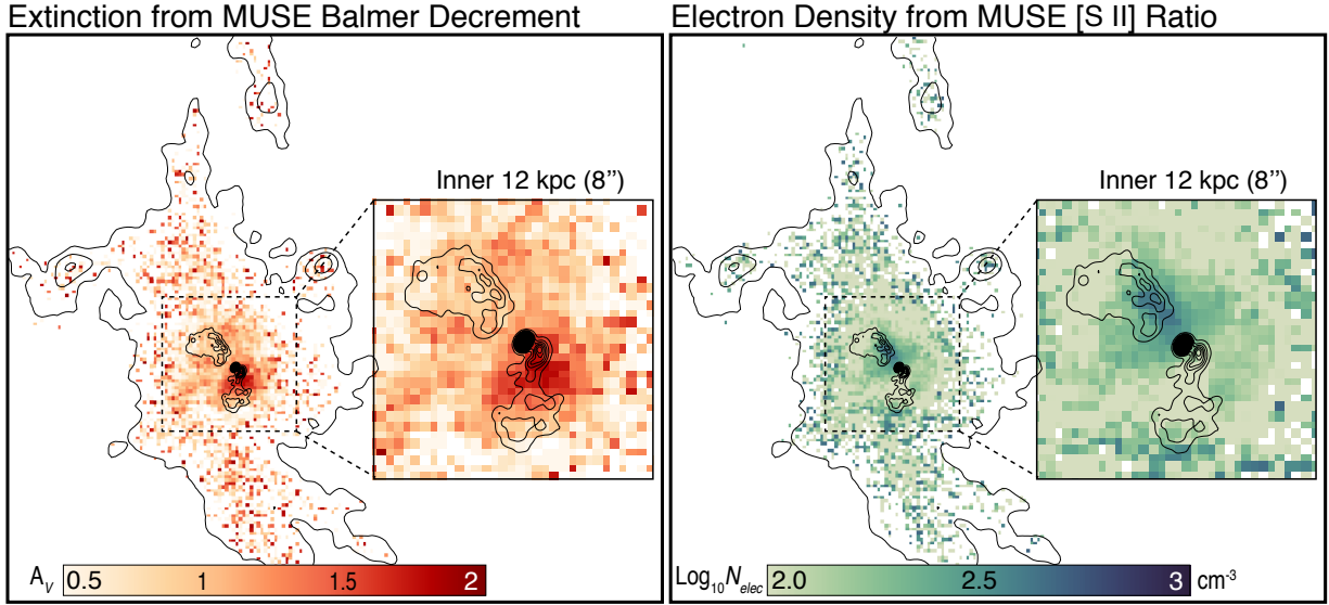
Figure 14. (left) An extinction ( A_V ) map made by scaling the MUSE Balmer decrement map ( H\alpha/H\beta ratio) following the procedure described at the end of subsection 2.2. The 8.4 GHz radio source is overlaid in black contours. The inset panel shows a zoom-in on this 12 \times 12 kpc 2 region. The color bar is in units of V -band magnitudes. (right) Electron density map, made by scaling the ratio of the forbidden Sulfur lines ( [S\ II]\lambda\lambda\ 6717\ \text{\AA} / 6732\ \text{\AA} ) using the calibration of Proxauf et al. (2014) and assuming an electron temperature of T_e = 10^4 K. The region of highest extinction is found just to the south of the nucleus, where the radio jet bends in position angle at the site of a bright radio knot with a large Faraday rotation measure, indicative of abrupt deflection. It is here that CO(2-1) is brightest (Fig. 6). The electron density map is highest at the boundaries of the southern radio lobe, and along the long axis of the northern radio lobe.
