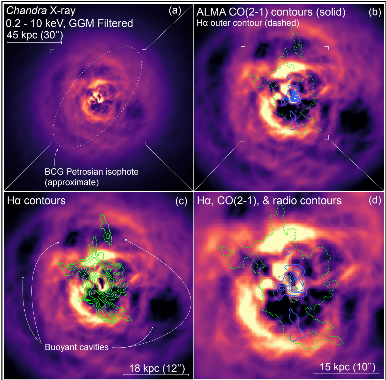
Figure 18. A new, deeper look at the X-ray cool core cospatial with the A2597 BCG. (a) 626 ksec Chandra X-ray observation of 0.2–10 keV emission in the innermost \sim 250 \times 250 \text{ kpc}^2 of the cluster. The X-ray data have been convolved with a Gaussian gradient magnitude (GGM) filter (e.g., Sanders et al. 2016a) to better show ripples and cavities. The optical Petrosian radius of the BCG’s stellar component is (roughly) marked by the gray dashed ellipse. Brackets indicate the relative fields of view shown in the surrounding panels. (b), (c), and (d) the same data, slightly zoomed in, with MUSE H \alpha , ALMA CO(2-1), and 8.4 GHz radio contours overlaid in green, blue, and gray, respectively. Moving inward, the ALMA contours in panel d show emission that is 3\sigma , 5\sigma , 10\sigma , and 20\sigma over the background RMS noise level. With the caveat that projection effects complicate interpretation, the H \alpha nebula shows strong circumstantial evidence that at least some of the filaments are draped around the edges of the buoyant X-ray cavities marked by arrows.
