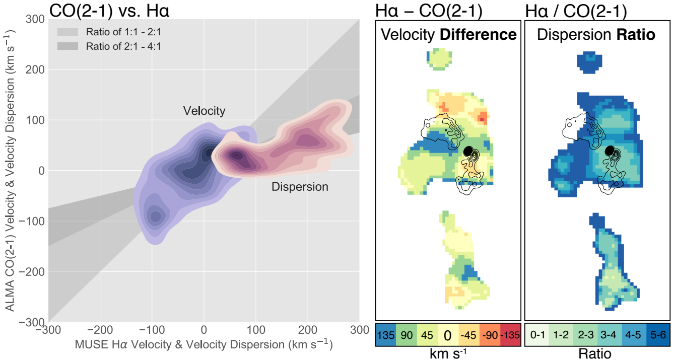
Figure 17. (Left panel) ALMA CO(2-1) vs. MUSE H \alpha velocity and velocity dispersion. Points are taken from every cospatial spaxel in the > 3\sigma overlap region between the warm ionized and cold molecular nebulae. The points have been smoothed with a Gaussian kernel. Contour colors encode the Gaussian kernel density estimate (i.e., a darker color indicates a higher density of data points). (Right panels) Maps of the difference and ratio between H \alpha and CO(2-1) velocity centroid and dispersion, made by subtracting and dividing the corresponding MUSE and ALMA moment maps, respectively. We have applied various corrections to account for, e.g., differing spatial resolutions, as described in subsection 2.3. The edges of these maps should be ignored. In the dispersion ratio map, for example, the outermost dark blue rim is smaller than the ALMA beam size, and an artifact of the division.
