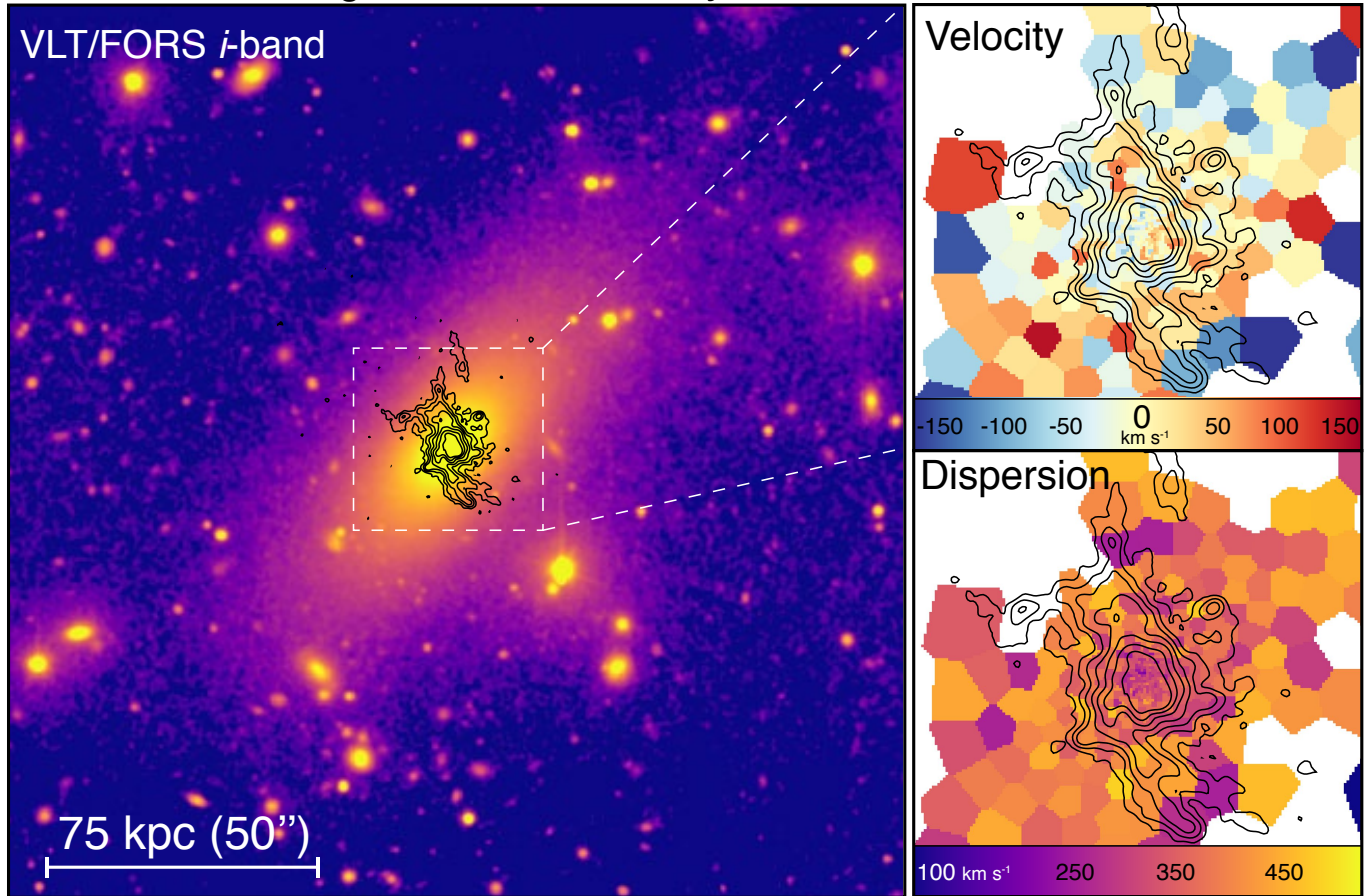
Figure 11. The host galaxy and the kinematics of its stellar component. ( Left ) VLT/FORS i -band image of the BCG and its surrounding 250 \text{ kpc} \times 250 \text{ kpc} environment. A logarithmic stretch has been applied to highlight the low surface brightness outskirts of the galaxy. H\alpha contours are shown in black, while the white dashed box indicates the FoV of the rightmost panels. ( Top right ) VLT/MUSE velocity map of the galaxy’s stellar component. The data have been Voronoi binned so increase S/N in the stellar continuum, as described in subsection 2.2. We only show the innermost 60 \times 60 \text{ kpc}^2 because the stellar surface brightness (and therefore S/N) drops rapidly beyond this FoV. Velocities have been projected around a zero-point at z = 0.0821 (e.g., cz = 24,613 \text{ km s}^{-1} ), as we have done for the ALMA and MUSE emission line velocity maps. ( Bottom right ) Best-fit stellar velocity dispersion (e.g. \text{FWHM}/2.35 ), also from the MUSE data. Dispersions are typical for a large giant elliptical galaxy (e.g., Faber & Jackson 1976).
