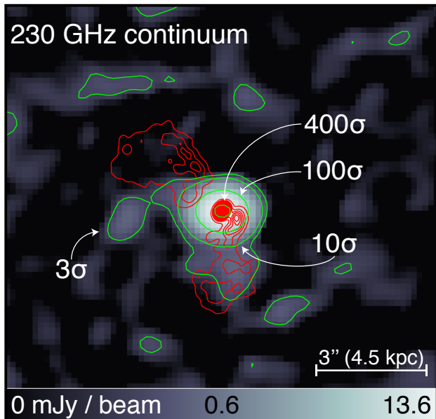
Figure 2. The ALMA 230 GHz continuum signal, summed over three basebands redward of the CO(2-1) line. The map is dominated by a mm synchrotron continuum point source associated with the AGN at the galaxy center, with a flux density of 13.6 \pm 0.2 mJy. Contours marking the 8.4 GHz VLA observation of the compact steep spectrum radio source are overlaid in red. The 10\sigma contour is consistent with an unresolved point source. A log stretch has been applied to the data so as to best show the 3\sigma extended emission against the \gtrsim 400\sigma point source. Much of this extended emission is likely to be noise, though the extension to the south along the 8.4 GHz radio source may be real. We are unlikely to have detected any extended dust continuum emission, given the FIR fluxes shown in Fig. 3.
