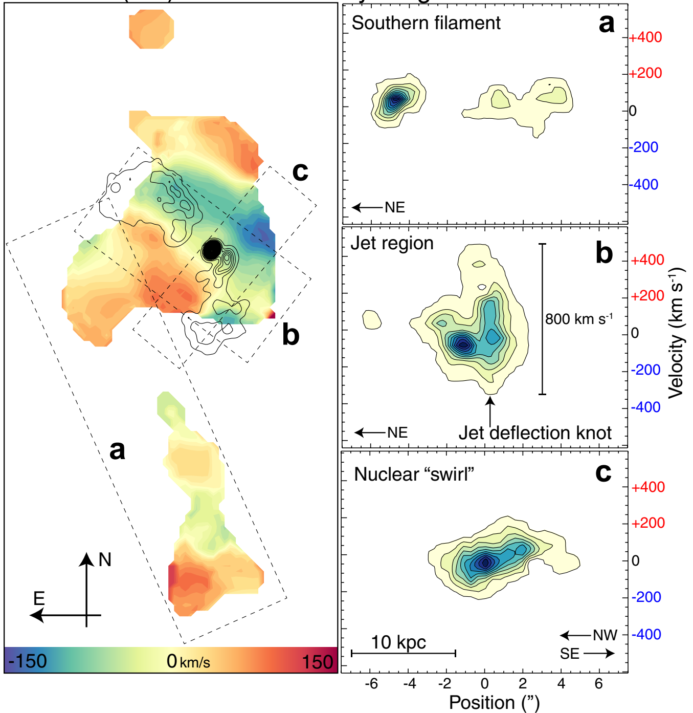
Figure 7. Position-velocity (PV) diagrams extracted from the three regions of the molecular nebula. The lefthand panel shows the Moment One velocity map from Fig. 6, with three position-velocity extraction apertures overlaid. The righthand panels show the PV diagrams extracted from these apertures. Arrows are used to show the cardinal orientation of each aperture’s long axis (the slit orientation for panel c is roughly perpendicular to that for panels a and b , and so the relative orientations are admittedly confusing at first glance). Note that while the length of the extraction aperture varied, all diagrams are shown on the spatial same scale in the righthand panels, enabling cross-comparison. Panel a shows that the southern filament has a narrow velocity width across its entire length, and no coherent velocity gradient. Panel b reveals the broadest velocity distribution of molecular gas in the entire nebula, and includes the region in which the 8.4 GHz radio source bends in position angle, likely because of deflection. Panel c shows rotation of molecular gas about the nucleus. All emission shown is \geq 3\sigma .
