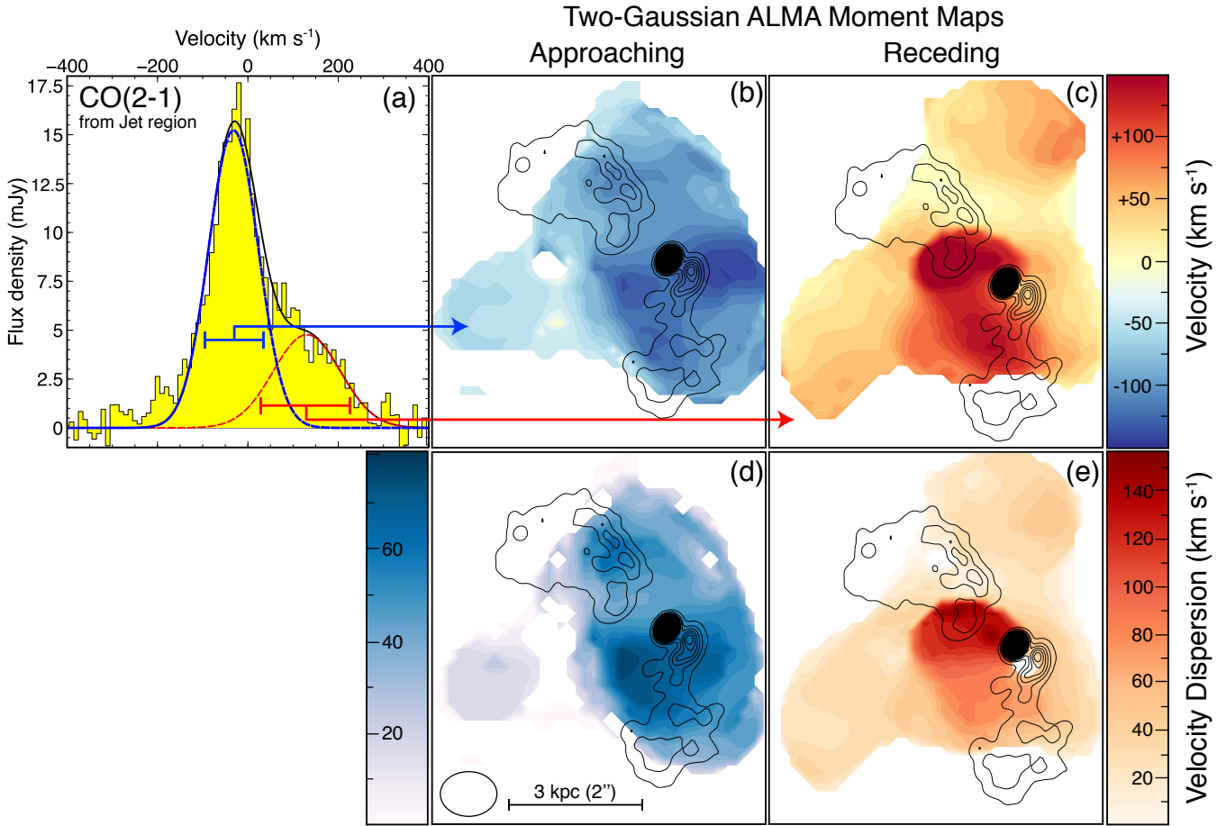
Figure 9. A closer look at the molecular gas cospatial with the radio jet. A single-Gaussian fit to this region (i.e., as shown for the moment maps in Fig. 6) does not adequately model the superposition of approaching and receding components along the same line of sight. Here we show moment maps created with a double-Gaussian fit, better representing the velocity distribution. (a) The CO(2-1) line profile extracted from a polygonal aperture encompassing the jet region, as shown in Fig. 5b. The line features a peak slightly blueward of center, as well as a strong red wing offset by \sim +150 km s -1 relative to the systemic velocity. Two Gaussians are fit to these components (shown in blue and red, respectively). Panels b and c show velocity maps for these approaching and receding molecular components, while panels d and e show their velocity dispersion maps. Multi-Gaussian fits for various sub-regions are explored in Fig. 10.
