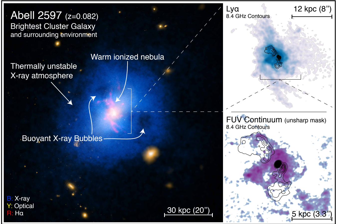
Figure 1. A multiwavelength view of the Abell 2597 Brightest Cluster Galaxy. (Left) Chandra X-ray, HST and DSS optical, and Magellan H\alpha+[N II] emission is shown in blue, yellow, and red, respectively (Credit: X-ray: NASA/CXC/Michigan State Univ/G.Voit et al; Optical: NASA/STScI & DSS; H\alpha : Carnegie Obs./Magellan/W.Baade Telescope/U.Maryland/M.McDonald). (Top right) HST /STIS MAMA image of Ly\alpha emission associated with the ionized gas nebula. Very Large Array (VLA) radio contours of the 8.4 GHz source are overlaid in black. (Bottom right) Unsharp mask of the HST /ACS SBC far-ultraviolet continuum image of the central regions of the nebula. 8.4 GHz contours are once again overlaid. In projection, sharp-edged rims of FUV continuum to the north and south wrap around the edges of the radio lobes. Dashed lines indicate relative fields of view between each panel. The centroids of all panels are aligned, with East left and North up. This figure has been partially adapted from Tremblay et al. 2016.
