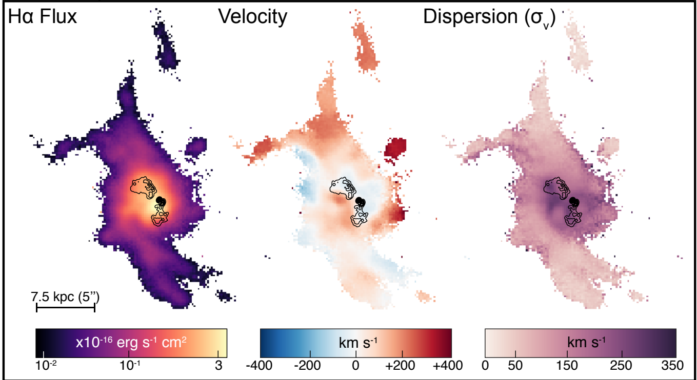
Figure 13. MUSE maps of H\alpha flux, line of sight velocity, and velocity dispersion in the warm ionized nebula, created after modeling and subtracting the stellar continuum as described in subsection 2.2. The H\alpha flux map (left panel) is shown with a logarithmic color scale to better show the faint filaments relative to the bright nucleus. Note the blueshifted “S”-shaped feature near the nucleus in the velocity map (center), strongly reminiscent of the shape of the 8.4 GHz radio source (shown in the flux map, for comparison). Note that these maps properly account for blending of the H\alpha and [N II] lines. Note also, particularly for the northern filaments, that velocities are higher at higher altitudes from the galaxy center, consistent more with uplift than gravitational freefall. Compare these maps to those for the cold molecular nebula in Fig. 6. We compare the MUSE and ALMA data directly in subsection 3.6.
