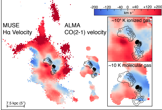
Figure 19. A side-by-side comparison of the MUSE H\alpha and ALMA CO(2-1) LOS velocity maps, shown on the same spatial and velocity scales. Insets show a zoom-in on the nuclear region for both maps. Black contours again show the 8.4 GHz radio source. Where they overlap, the MUSE and ALMA velocity maps look very similar to one another. These maps are more quantitatively compared in Fig. 17.
