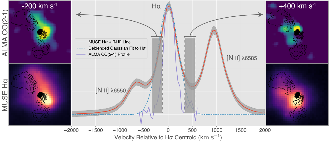
Figure 16. The MUSE H \alpha and ALMA CO(2-1) datacubes reveal similar morphologies at matching velocities, consistent with the hypothesis that the warm ionized and cold molecular gas are co-moving with one another, as would be predicted if the H \alpha emission arose from the warm ionized skins of mm-bright molecular cores. Here we show the MUSE H \alpha + [N II] profile extracted from a circular aperture with a diameter of 30 spaxels ( \sim 6'' ), centered on the galaxy core. We have deblended the H \alpha line from the [N II] doublet, and plot the resulting single Gaussian fit to H \alpha with the blue dashed line. The ALMA CO(2-1) spectrum, extracted from a (roughly) matching aperture, is plotted in purple.
