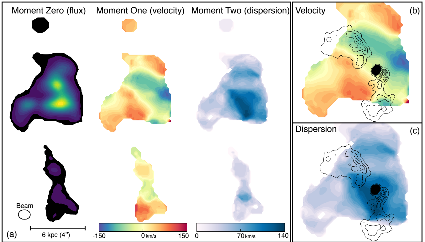
Figure 6. (a) Zeroth, First, and Second moment maps of integrated CO(2-1) intensity, mean velocity, and velocity dispersion (respectively) in the cold molecular nebula. The maps have been created from the ALMA cube using the “masked moment” technique to preserve spatial and spectral coherence of \geq 3\sigma structures in position-velocity space, as described in subsection 2.1. Panels (b) and (c) show a zoom-in on the nuclear region in the velocity and velocity dispersion maps, respectively. Take caution when interpreting these, because there are two velocity components (one approaching/blueshifted, the other receding/redshifted) superposed on one another. The velocity structure here is therefore best represented by a double-Gaussian fit, which we show in Fig. 9.
