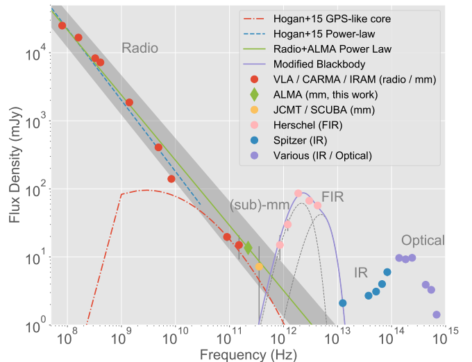
Figure 3. Radio-through-optical SED for Abell 2597, including the new ALMA mm continuum point. Dashed and solid lines show various fits to components of the spectrum including a one- and two-component fit to the radio and ALMA data (Hogan et al. 2015a,b), as well as a modified blackbody fit to the far-infrared Herschel data (Mittal et al. 2011, 2012). Observation details (including dates) and references for all photometric points are given in Table 1. Error bars are shown on the plot, though in many cases remain invisible because they are smaller than the data point. The gray shaded region shows the error on the single powerlaw fit to both the radio and ALMA continuum data. These fits are discussed in subsection 3.1.
