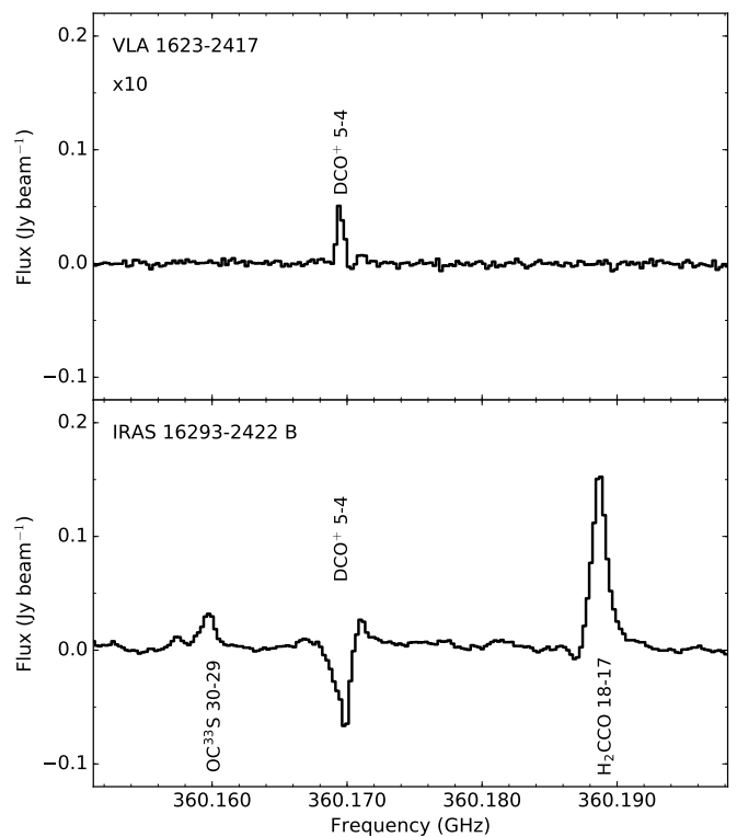
Fig. 7. Comparison of the spectra centered on \text{DCO}^+ 5–4 of VLA 1623-2417 A (12m array) and one beam offset from IRAS 16293-2422 B (combined 12m array and ACA). The spectra for VLA 1623-2417 has been multiplied by a factor of 10 in order to compare more easily. Note the lack of molecular line emission toward VLA 1623-2417 in contrast to IRAS 16293-2422.
