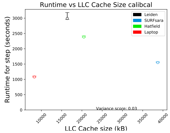
(a) calib_cal
