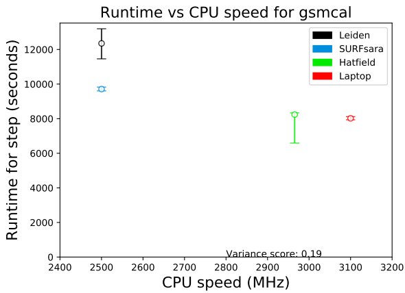
(b) gsmcal_solve
