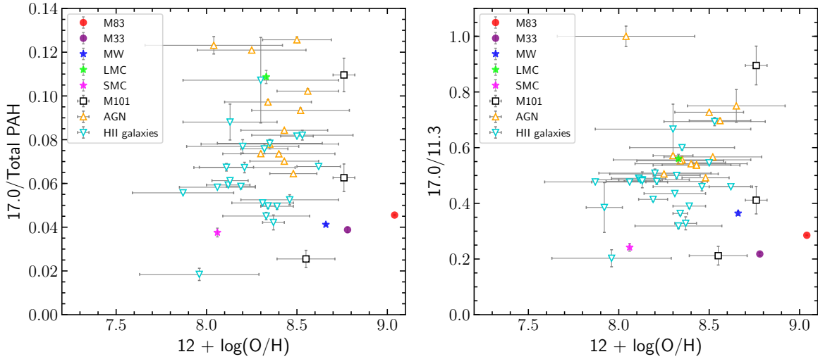
Figure 12. The ratio of the 17.0 \mu\text{m} complex with total PAH emission as a function of metallicity (left panel), and the 17.0/11.3 ratio as a function metallicity (right panel). For the M83, M33, MW, SMC, and LMC H II regions the average ratio fluxes are plotted using the metallicities from Table 3.
