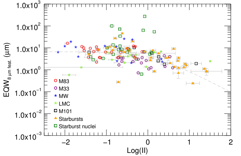
Figure 18. The equivalent width of the 8 \mu\text{m} complex vs. the ionization index (II). The dashed line shows the fit from Gordon et al. (2008) , fixed for normalization of the 8 \mu\text{m} feature (see text for details).
