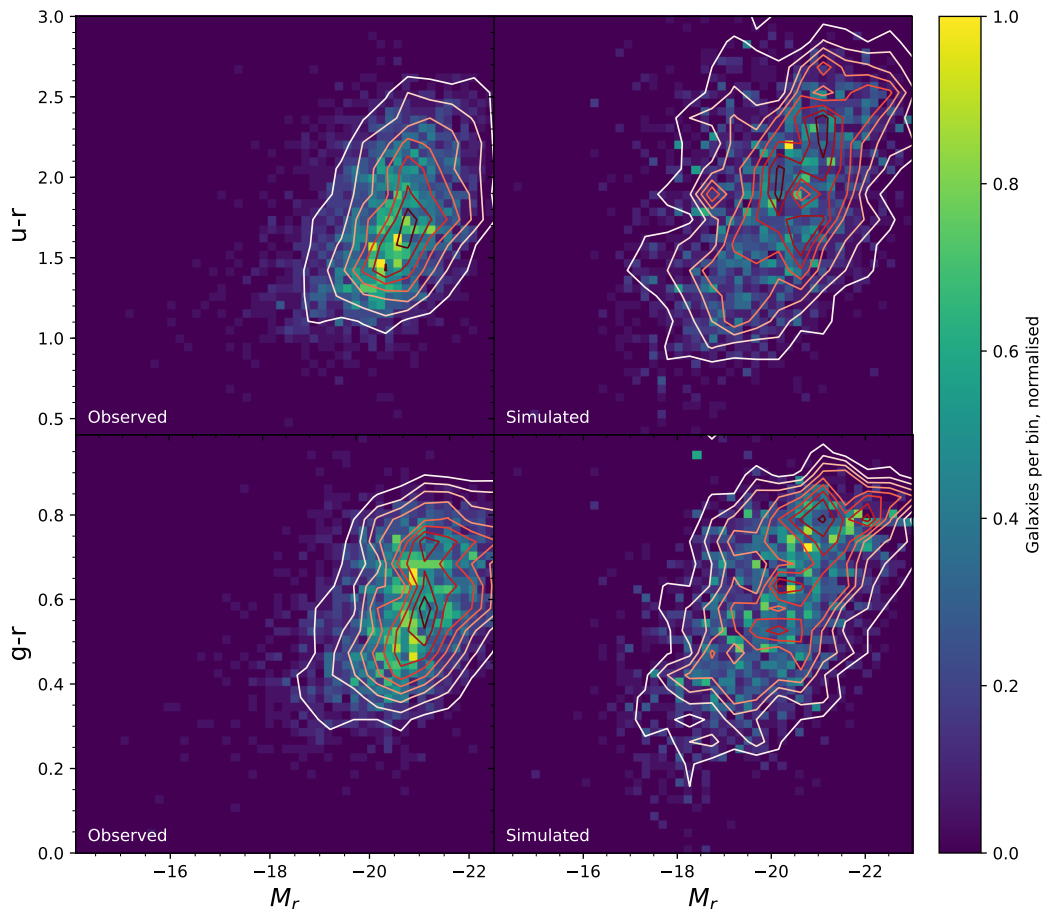
Figure 7. The distribution of galaxies in the colour versus r -band absolute magnitude diagram for the H-ATLAS sample, with the colour showing the density of galaxies in the diagram (see colour bar to the right). The left-hand panels show the observed distributions, which are the same as shown in the right-hand panels of Figure 2. The right-hand panels show the results of our simulation of where the H-ATLAS galaxies are expected to lie in this diagram if galaxies lie on a continuous, curved Galaxy Sequence (§4).
