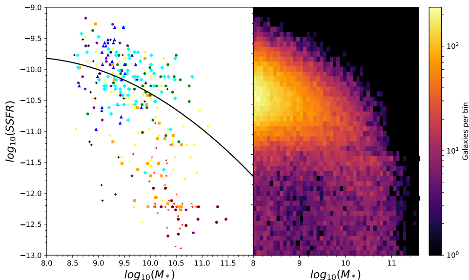
Figure 1. Left: Specific star-formation rate versus stellar mass for the galaxies in the Herschel Reference Survey (E17). The values of SSFR and stellar mass are estimates from the MAGPHYS SED-modelling program (Da Cunha et al. 2008). The colour and shape of each marker indicate the morphology of the galaxy: maroon circles - E and E/S0; red left-pointing triangles - S0; orange squares - S0a and Sa; yellow stars - Sab and Sb; green octagons - Sbc; cyan diamonds - Sc and Scd; blue triangles - Sd, Sdm; purple pentagons - I, I0, Sm and Im. The crosses show galaxies for which there is not a clear morphological class (Boselli et al. 2010). The line is a fit to the HRS galaxies with \log_{10}(\text{SSFR}) > -11.5 , which is the region of the diagram covered by late-type galaxies. The line is used in the Monte-Carlo simulation described in §4, and has the form \log_{10}(\text{SSFR}) = -10.39 - 0.479(\log_{10}(M_*) - 10.0) - 0.098(\log_{10}(M_*) - 10.0)^2 . Right: The artificial sample of 40,000 galaxies generated in the Monte-Carlo simulation described in §4, plotted in the same diagram as the HRS galaxies.
