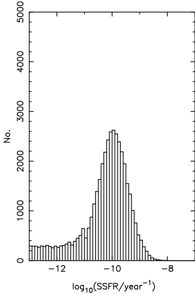
Figure 4. Histogram of specific star-formation rate for the 40,000 galaxies generated in the Monte-Carlo simulation described in §4.
