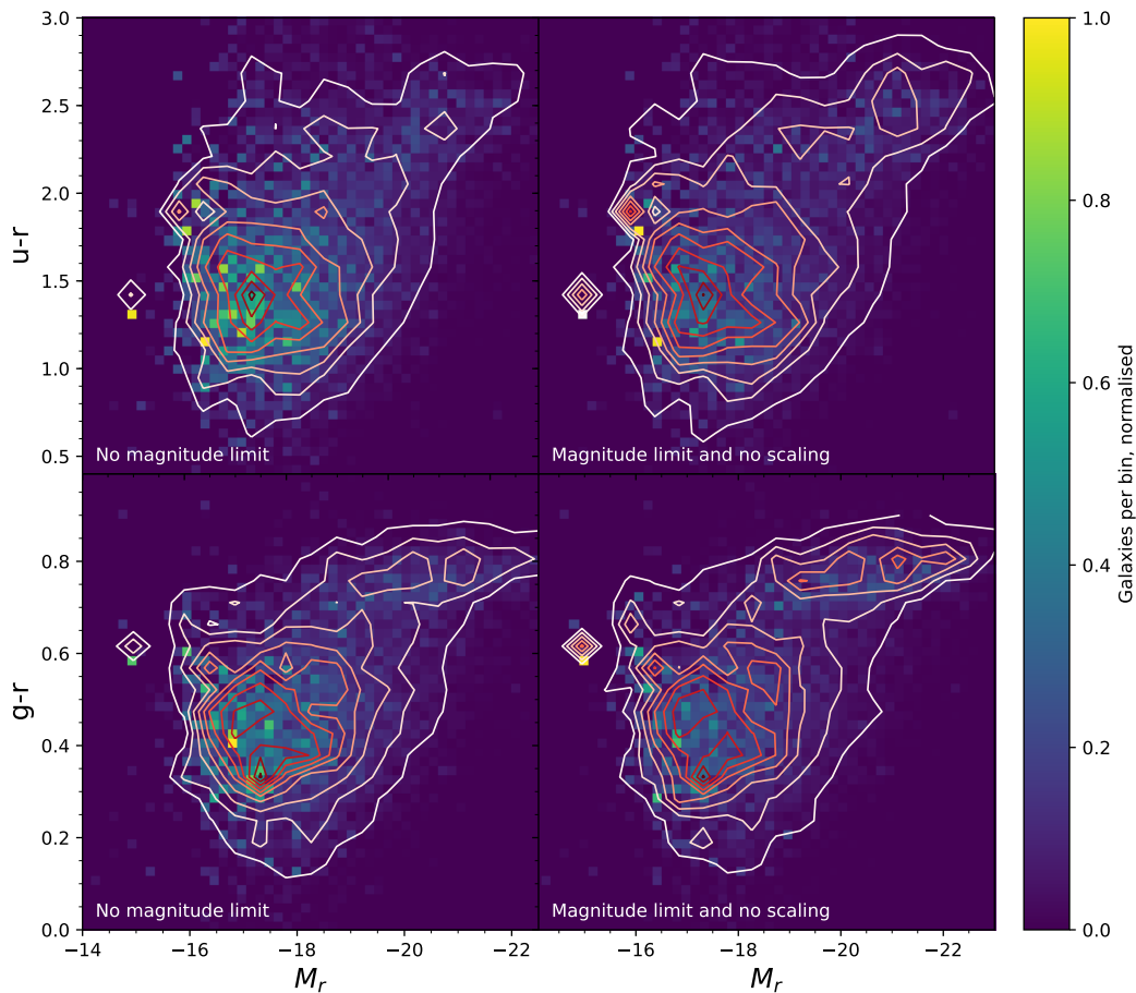
Figure 9. The distribution of galaxies in the colour-versus-absolute-magnitude diagram, with the colour showing the density of galaxies in this diagram (see colour scale to the right). The left-hand panels show the distribution for all 40,000 galaxies in our artificial sample (§4) when no flux limit is imposed on the sample. The right-hand panels show the result for an artificial sample with f_{pass} , the multiplicative factor for the stellar mass function of passive galaxies (§4), set to 1, for the artificial galaxies that satisfy the GAMA magnitude limit ( r < 19.8 ). To see the effect of changing the value of this parameter, these panels should be compared with the right-hand panels for Figure 6, for which f_{pass} = 0.5 .
