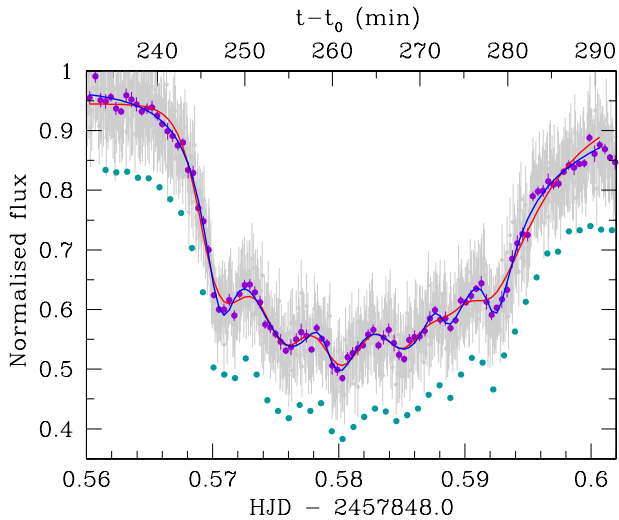
Figure 7. The LT light curve at the original 5-s cadence (gray) and binned by a factor seven (purple points) and zoomed in the B transit. The solid lines are the best fits with the function given by Eq. 1, where the ingress and egress time scales have been fixed to the values given by a fit to the A dip (red), or considered as free parameters (blue). The GTC white-light light curve (green points) has also been plotted with an offset -0.1 in order to emphasise the match between the short-term variability in the two independent data sets. The top x -axis ( t - t_0 ) is the time in minutes from the first data point of the unbinned LT light curve.
