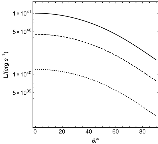
Figure 2. The luminosity of the decretion disc. The initial outer edge of the disc is at R_0 = 10^4 R_\odot . The times shown are t = 0 (solid line), t = 10^6 yr (dashed line) and t = 10^7 yr (dotted line).
