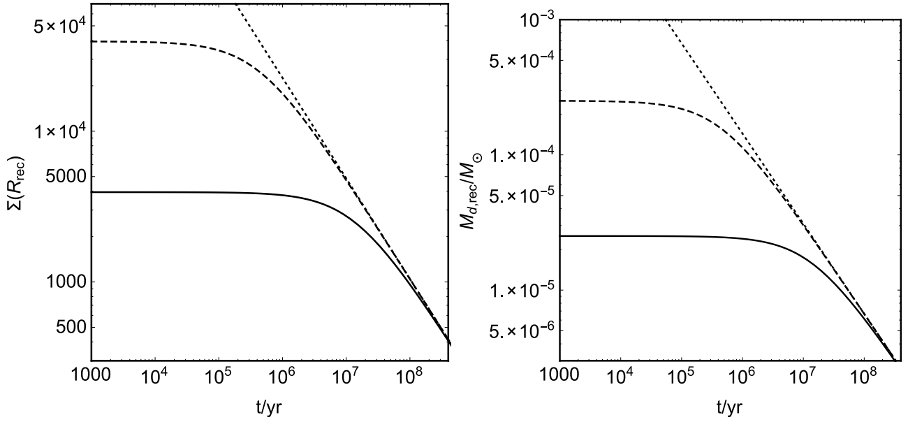
Figure 1. The decretion disc. Left: surface density at the recoil radius R_{\text{rec}} = 10 R_{\odot} as a function of time. Right: mass of the disc in R < R_{\text{ub}} . The initial outer edge of the disc is at R_0 = 10^5 R_{\odot} (solid line) and R_0 = 10^4 R_{\odot} (dashed line). The dotted lines show the analytic fits given in equations (28) and (29).
