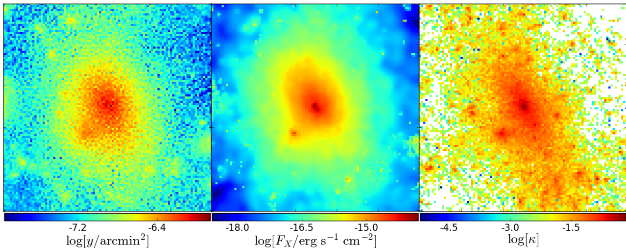
Figure 1. The three panels show 17' \times 17' cut-outs from the BAHAMAS light cone maps. From left to right we show the tSZ signal ( y ), the X-ray flux ( F_X ) and the lensing convergence ( \kappa ), centred on the most massive cluster, \log[M_{500}/(h^{-1}M_\odot)] = 14.27 . The X-ray map is in the 0.5–2.4 keV energy band and the \kappa map was generated using the KiDS source redshift distribution.
