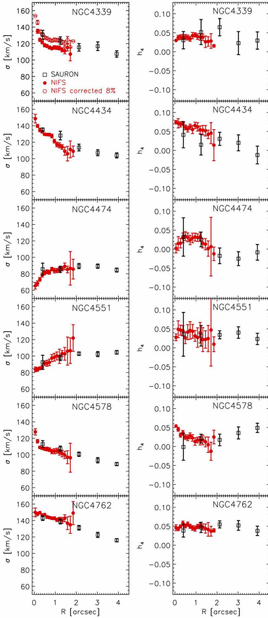
Figure 3. Comparison of radial profiles of the velocity dispersion (left column) and h_4 (right column) between the NIFS (red circles) and SAURON (open squares) data. The radial profiles were obtained by averaging using the bisquare weight of the values within concentric circular rings. The error bars show the half-width of the 95 per cent confidence interval around the sample mean. For NGC 4339 the NIFS velocity dispersion is lower by about 8 per cent, while for all other galaxies the agreement between the optical and near-infrared kinematics is remarkable.
