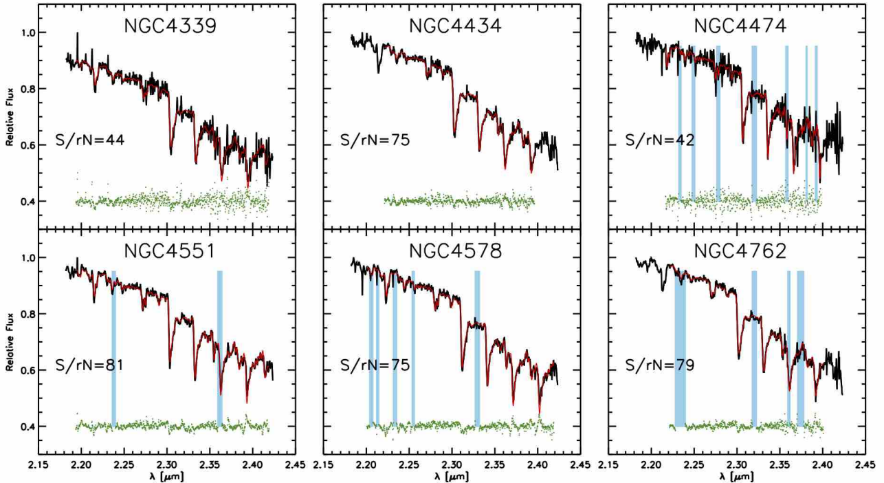
Figure 1. Example NIFS spectra of target galaxies obtained by summing the data cubes within a circular aperture of 1'' radius. Red line is the pPXF best fit model, while the green dots are the residuals between the data and the fit. Shaded light blue area indicate regions that were excluded from the fit. These fits are representative in terms of the wavelength range and the fit parameters of pPXF of fits for each Voronoi-binned spectrum providing the kinematics for each galaxy (Fig. 2). Signal-to-residual noise (S/rN) ratios for these spectra are given on each panel.
