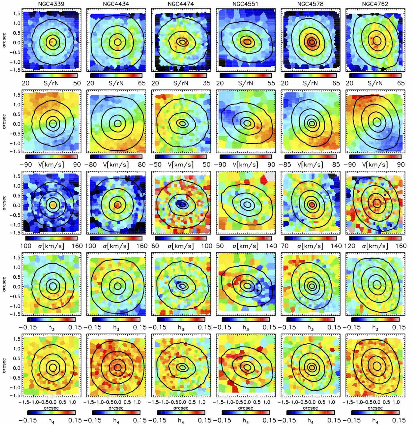
Figure 2. NIFS kinematics for sample galaxies (from left to right) NGC 4339, NGC 4434, NGC 4474, NGC 4551, NGC 4578 and NGC 4762. From top to bottom each panel shows maps of: signal-to-residual noise ratio (S/rN), the mean velocity (with the systemic velocity subtracted), the velocity dispersion, the Gauss-Hermite coefficients h_3 and h_4 . A median value of -0.054 was subtracted from the h_3 for NGC 4474. Colour-bars indicate the range of scales shown on maps. Black contours are isophotes, shown in steps of half a magnitude. North is up and East to the left.
