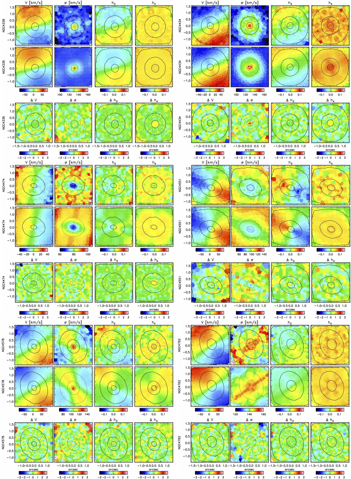
Figure E3. Comparison between the maps of symmetrised kinematics observed with NIFS and the best fitting Schwarzschild models. Each galaxy has three rows of maps showing the mean velocity, velocity dispersion, h_3 and h_4 Gauss-Hermite moments. Galaxies are (top left to bottom right): NGC 4339, NGC 4434, NGC 4474, NGC 4551, NGC 4578 and NGC 4762. Observations are in the first row, Schwarzschild models in the second row and the third row shows residuals (model-data for a given kinematic map) divided by the uncertainties. This means that colours trace the level at which the models differ to the data relative to the errors, and the extremes are set to 3 times the uncertainty. Black contours are light isophotes as observed and objects are oriented such that north is up and east to the left.
