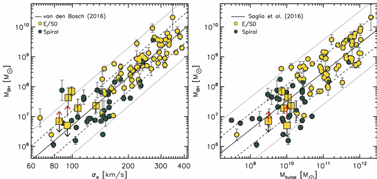
Figure 10. Left: Black hole mass - velocity dispersion relation based on the compilation of galaxies with dynamical M_{\text{BH}} measurements from Saglia et al. (2016), divided by their morphological classification as shown on the legend (based on column “Type” from that paper). The solid line is the best fitting relation from van den Bosch (2016), and the dashed and dotted lines show the one and two \sigma confidence zone. Galaxies from this study are shown with large squares or as upper limits (square with down pointing black arrows). The red upward pointing arrows indicate the lower limit on M_{\text{BH}} that could be expected to be measured at the resolution of our data assuming the sphere-of-influence argument. Note how our secure mass estimates are all above the relation and in two cases just outside of the 2\sigma confidence zone, making them amongst the largest outliers from the relation. Right: Black hole mass - bulge mass relation based on Saglia et al. (2016) compilation. The solid line is the best fitting relation from that work, while the dashed and dotted lines show the one and two \sigma confidence zone. Galaxies are divided by their morphology as shown on legend. In this case, our galaxies (filled squares) are within one \sigma confidence zone and consistent with the relation, while the upper limits are below the relation. The likelihood that the galaxies with the upper limit mass estimates do not harbour black holes is discussed in Section 5.4.
