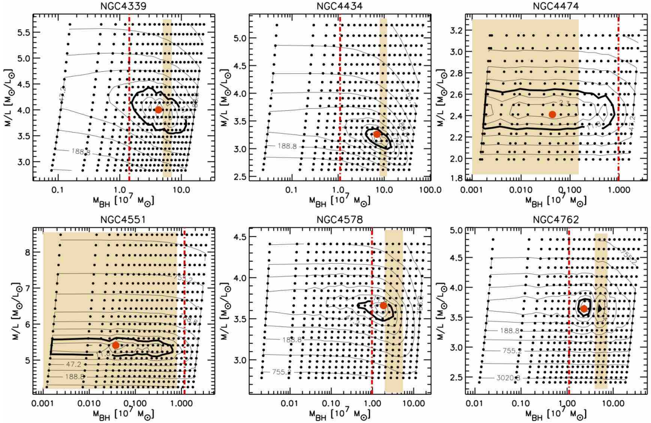
Figure 8. Grids of Schwarzschild models (shown by small round symbols) with different mass-to-light ratios and black hole mass. The best fitting models are shown by a large (red) circles in the formal \Delta\chi^2 minimum, while shaded rectangles trace the black hole mass estimates of the JAM modelling. Note that we do not compare the M/L ratios as they are calculated within different regions (see Section 4.3 for details why black hole masses can be compared). Contours are the \Delta\chi^2 = \chi^2 - \chi^2_{min} levels and the thickest contours show the 3\sigma level for a two-dimensional distribution. The dash-dotted (red) vertical line indicates the mass of the black hole which has the radius of the sphere of influence 2.5 times smaller than the FWHM of the narrow component of the AO PSF (Table 3). This is a very approximate estimate of the lower mass limit to a black hole we expected to be able to detect.
