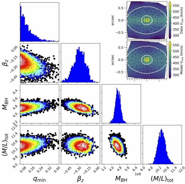
Figure A1. A set of plots showing the posterior probability distribution for the non-linear model parameters of JAM modelling ( q_{\min} , \beta_z , M/L_{\text{tot}} and M_{\text{BH}} ), marginalised over two dimensions (colour contours) and one dimension (blue histograms). The symbols are coloured according to their likelihood: white corresponds to the maximum value and dark blue to a 3\sigma confidence level. The inset in the upper right corner shows the data V_{\text{rms}} (bottom) and V_{\text{rms}} of the best fitting model (top).
