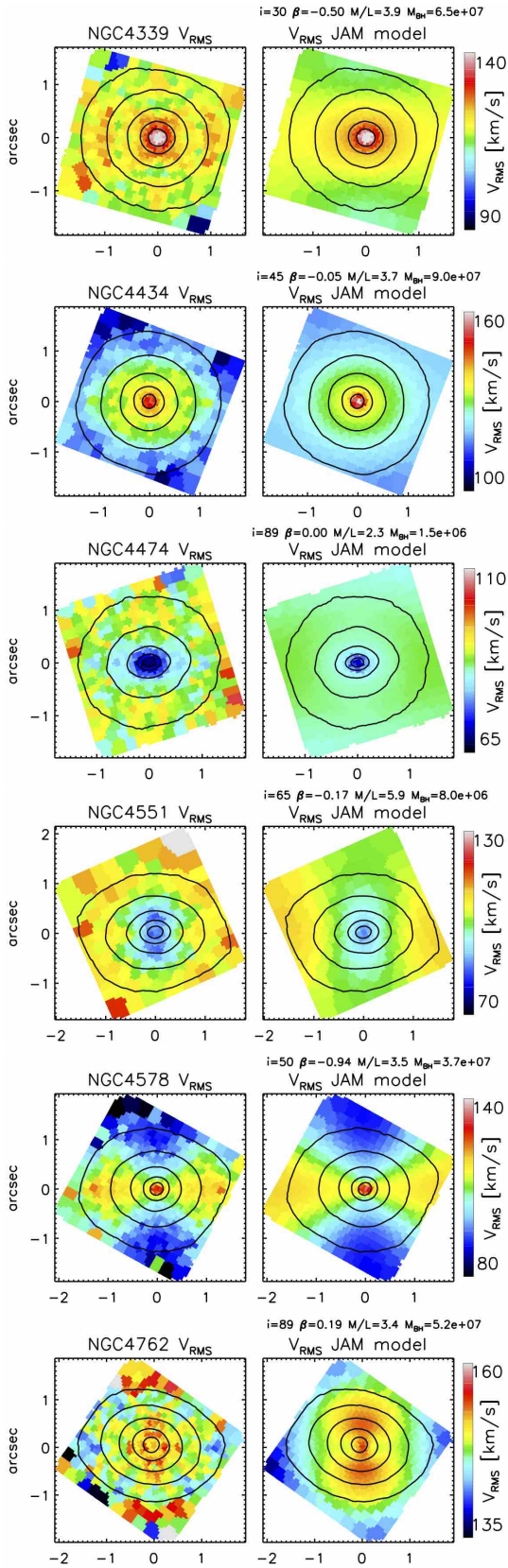
Figure 6. Comparison between the second velocity moment as parametrised by V_{\text{RMS}} from the NIFS data and the JAM models, for the best fit parameters (for NGC 4474 and NGC 4551 we use the upper limit for the black hole mass), which are shown on top of the model V_{\text{RMS}} maps. While the models were constrained using the original kinematics, V_{\text{RMS}} maps shown here are symmetrised as described in Section 4.4 for comparison purposes with bi-symmetric maps produced by the JAM models.
