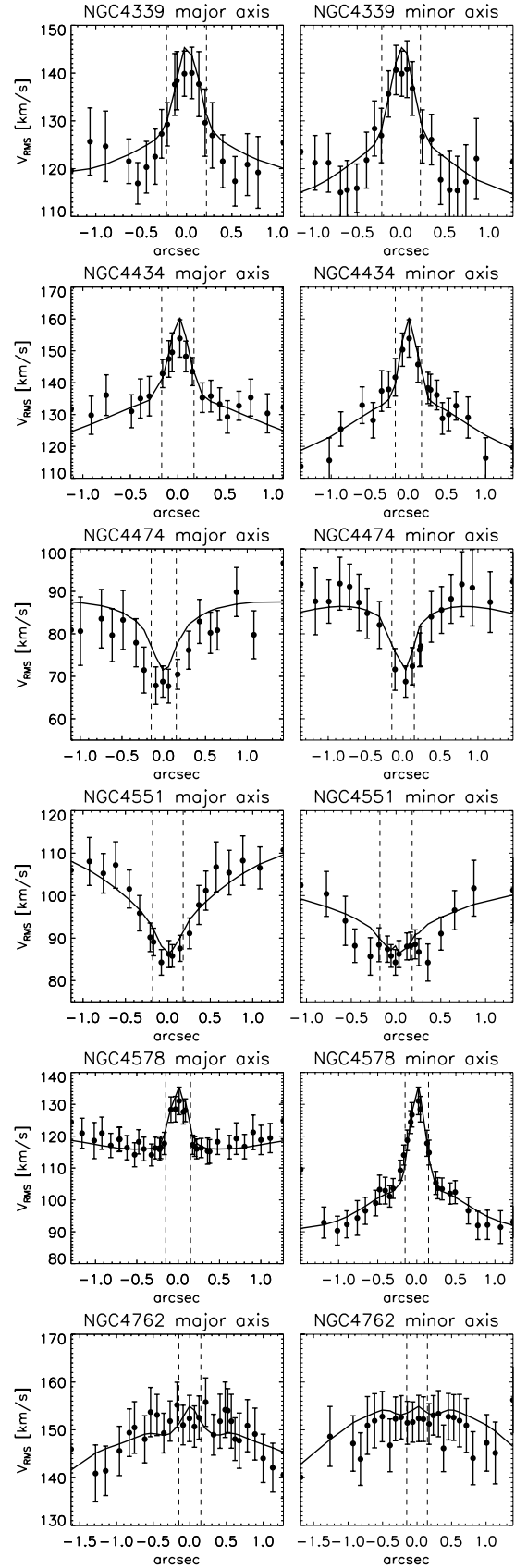
Figure 7. Comparison between the V_{\text{RMS}} extracted from the (symmetrised) V_{\text{RMS}} maps along the major and minor axes and the JAM models, having the same parameters as in Fig. 6.
