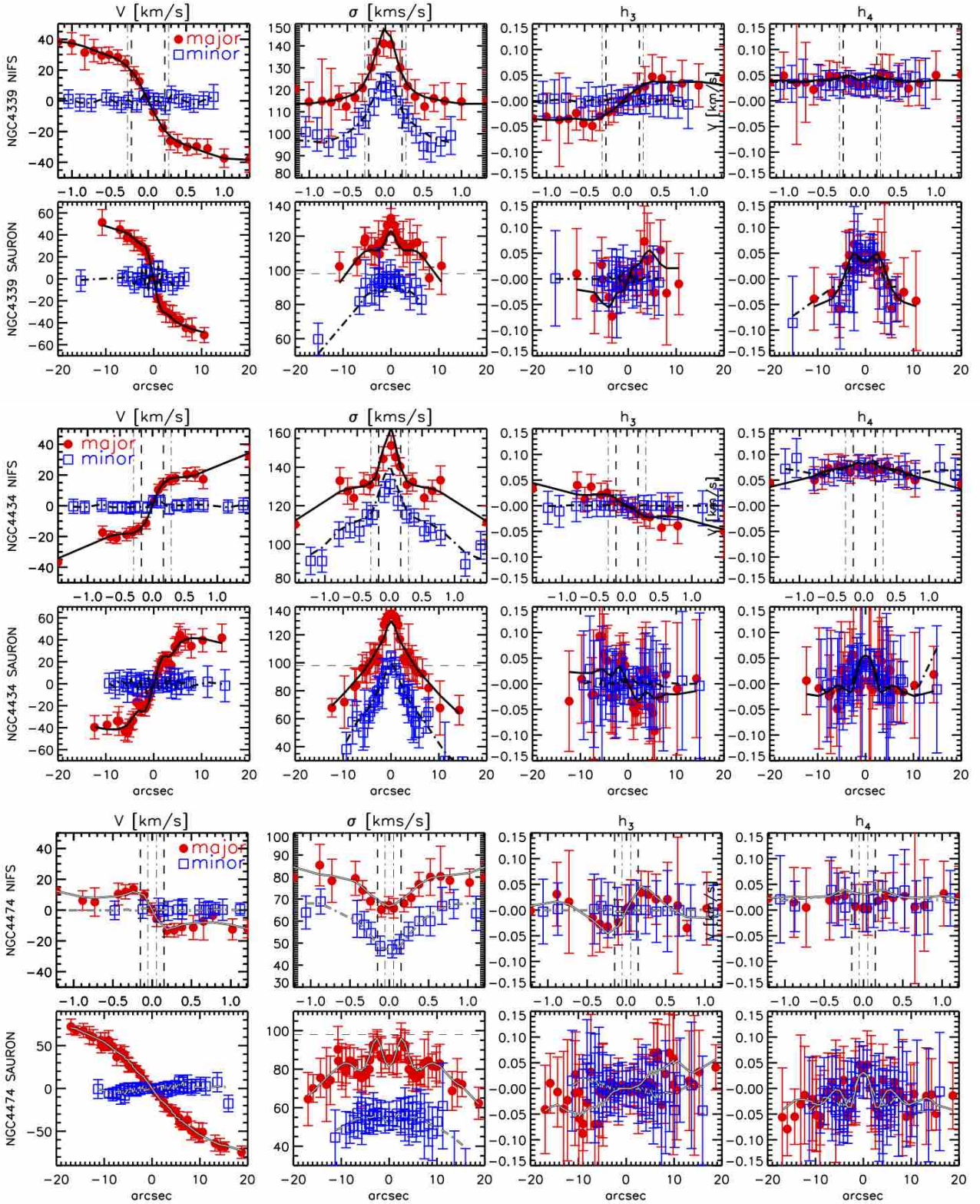
Figure E1. Comparison between the best fit Schwarzschild models and the symmetrised kinematics extracted along the major and minor axis for both NIFS and SAURON data of NGC 4339, NGC 4434 and NGC 4474 (for NGC 4474 we used both the formally best fitting model and the model providing the upper limit on M_{\text{BH}} ). Major axis data and models are shown with a solid line and red circles, while the a dash-dot line and blue open squares represent the positions along the minor axis. Upper limit models are shown with grey lines. The data were extracted along pseudo-slits of width 0.05'' and 0.8'' for NIFS and SAURON data respectively. Each galaxy is represented by two rows (top - NIFS, bottom - SAURON) of 4 panels showing the mean velocity, the velocity dispersion, h_3 and h_4 Gauss Hermite moments. The minor axis (both for NIFS and SAURON) velocity dispersion values are offset downwards for better visibility. Vertical dashed lines on the plots pertaining to NIFS data-model comparison indicate the FWHM of the PSF, while vertical dot-dashed lines indicate the estimated size of the SoI of the best fit model or the upper limit (in case of NGC 4474 and NGC 4551). Horizontal line on the velocity dispersion plot for SAURON data indicates the SAURON spectral resolution. NIFS spectral resolution ( \sim 30\text{km/s} ) is below the plotting range.
