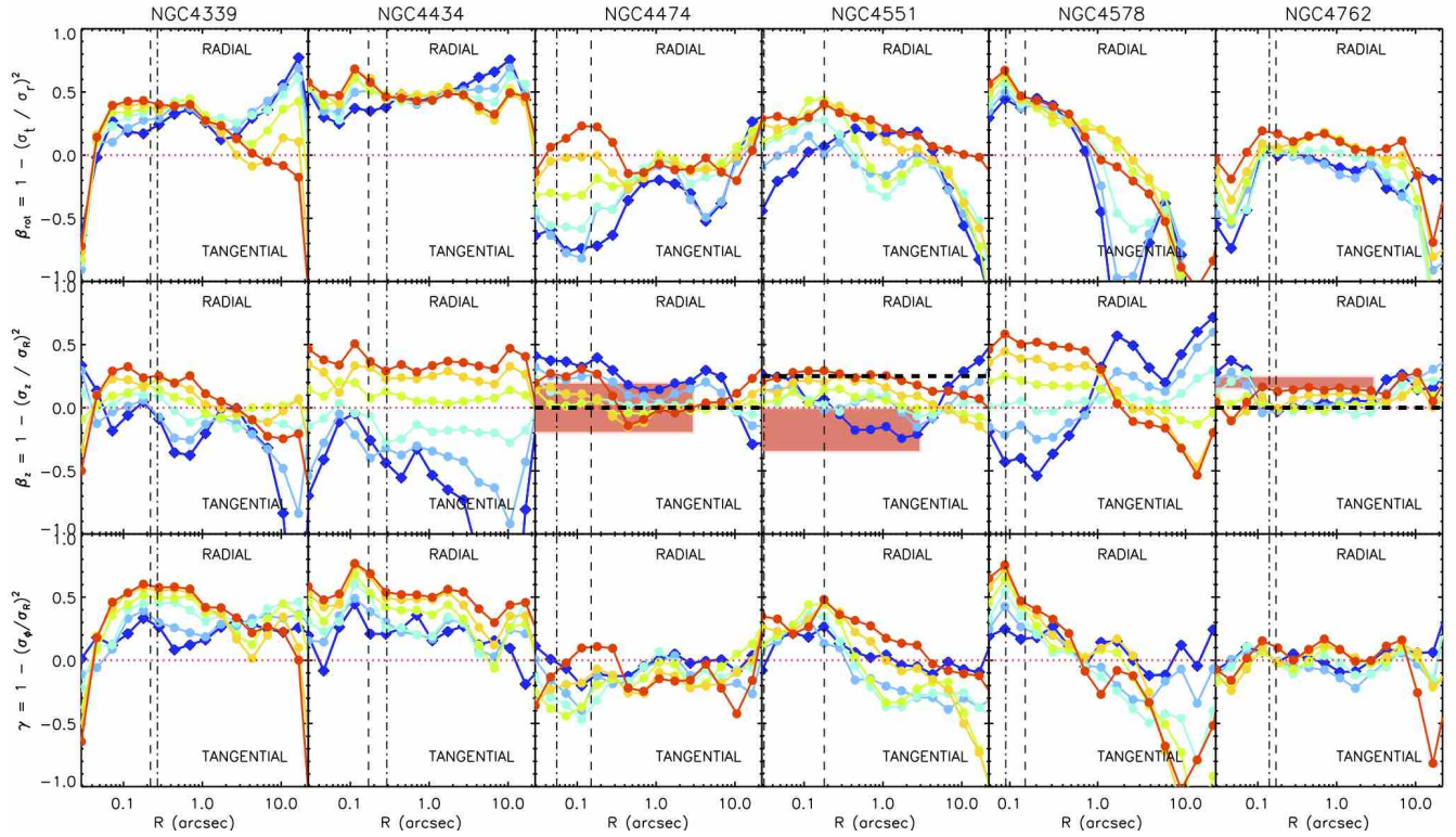
Figure 11. Radial profiles of the velocity anisotropy characterising the best fit Schwarzschild dynamical models. Each galaxy is in a column as indicated by names. Top: velocity anisotropy \beta_{rot} parameterised in the spherical coordinate system. Middle: velocity anisotropy \beta_z parameterised in the cylindrical coordinate system relating the radial and vertical axes (definition is equivalent as in JAM models). Bottom: velocity anisotropy \gamma parameterised in the cylindrical co-ordinate system relating the coordinates of the equatorial plane. In all cases the velocity anisotropy was measured at different polar angles defined in the meridional plane, spanning from 15^\circ (close to the equatorial plane, shown with the red line) to 75^\circ (close to the symmetry axis, shown with the blue line). The change in colours show the increase of the angle. Dashed vertical lines indicate the achieved resolution with the LGS AO (the FWHM of the narrow component of the PSF) and the dot-dashed vertical lines show the radii of the black hole SoIs using the best fitting M_{BH} (for NGC 4473 and NGC 4551 we use the upper limits) from Table 5. The shaded regions in the middle panels show the range of anisotropies estimated by JAM models for galaxies seen at inclination larger than 60^\circ . Thick dashed black line shows JAM \beta_z from Cappellari et al. (2013a) constrained by the SAURON data only.
